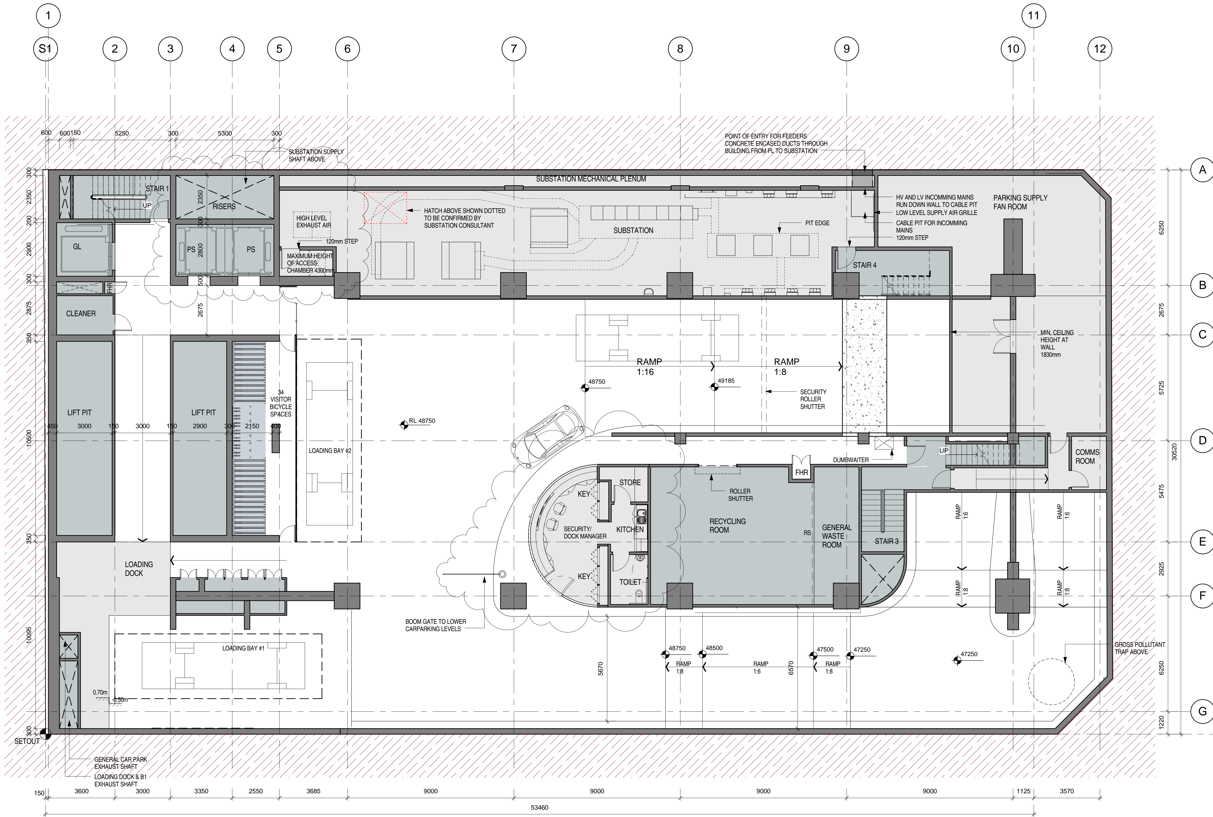
Level B1 Plan
