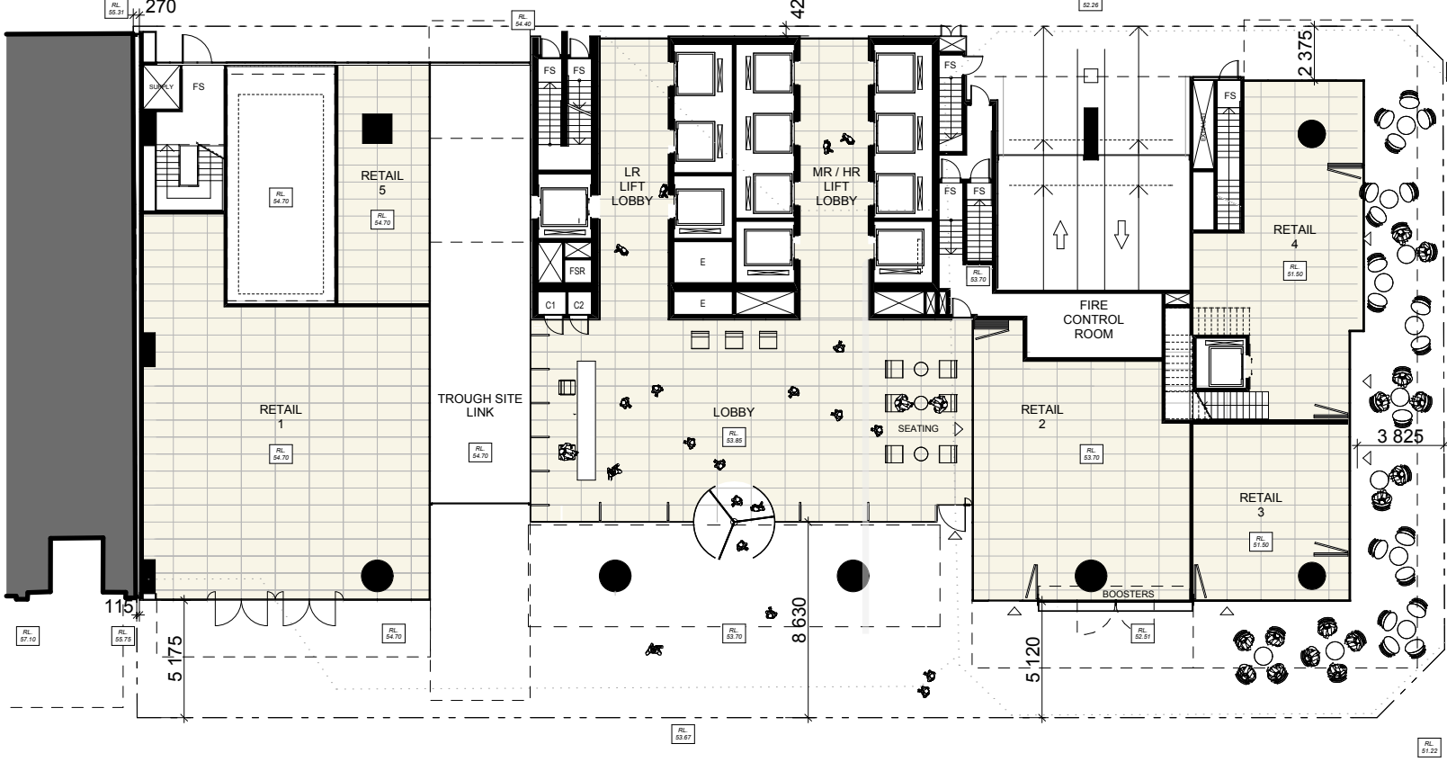
LEVEL 6 - GROUND
