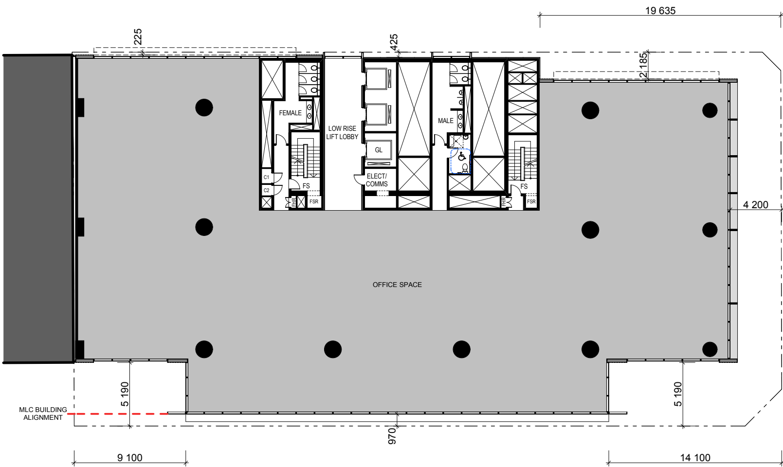
LEVELS 12 TO 19
