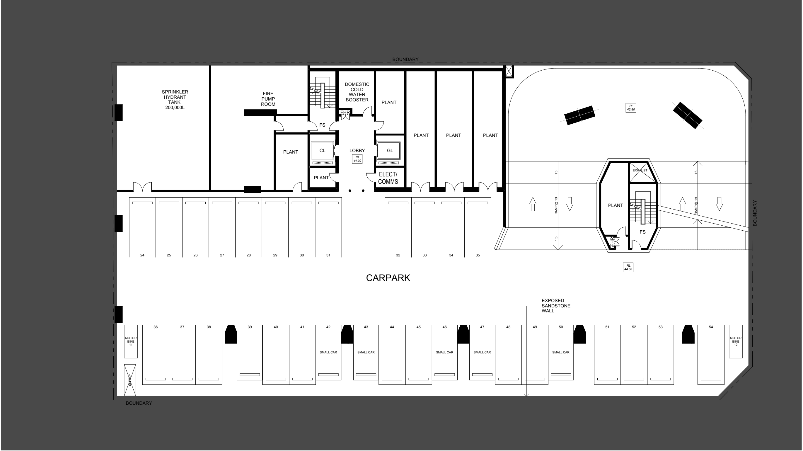
LEVEL 3 - BASEMENT 3
