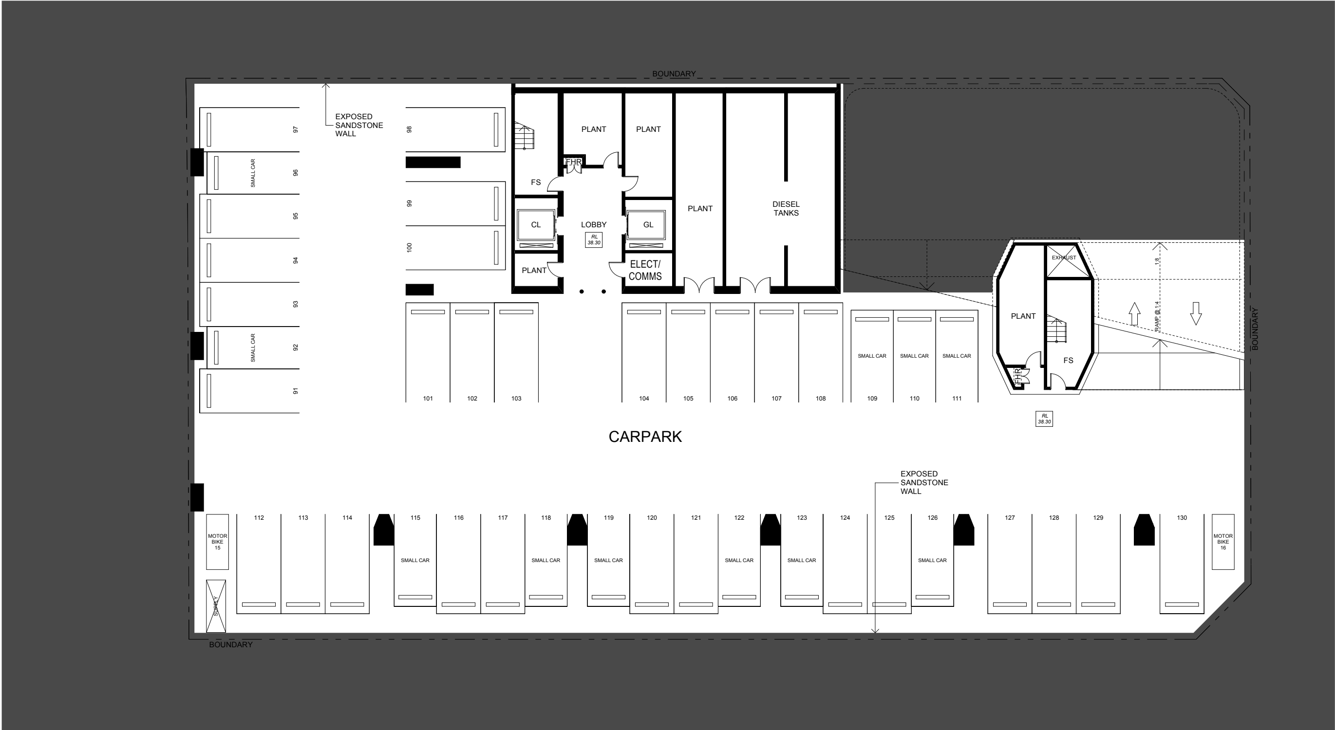
LEVEL 1 - BASEMENT 5
