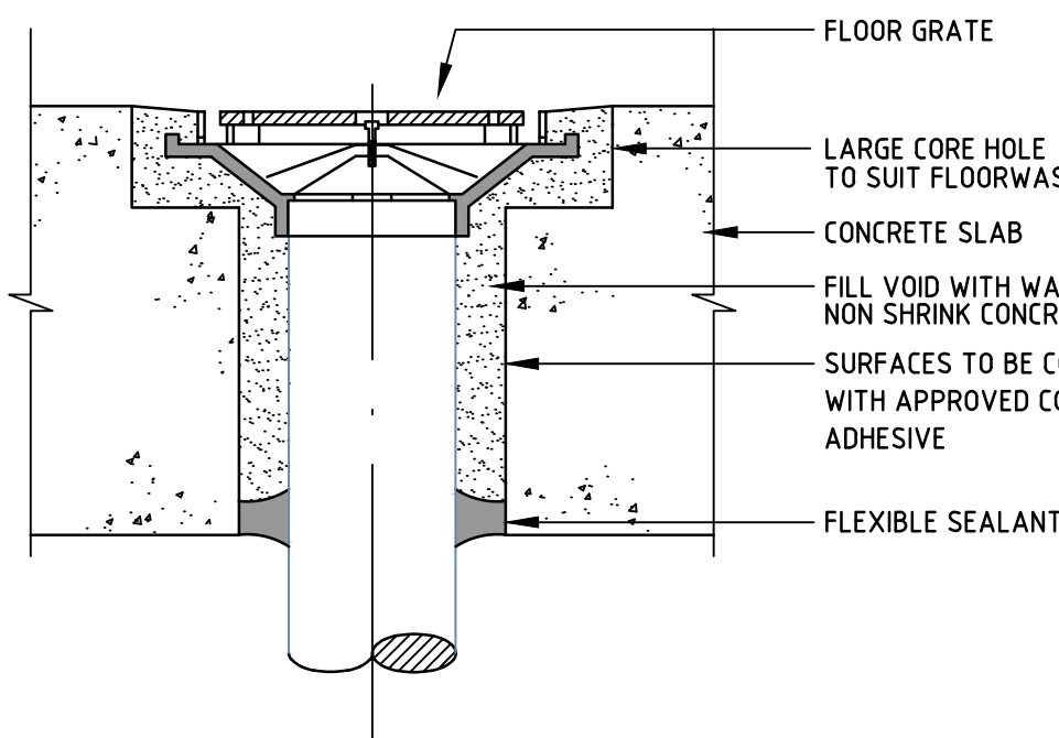
TYPICAL PENETRATION FOR PIPE SET INTO SLAB NOT TO SCALE
