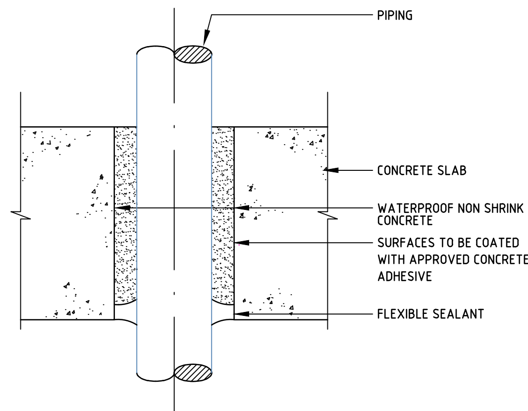
TYPICAL PENETRATION FOR PIPE RISER SET INTO SLAB NOT TO SCALE
