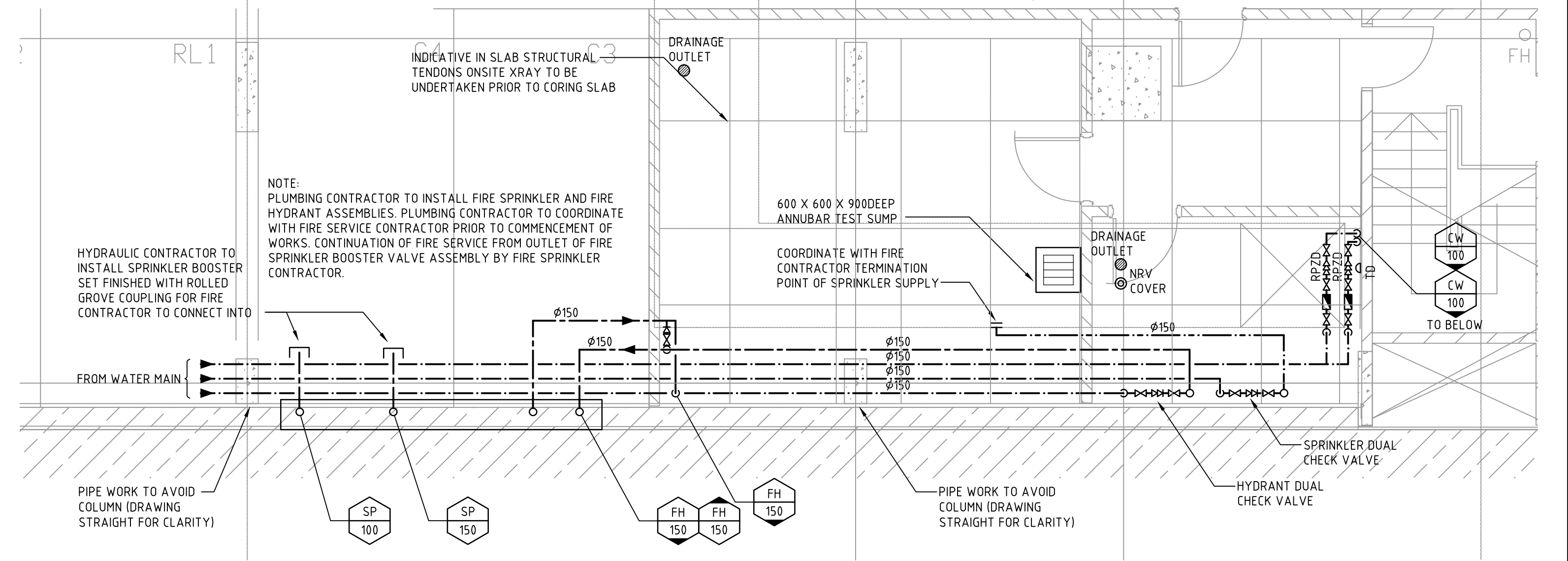
DETAIL 1 1:50 H-10101
