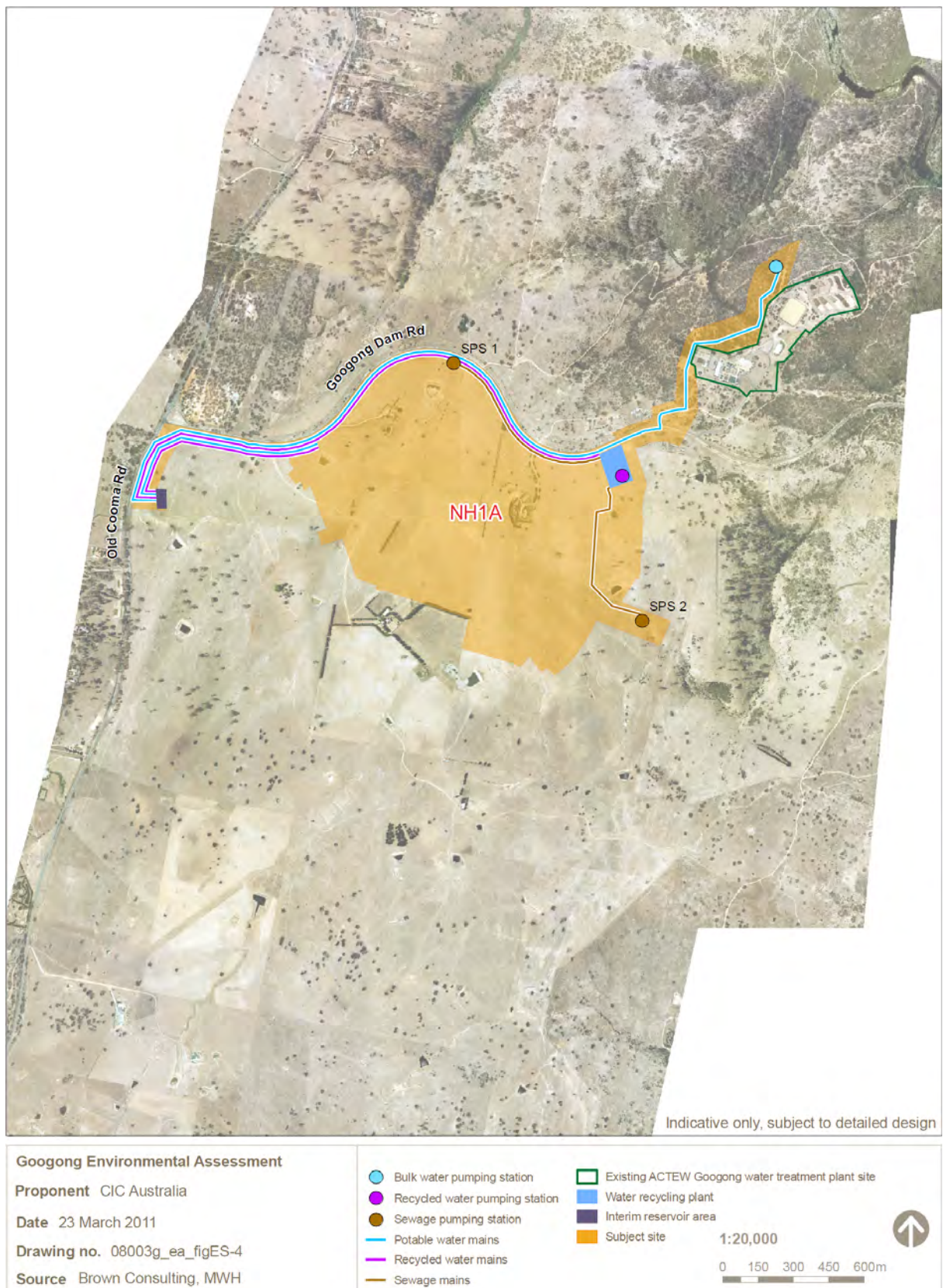
Figure 4: Stage 1 Project Layout
