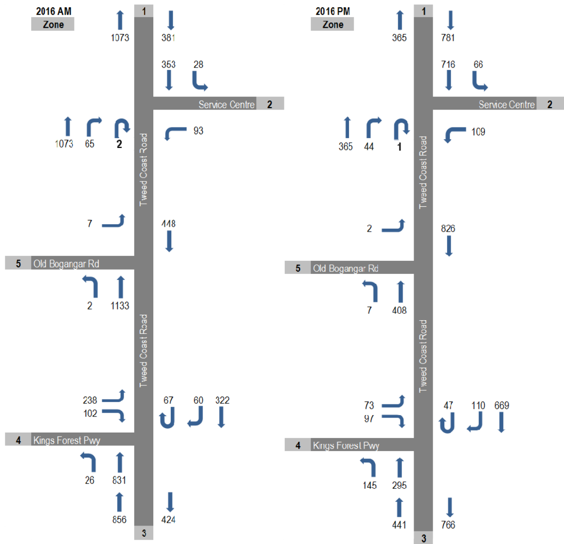
Figure 3.3: 2016 Aimsun Model Volumes
