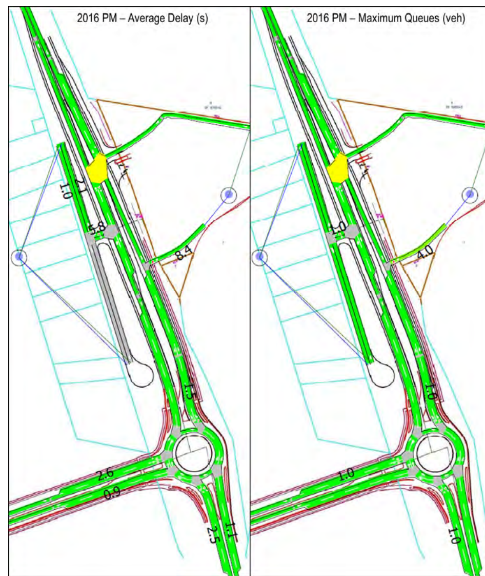
Figure 4.3: 2016 PM Model Outputs
