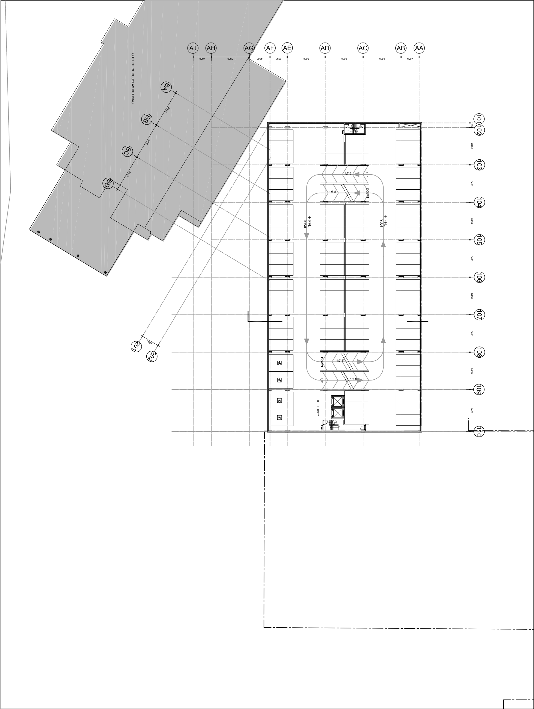
WESTERN CARPARK - LEVEL P6 (FFL 99.8)
