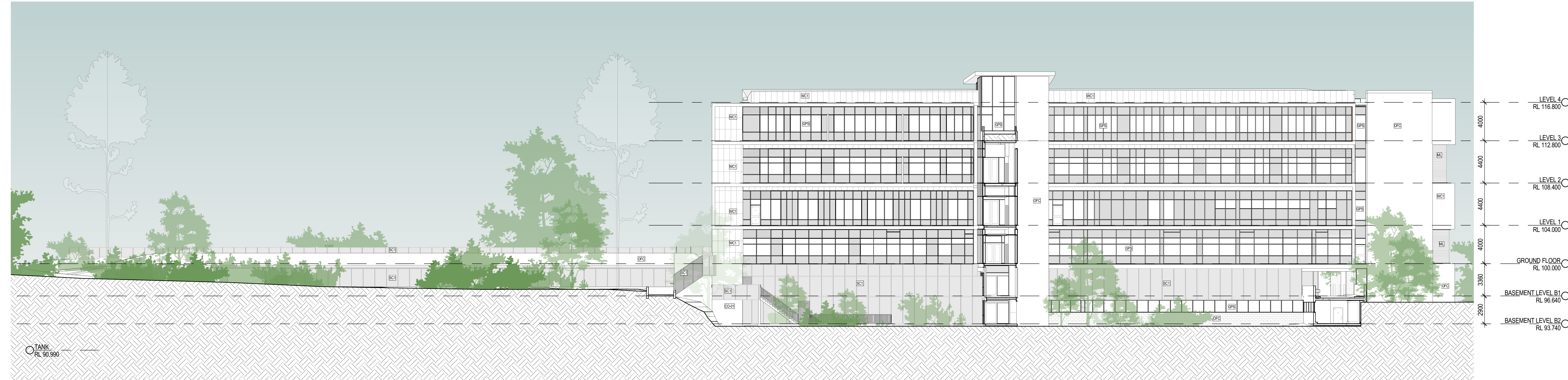
2 SOUTH SECTION THROUGH COURTYARD - EXTENSION 1: 200
