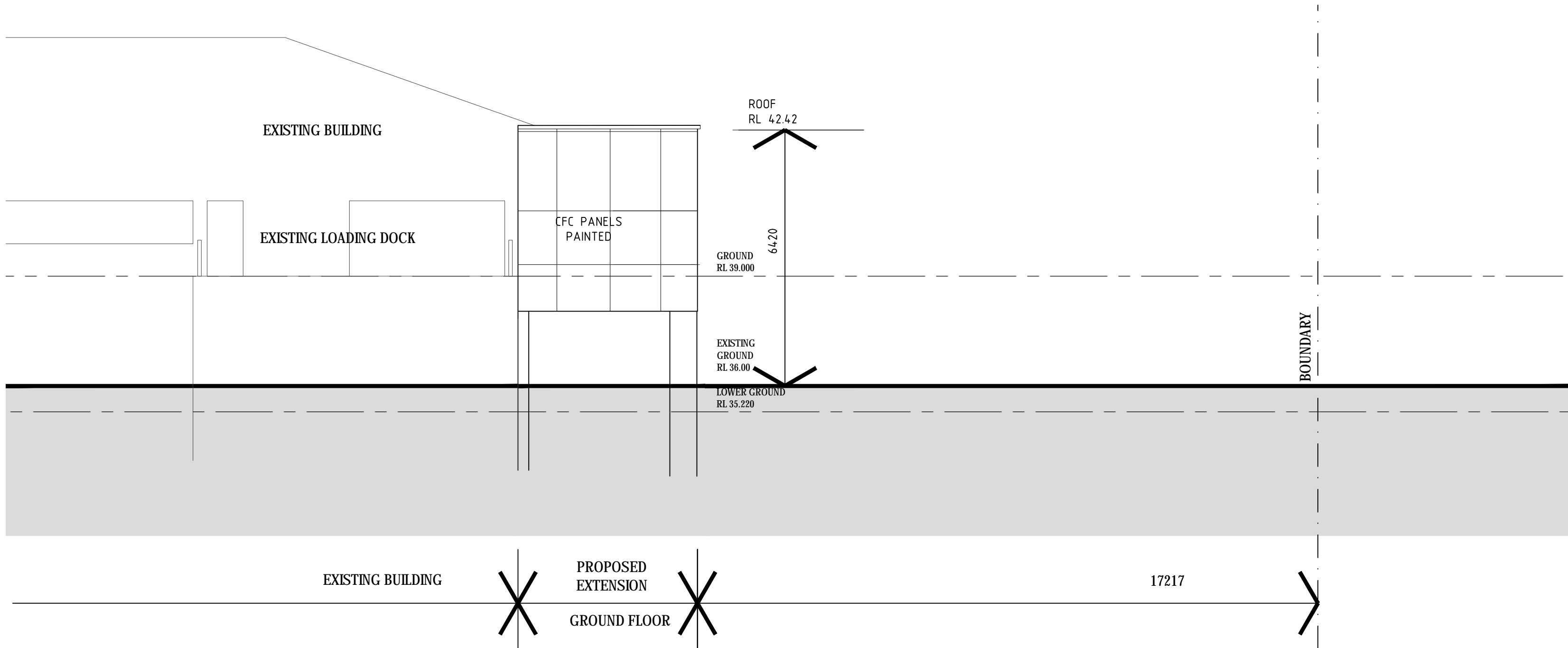
ELEVATION - SOUTH
