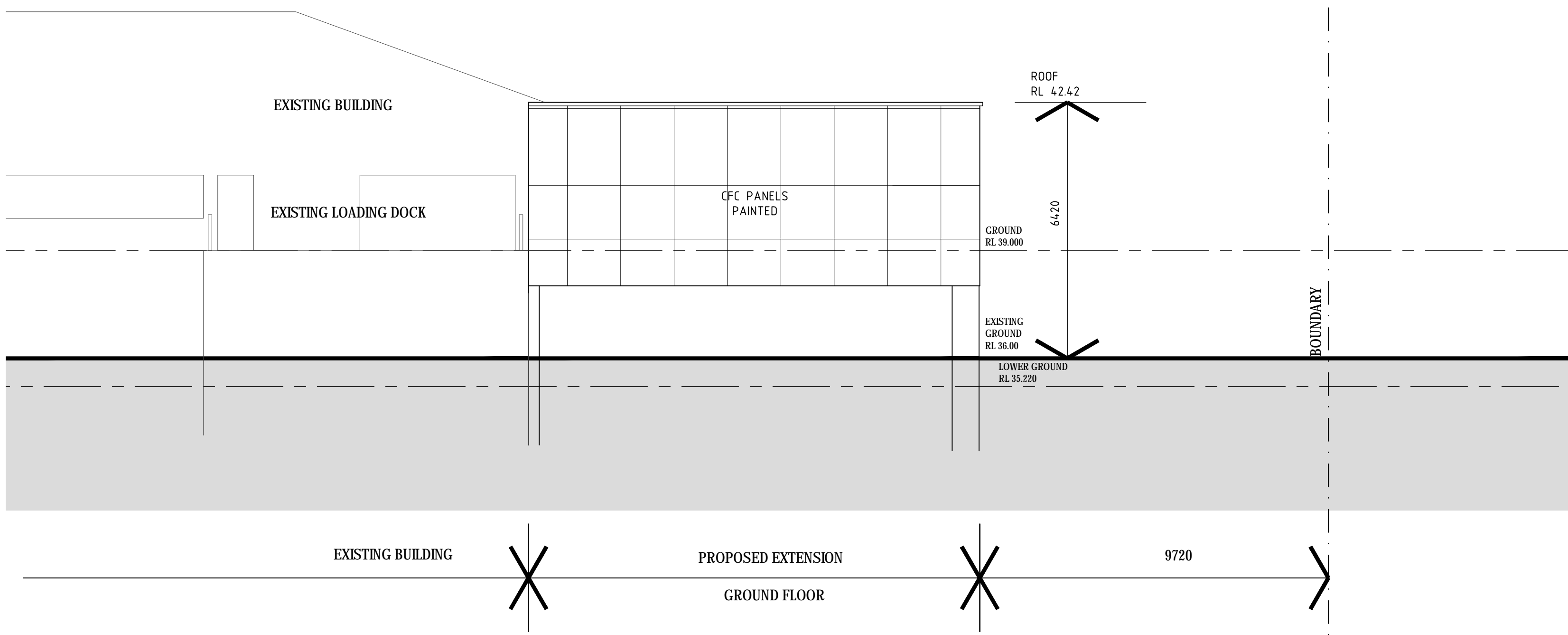
ELEVATION - SOUTH
