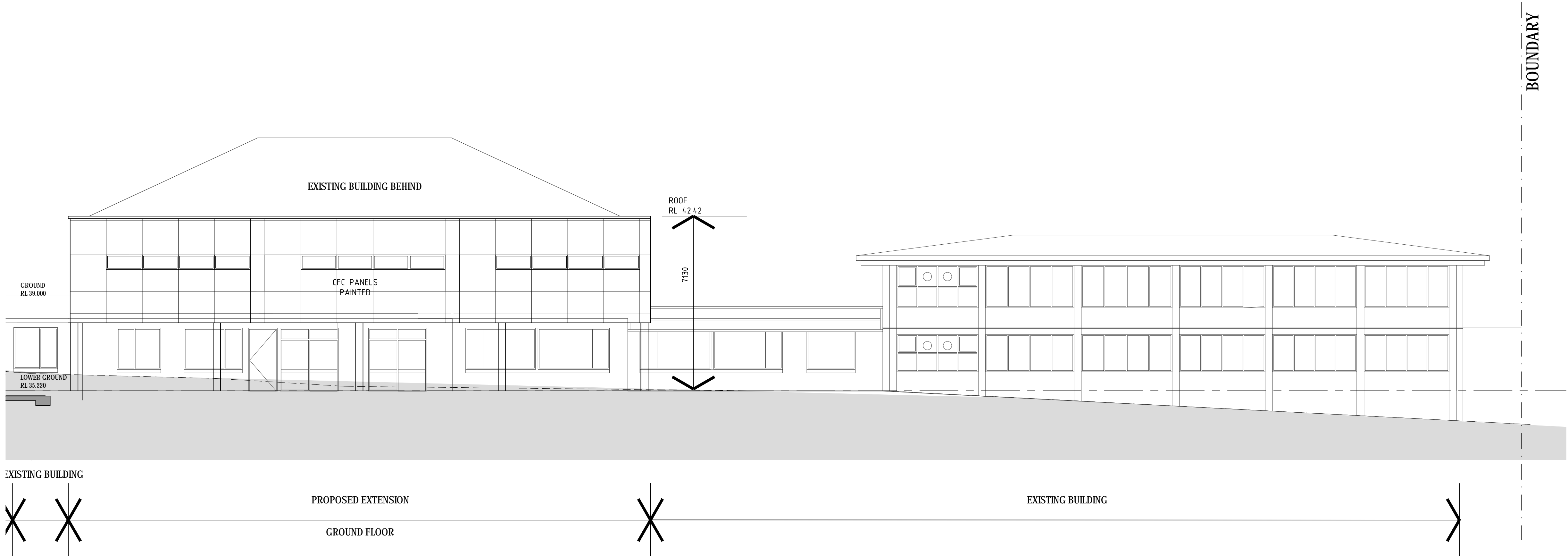
ELEVATION - EAST
