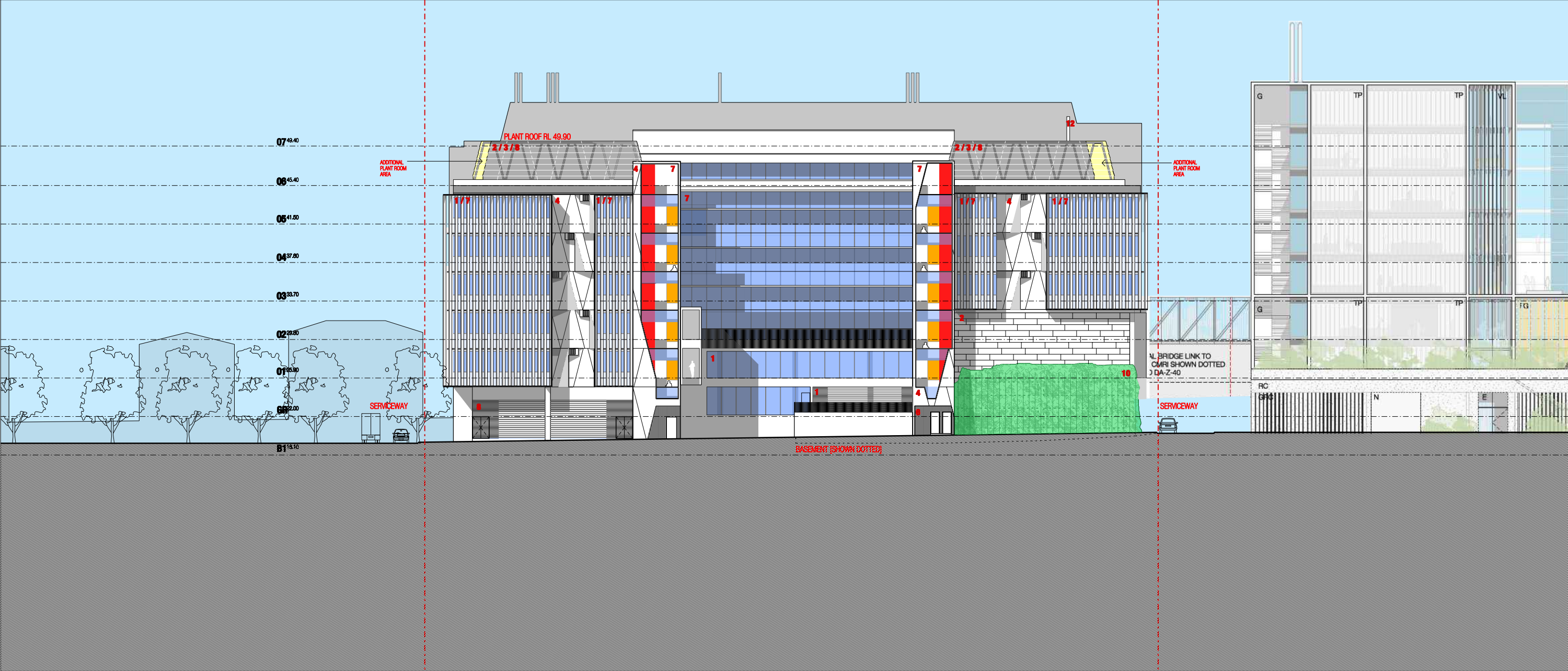
1 NORTH ELEVATION SCALE 1:200
