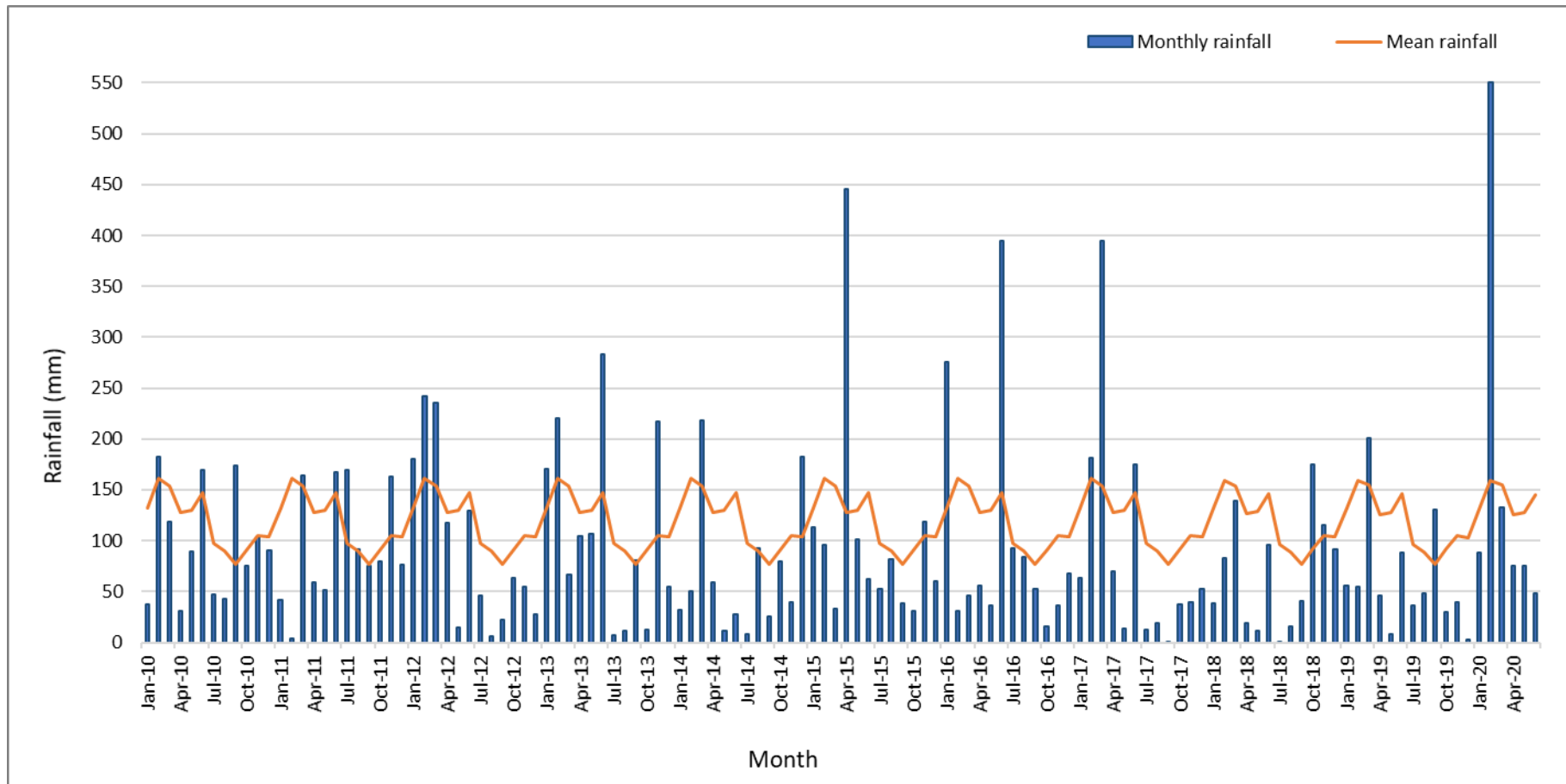
Figure 6: Monthly rainfall for the study area (January 2010 to June 2020).
