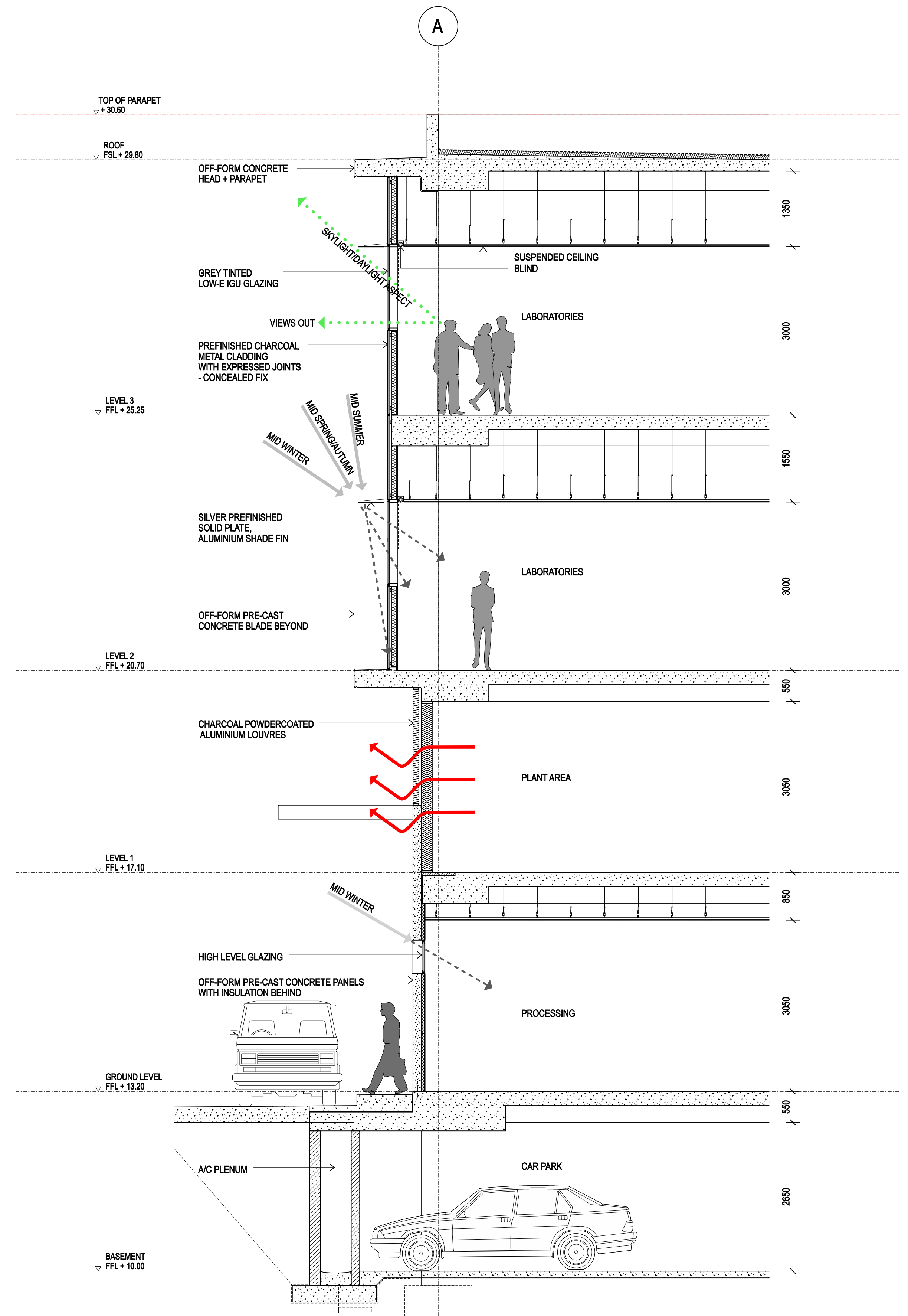
02 DETAIL SECTION - NORTH FACADE 1:50
