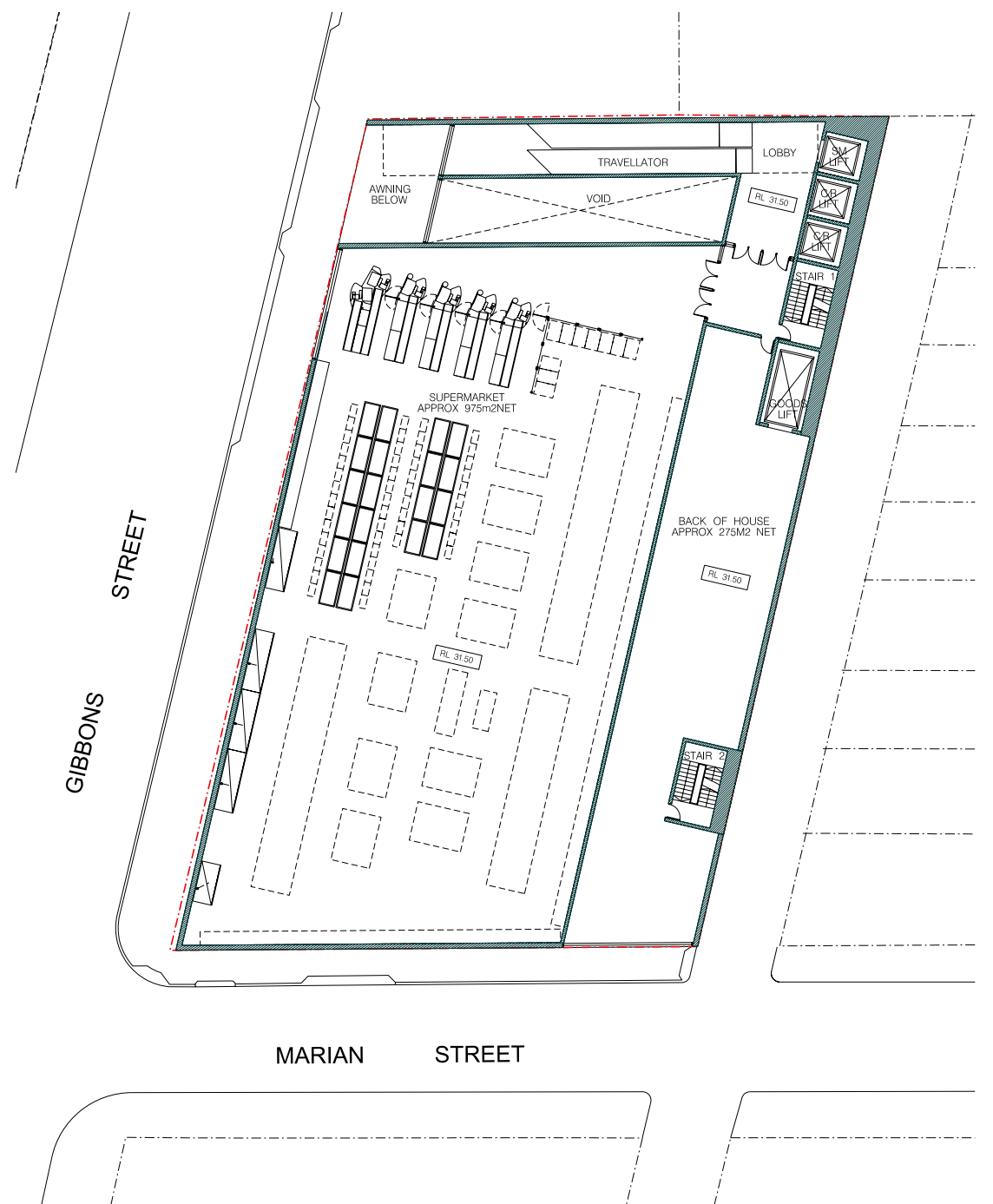
02 LEVEL 1 FLOOR PLAN 1:200
