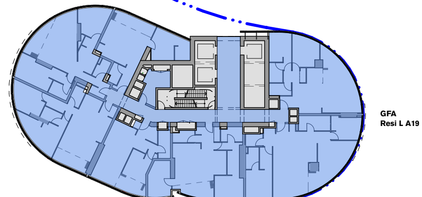
LEVEL 27 A19 1:500
