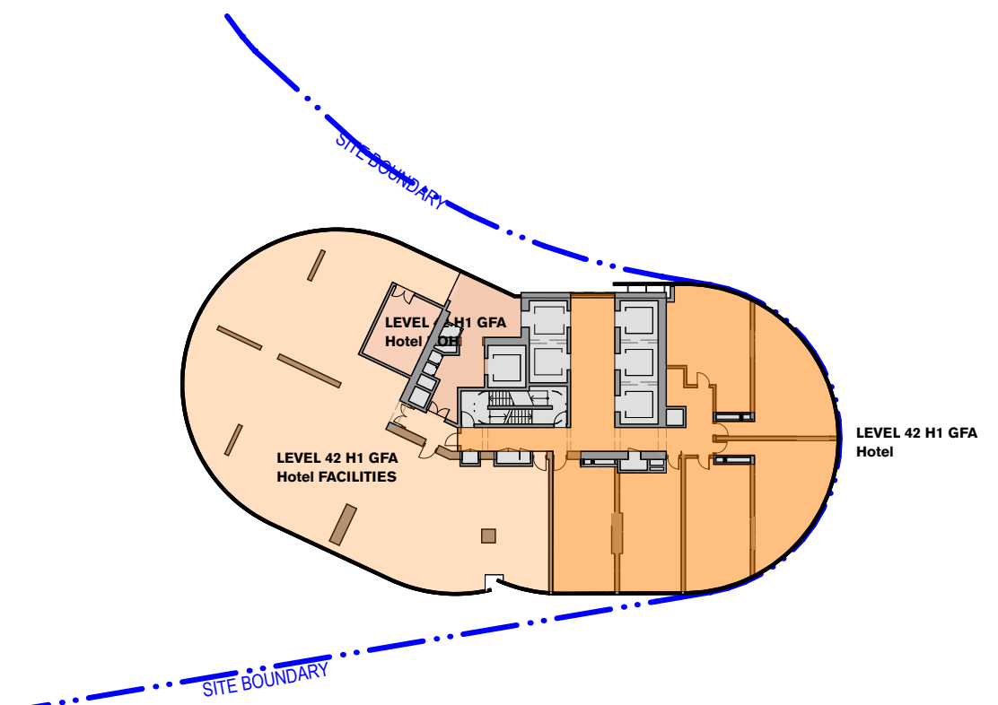
LEVEL 42 H1 - Hotel BOH 1:500
