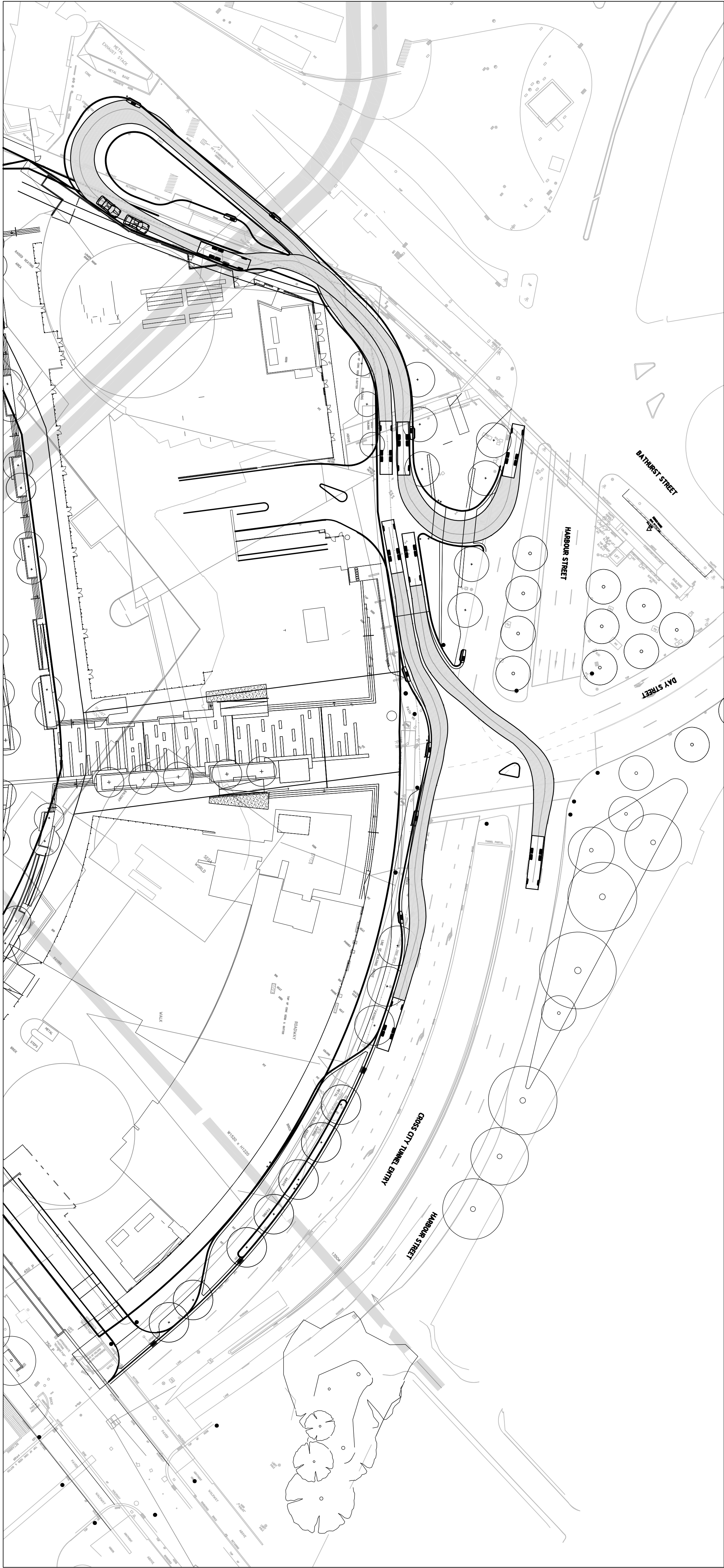
AUSTRALIAN STANDARDS 10.7m HRV @ 15Km/h BASED ON AUSTRALIAN STANDARDS 1989 HEAVY RIGID VEHICLE TEMPLATE
