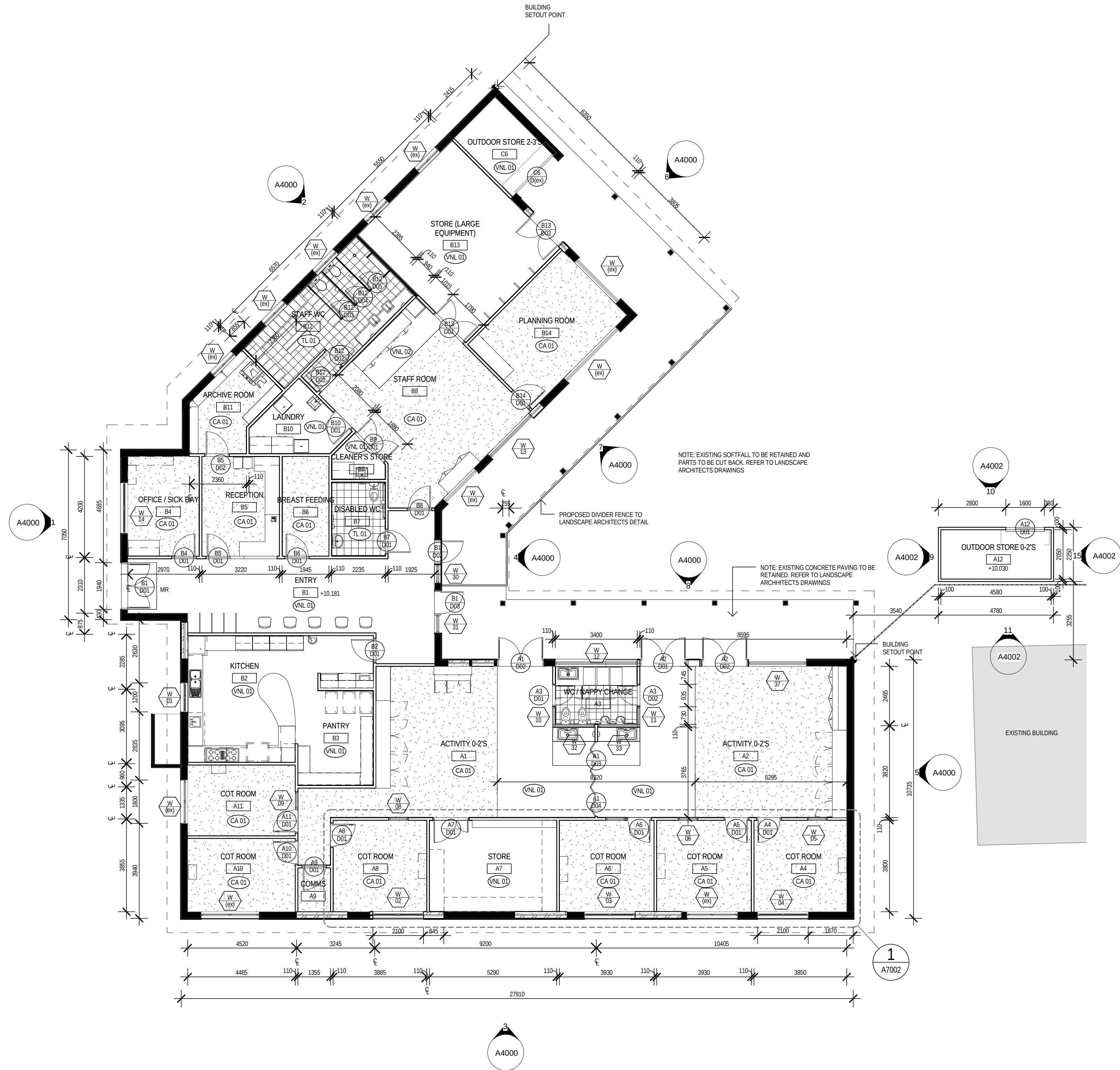
1 GROUND FLOOR BUILDING A 1 : 100
