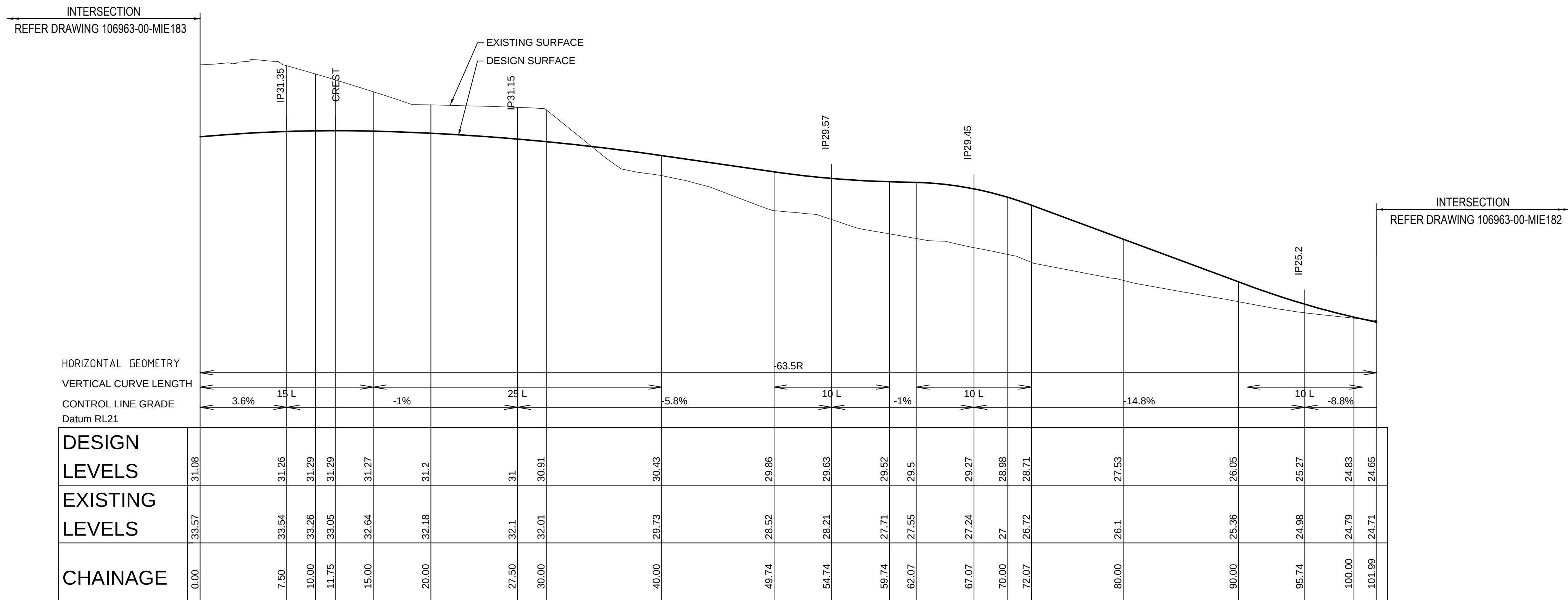
LONGITUDINAL SECTION AMBULANCE ACCESS DRIVEWAY 2a
