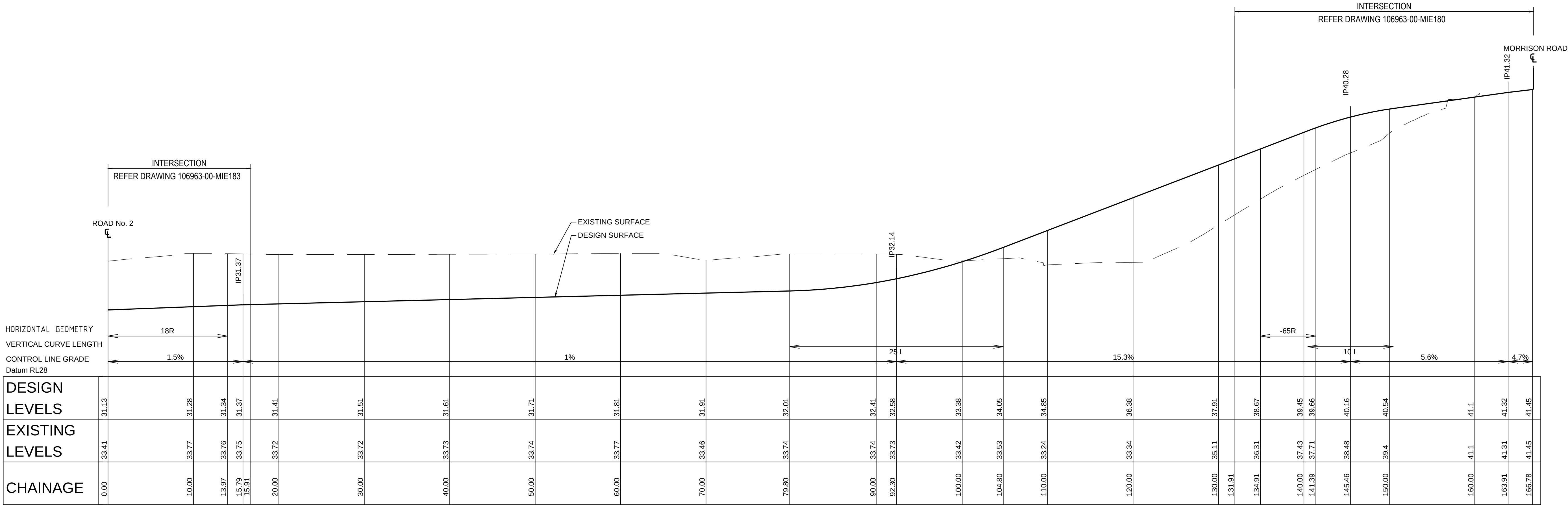
LONGITUDINAL SECTION ROAD 6
