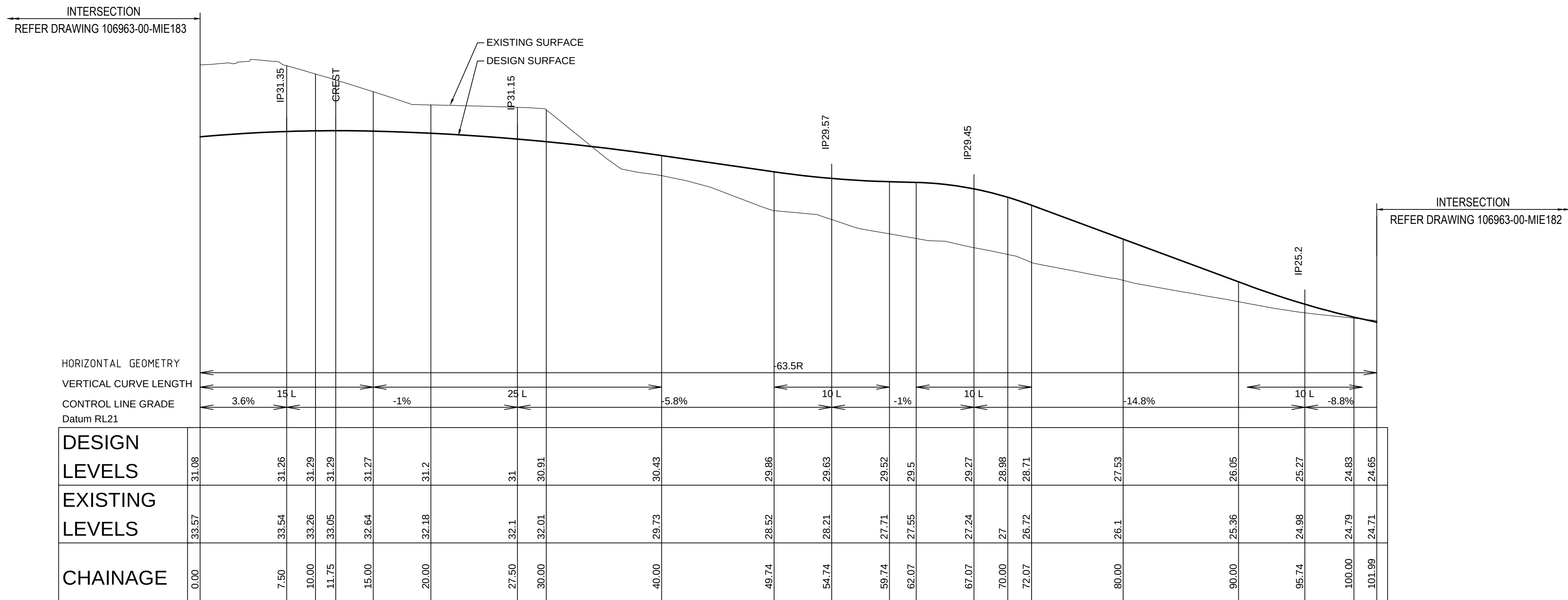
LONGITUDINAL SECTION ROAD 2a HORIZONTAL SCALE 1:250 VERTICAL SCALE 1:100
