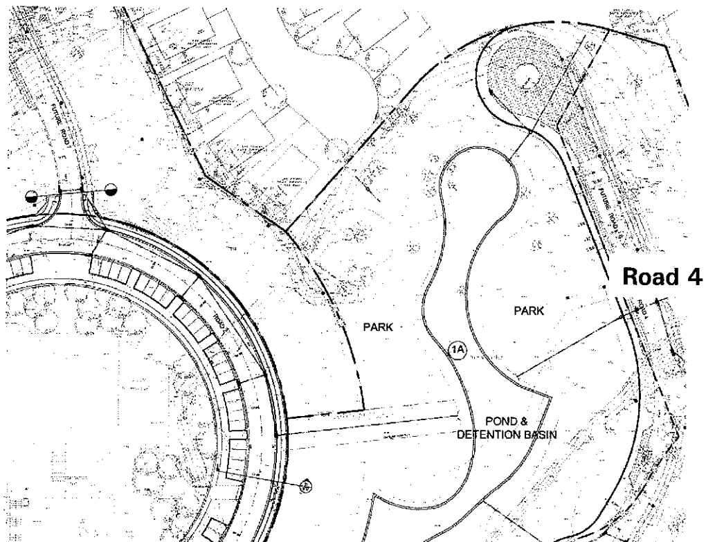
Figure 2 – Road 4 marked in the initial approved as “Future Road” (eastern side of detention basin) (Source: Meinhardt)
