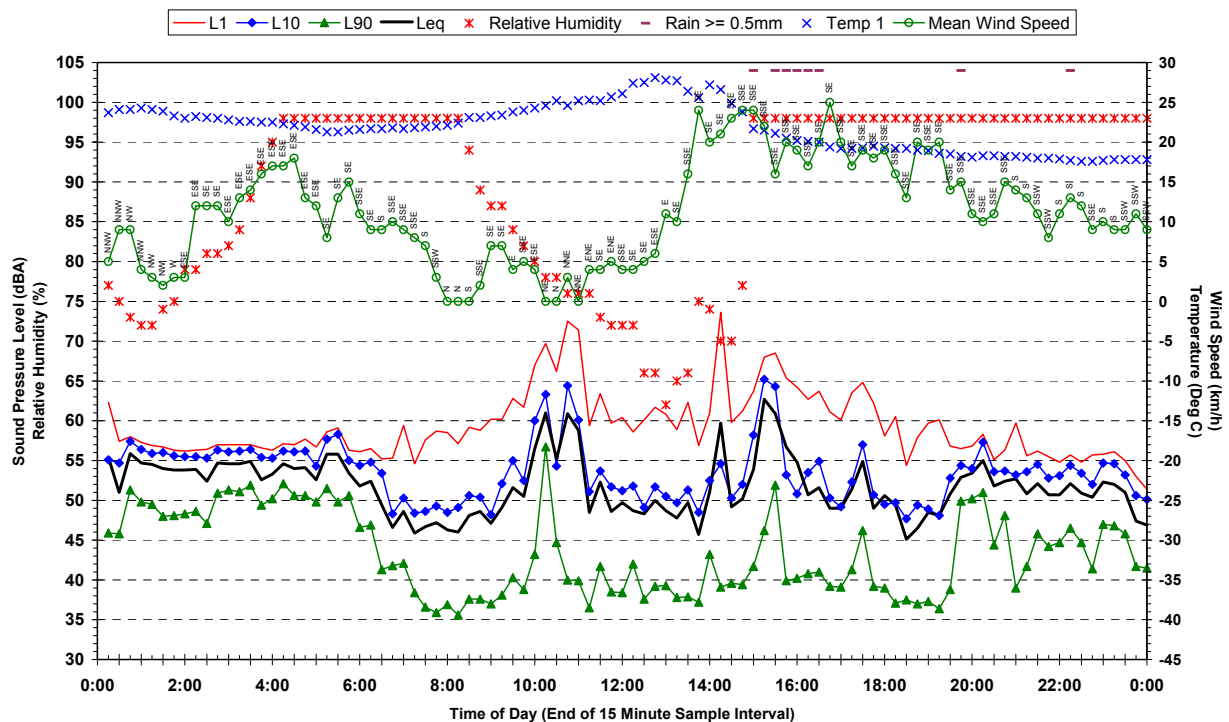
Statistical Ambient Noise Levels 51 Hunter Street, Riverstone - Saturday 17 March 2007
