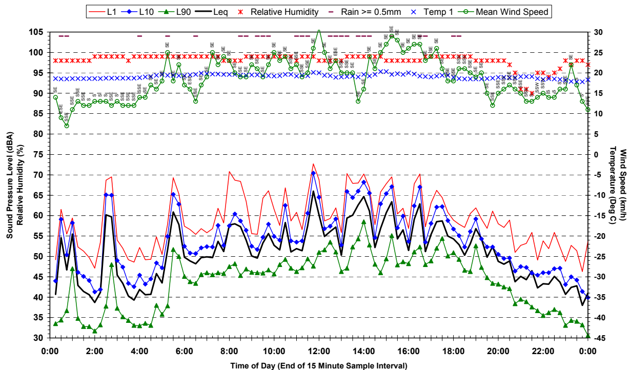
Statistical Ambient Noise Levels 3 Richards Avenue, Riverstone - Monday 12 February 2007
