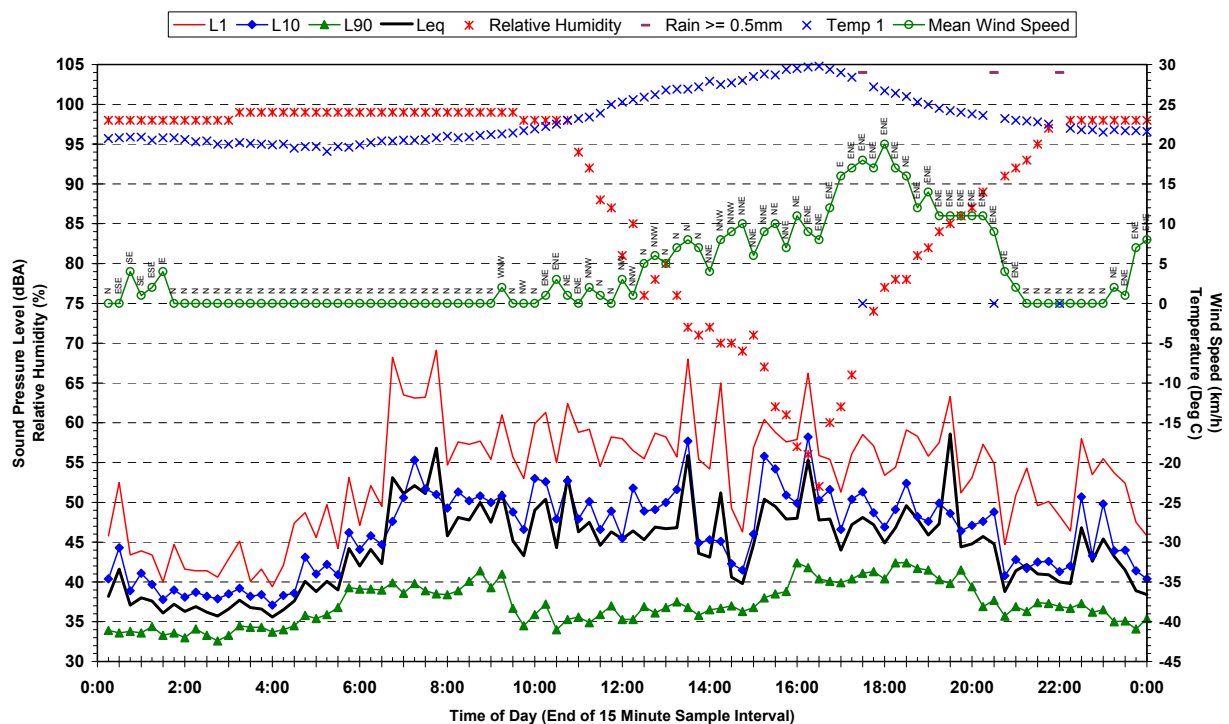
Statistical Ambient Noise Levels 155 Bridge Street, Schofields - Friday 23 March 2007
