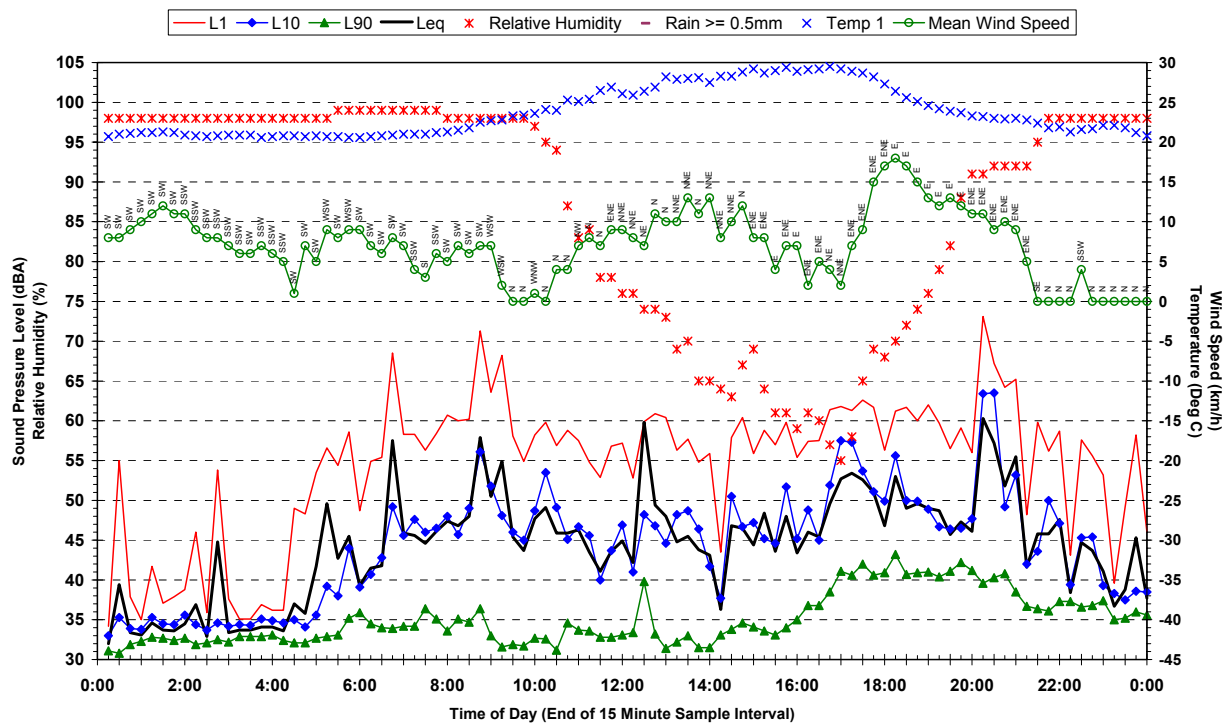
Statistical Ambient Noise Levels 63 Manorhouse Boulevard, Quakers Hill - Thursday 22 March 2007
