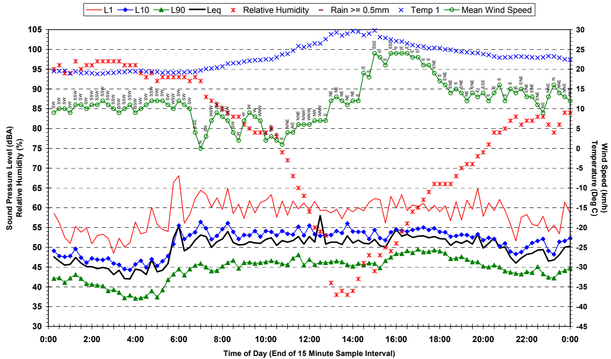
Statistical Ambient Noise Levels Kerry Jones Child Care Centre, Quakers Hill - Saturday 10 February 2007
