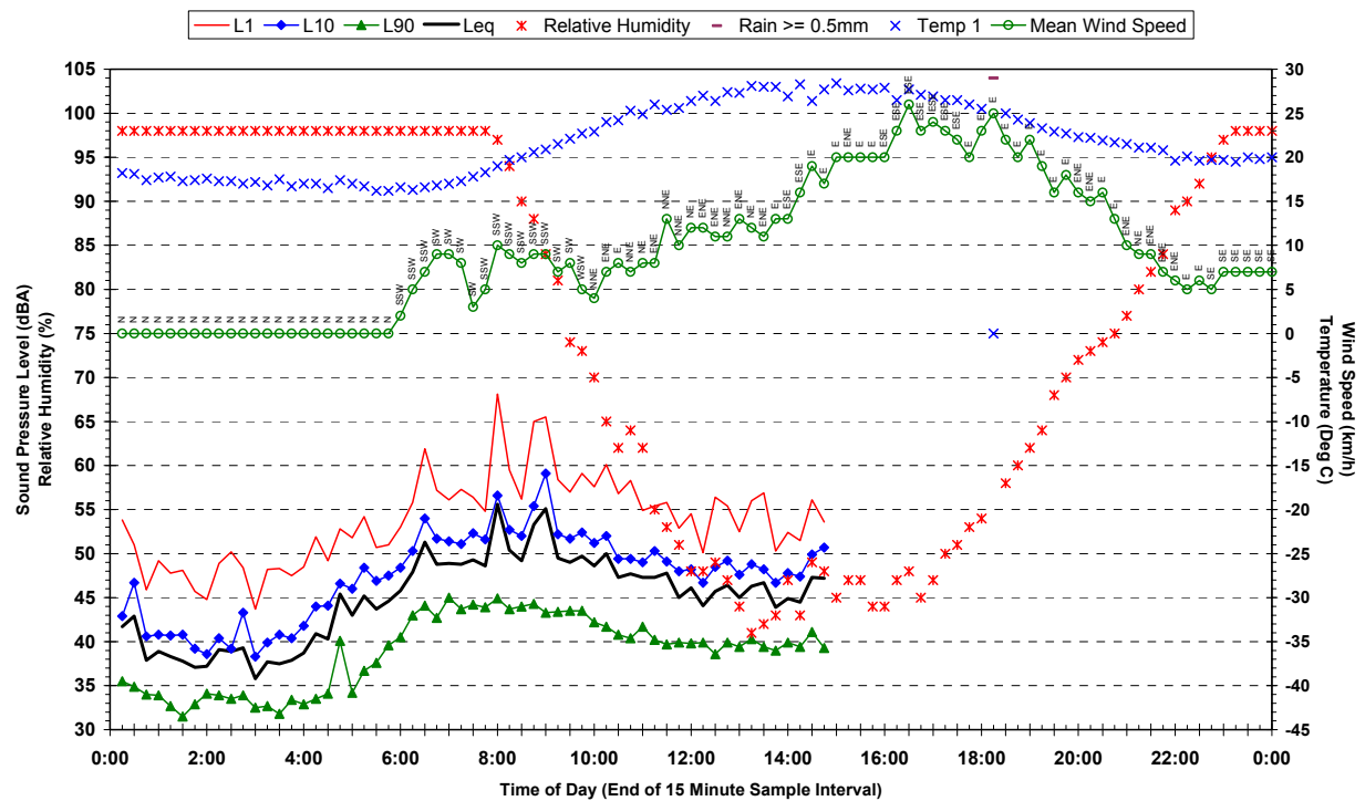
Statistical Ambient Noise Levels 3 Richards Avenue, Riverstone - Thursday 15 February 2007
