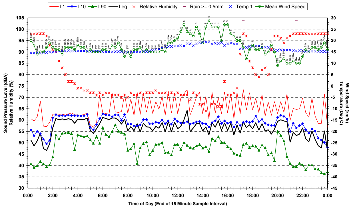
Statistical Ambient Noise Levels 128A Railway Terrace, Riverstone - Sunday 25 March 2007
