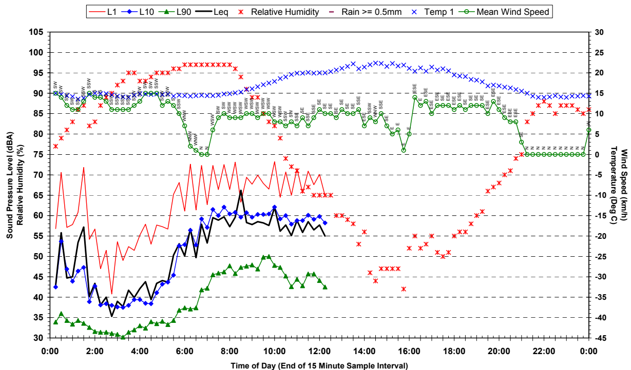
Statistical Ambient Noise Levels 128A Railway Terrace, Riverstone - Tuesday 27 March 2007
