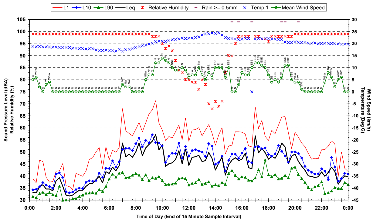
Statistical Ambient Noise Levels 155 Bridge Street, Schofields - Monday 19 March 2007
