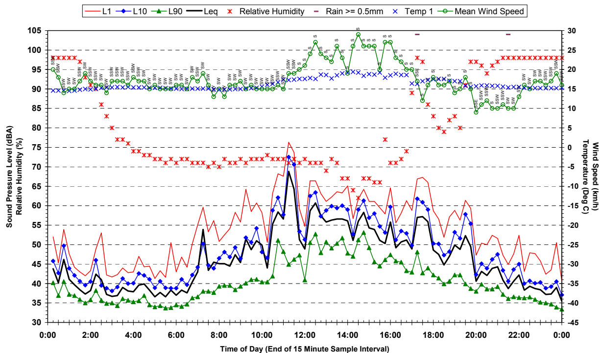
Statistical Ambient Noise Levels 155 Bridge Street, Schofields - Sunday 25 March 2007
