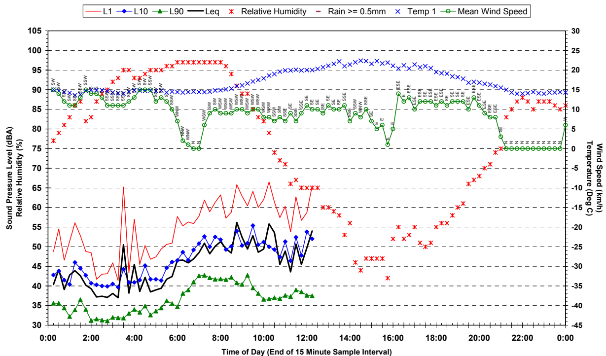
Statistical Ambient Noise Levels 51 Hunter Street, Riverstone - Tuesday 27 March 2007
