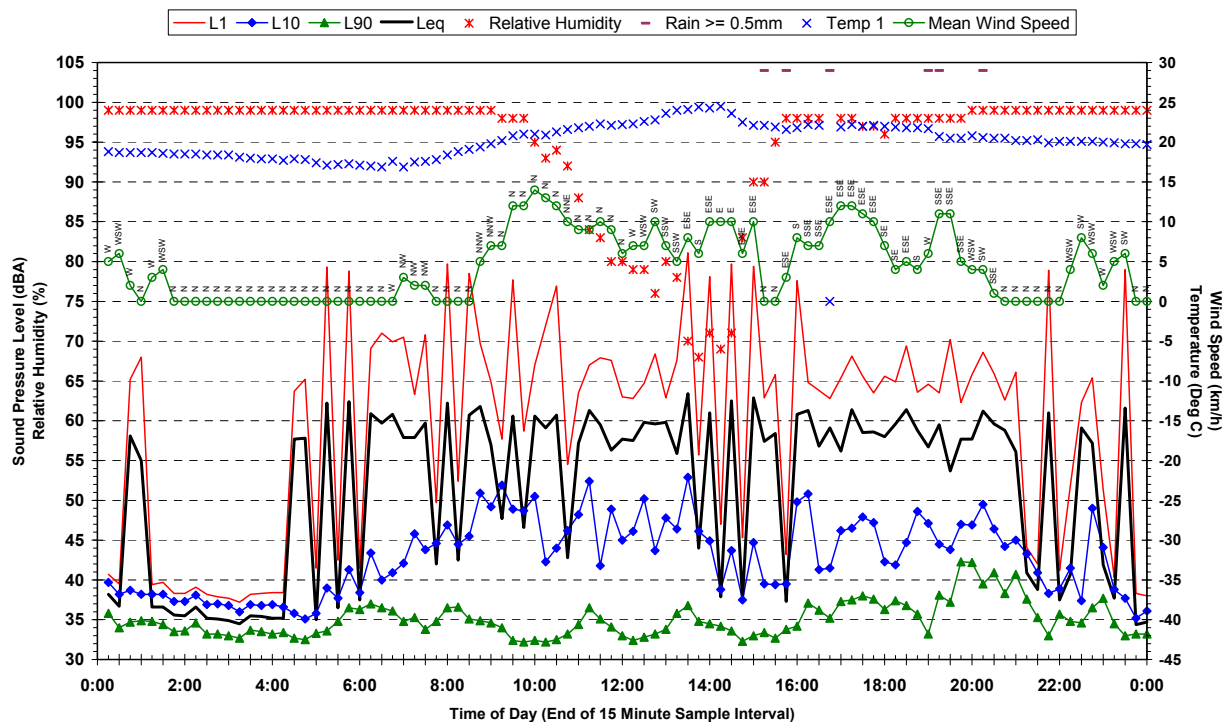
Statistical Ambient Noise Levels Reycroft Avenue, Quakers Hill - Monday 19 March 2007
