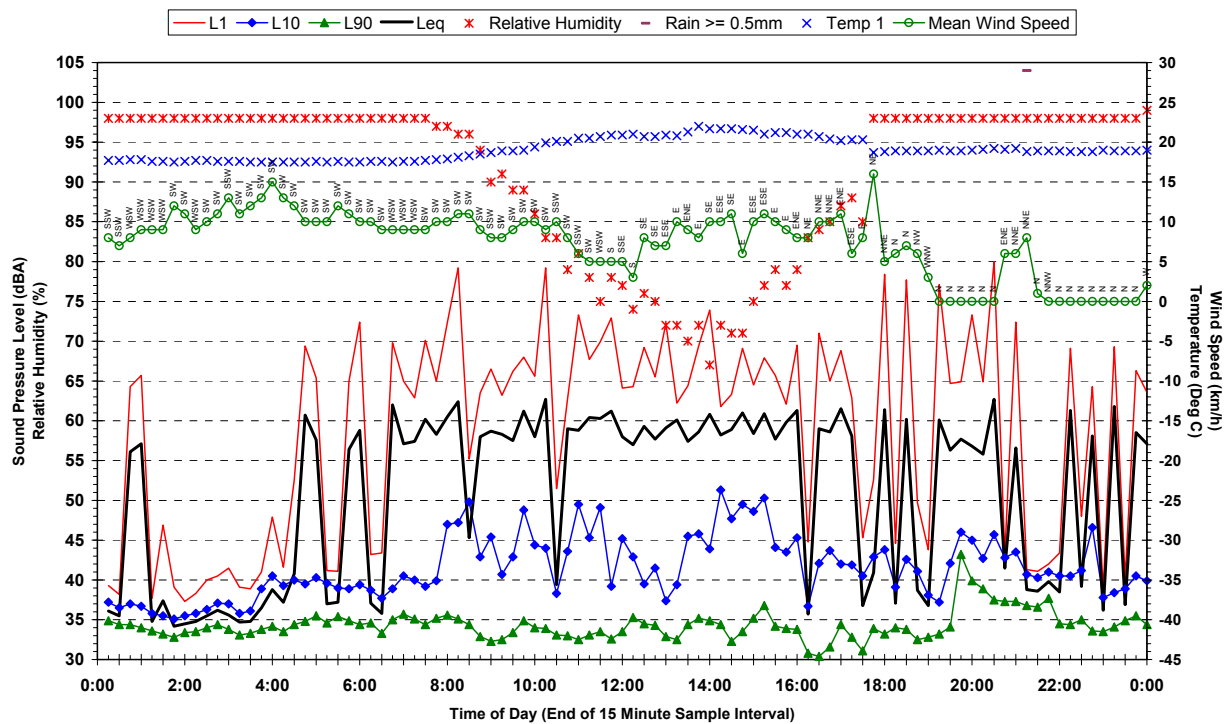
Statistical Ambient Noise Levels Reycroft Avenue, Quakers Hill - Sunday 18 March 2007
