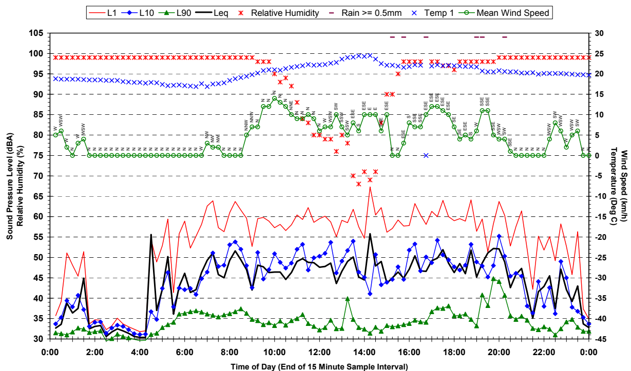
Statistical Ambient Noise Levels 63 Manorhouse Boulevard, Quakers Hill - Monday 19 March 2007
