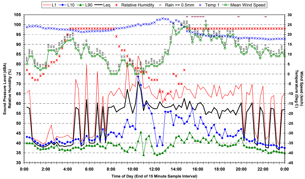
Statistical Ambient Noise Levels Reycroft Avenue, Quakers Hill - Saturday 17 March 2007
