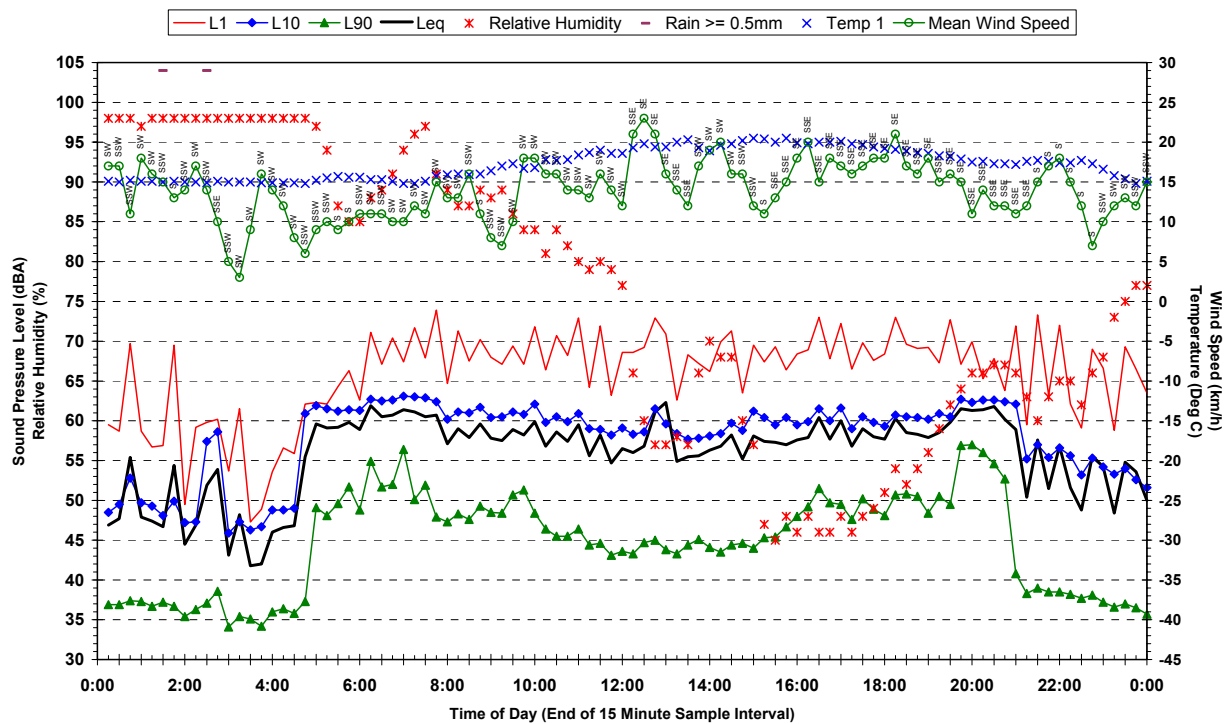
Statistical Ambient Noise Levels 128A Railway Terrace, Riverstone - Monday 26 March 2007
