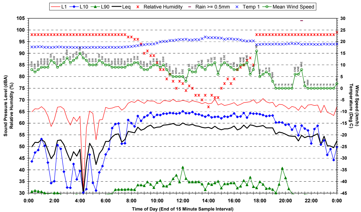
Statistical Ambient Noise Levels Corner Otago Street and Riverstone Parade, Vineyard - Sunday 18 March 2007
