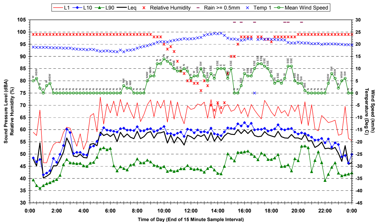
Statistical Ambient Noise Levels 128A Railway Terrace, Riverstone - Monday 19 March 2007
