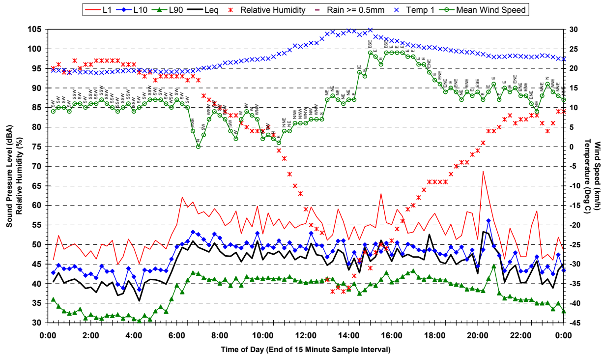
Statistical Ambient Noise Levels 3 Richards Avenue, Riverstone - Saturday 10 February 2007
