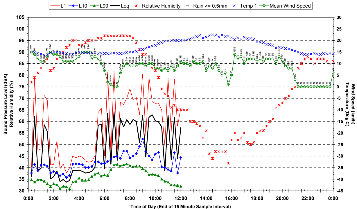
Statistical Ambient Noise Levels Reycroft Avenue, Quakers Hill - Tuesday 27 March 2007
