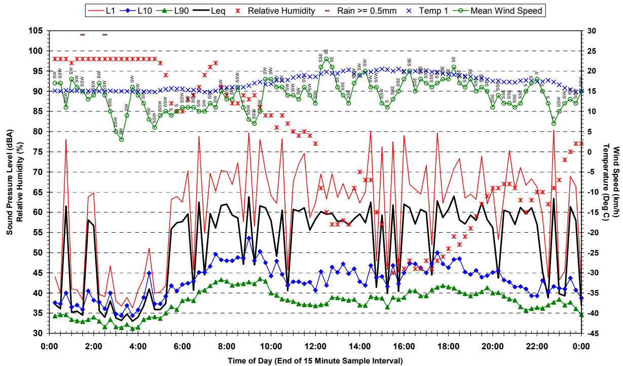
Statistical Ambient Noise Levels Reycroft Avenue, Quakers Hill - Monday 26 March 2007
