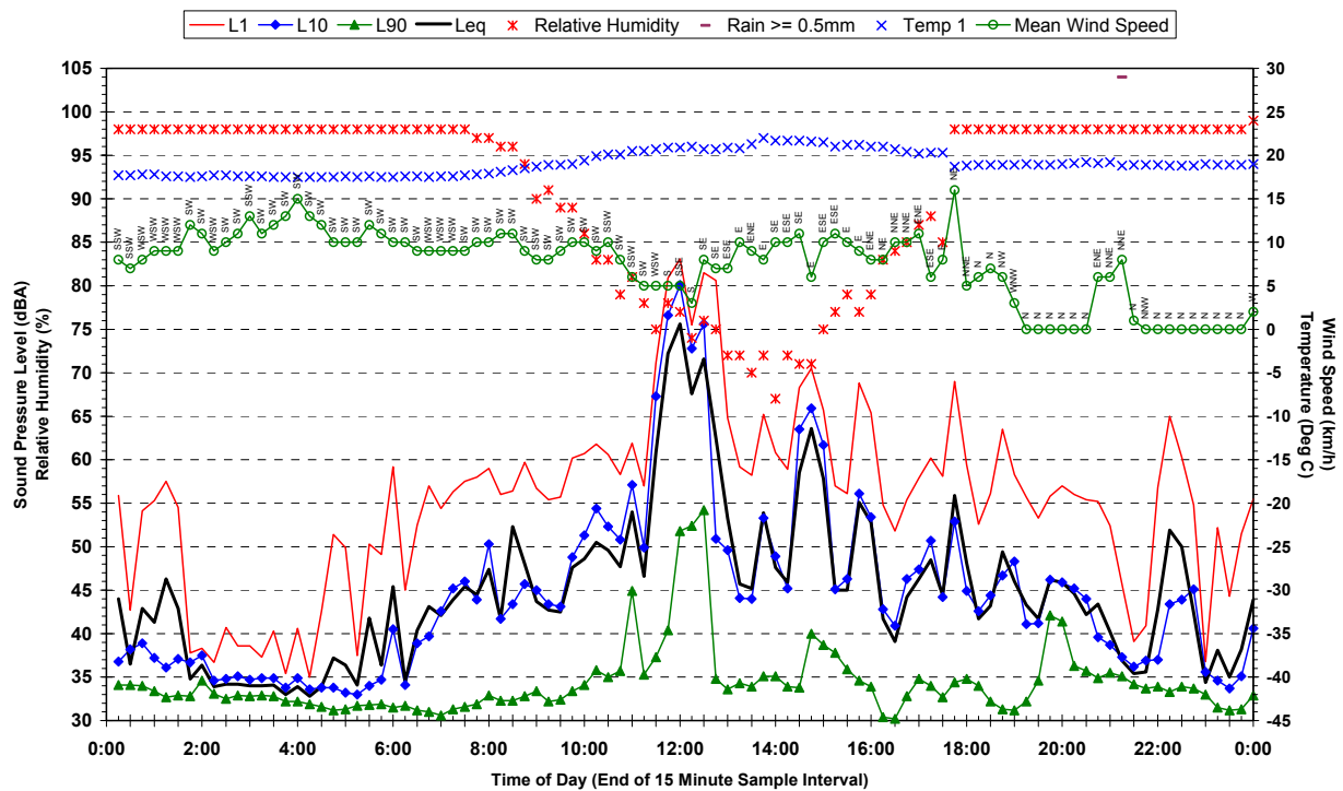
Statistical Ambient Noise Levels 63 Manorhouse Boulevard, Quakers Hill - Sunday 18 March 2007
