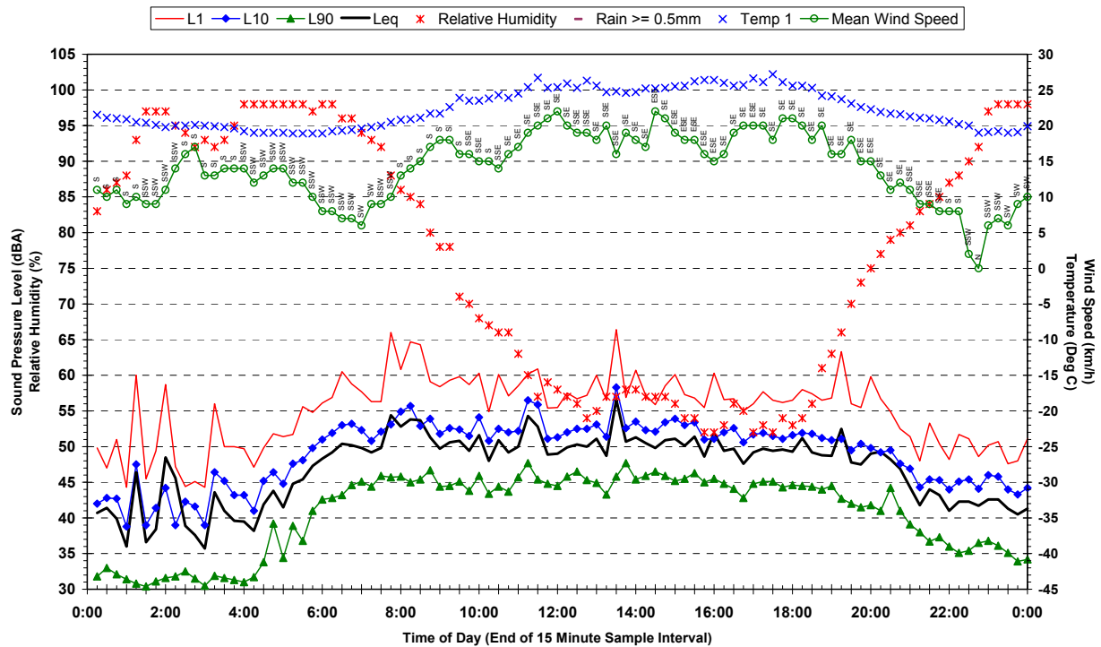
Statistical Ambient Noise Levels 3 Richards Avenue, Riverstone - Friday 9 February 2007
