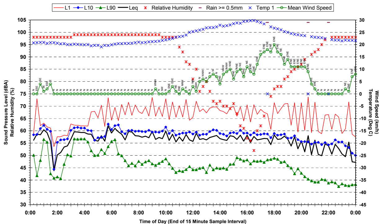
Statistical Ambient Noise Levels 128A Railway Terrace, Riverstone - Friday 23 March 2007
