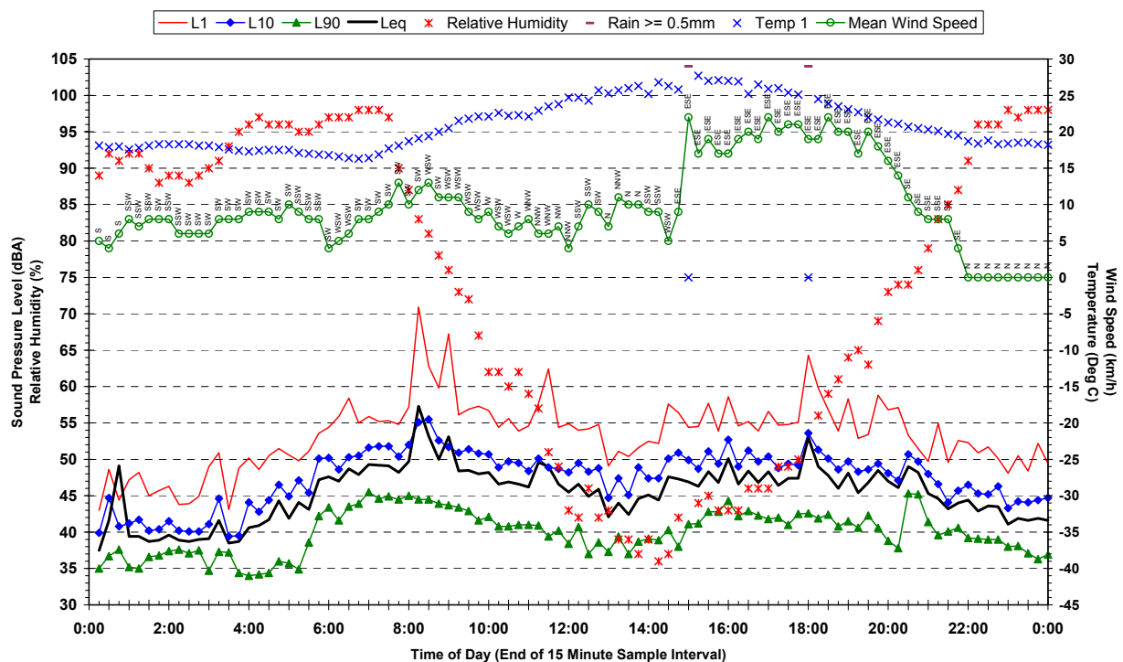
Statistical Ambient Noise Levels 3 Richards Avenue, Riverstone - Wednesday 14 February 2007
