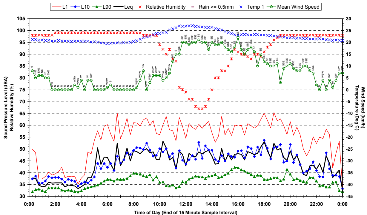
Statistical Ambient Noise Levels 63 Manorhouse Boulevard, Quakers Hill - Wednesday 21 March 2007
