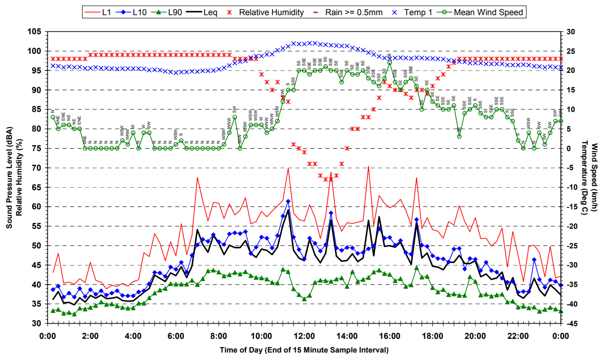
Statistical Ambient Noise Levels 155 Bridge Street, Schofields - Wednesday 21 March 2007
