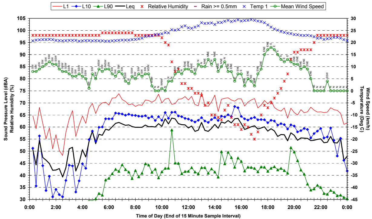
Statistical Ambient Noise Levels Corner Dulwich Road and Riverstone Parade, Vineyard - Thursday 22 March 2007
