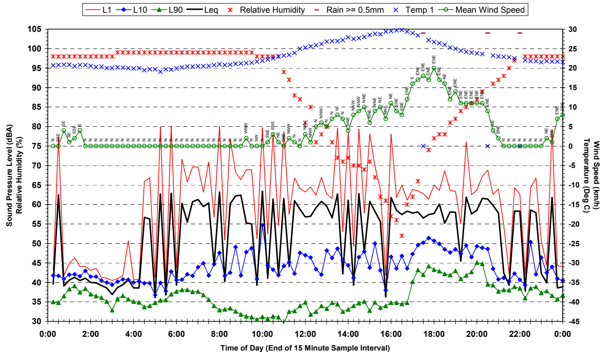
Statistical Ambient Noise Levels Reycroft Avenue, Quakers Hill - Friday 23 March 2007
