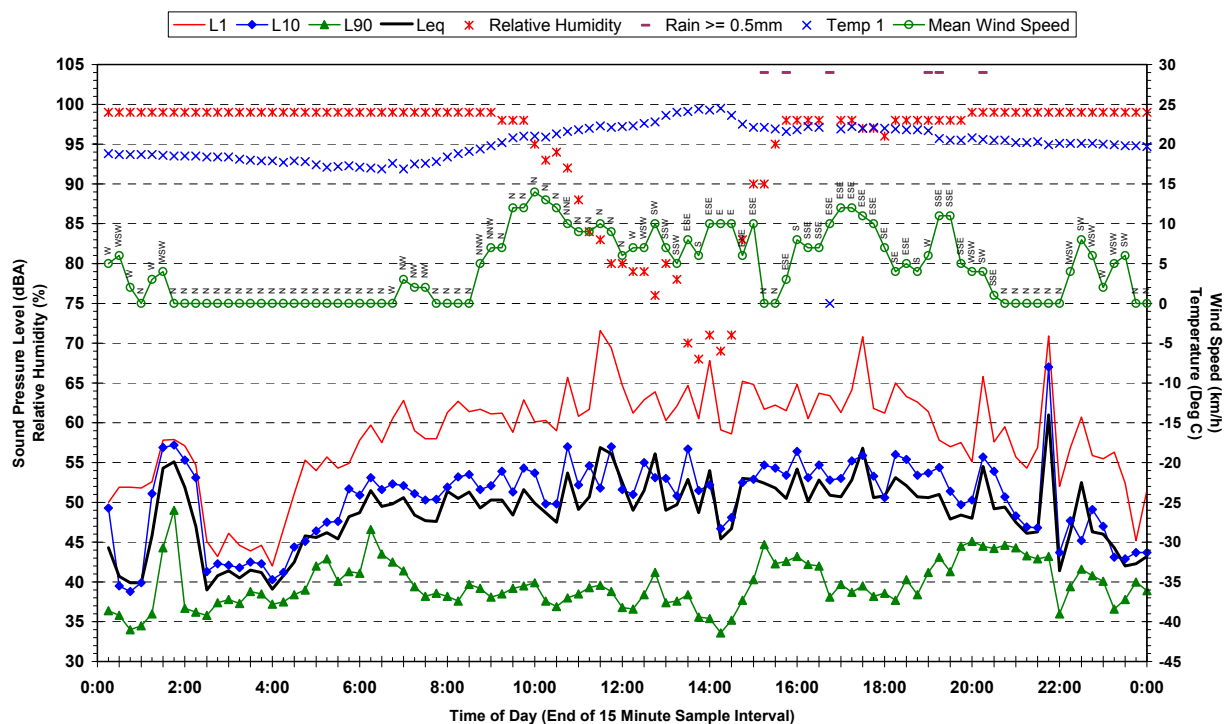
Statistical Ambient Noise Levels 51 Hunter Street, Riverstone - Monday 19 March 2007
