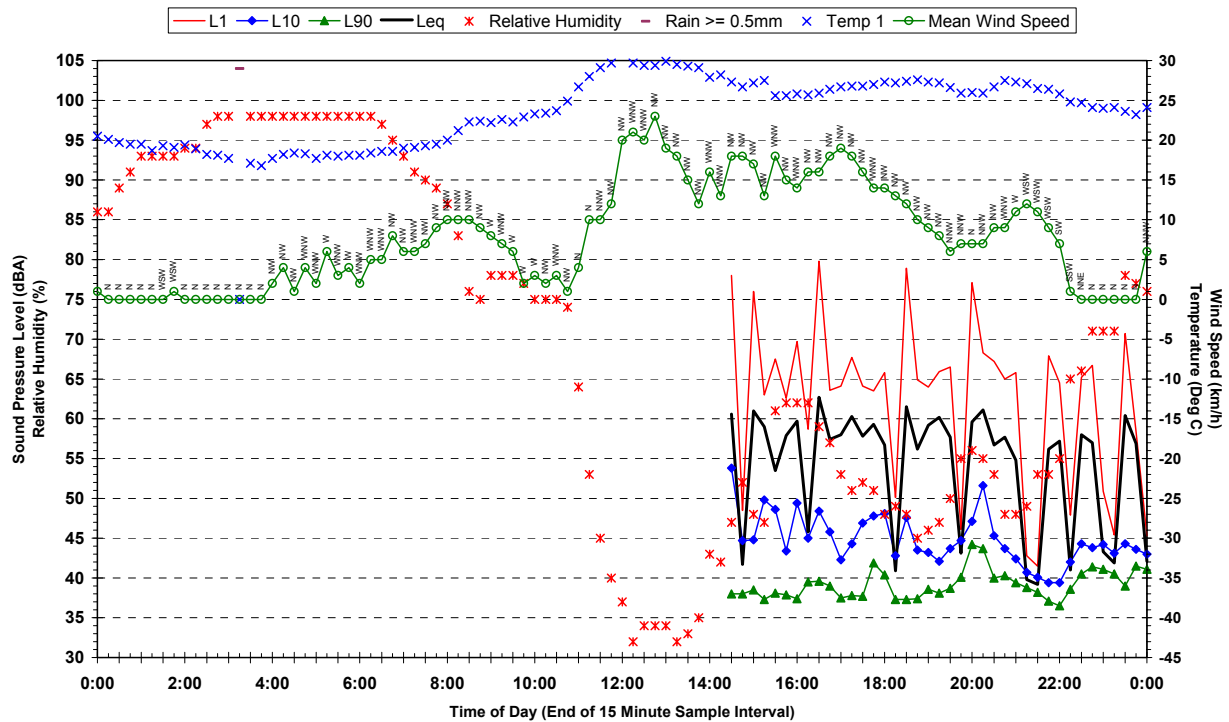
Statistical Ambient Noise Levels Reycroft Avenue, Quakers Hill - Friday 16 March 2007
