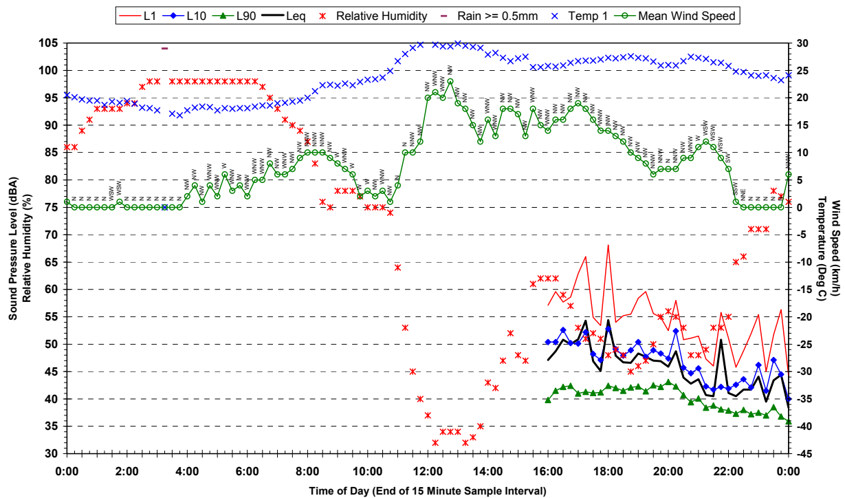
Statistical Ambient Noise Levels 155 Bridge Street, Schofields - Friday 16 March 2007
