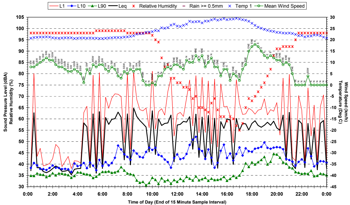
Statistical Ambient Noise Levels Reycroft Avenue, Quakers Hill - Thursday 22 March 2007
