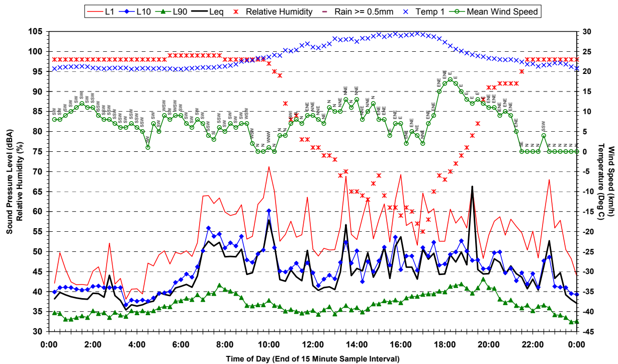
Statistical Ambient Noise Levels 155 Bridge Street, Schofields - Thursday 22 March 2007
