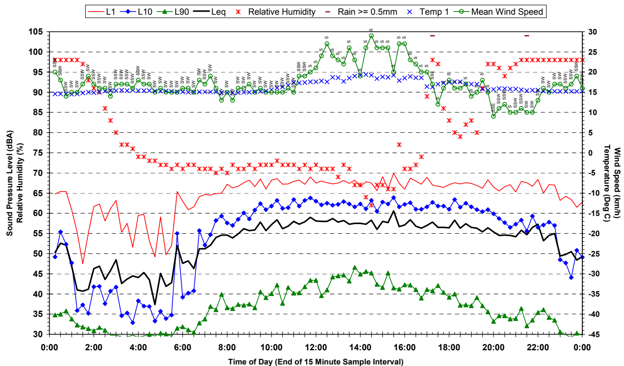
Statistical Ambient Noise Levels Corner Dulwich Road and Riverstone Parade, Vineyard - Sunday 25 March 2007
