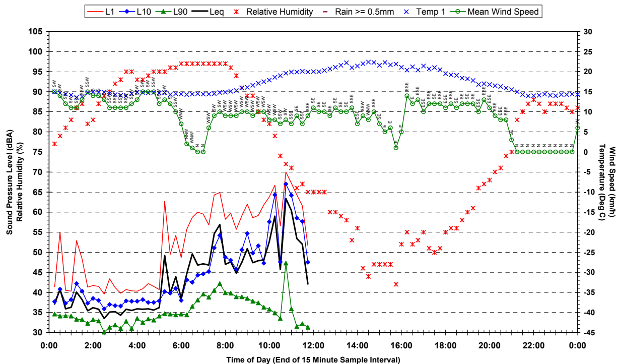
Statistical Ambient Noise Levels 63 Manorhouse Boulevard, Quakers Hill - Tuesday 27 March 2007
