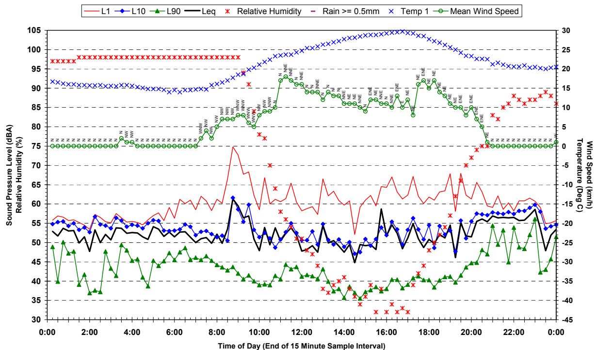
Statistical Ambient Noise Levels 51 Hunter Street, Riverstone - Thursday 15 March 2007
