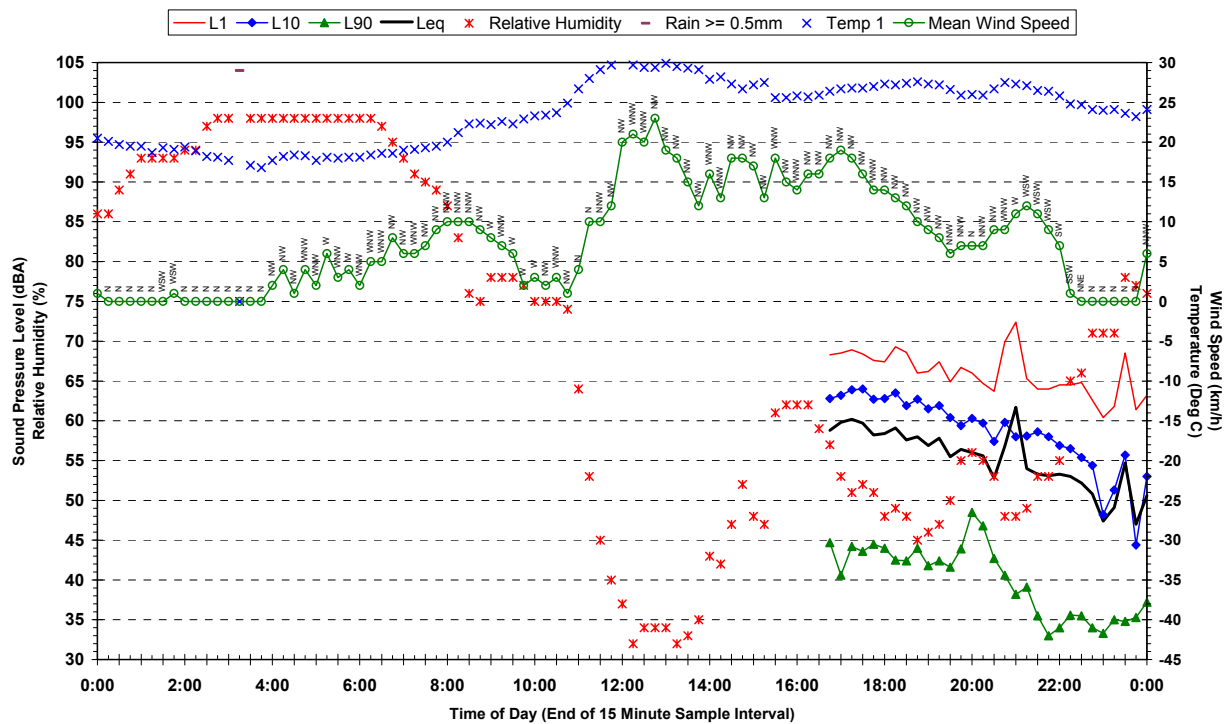
Statistical Ambient Noise Levels Corner Dulwich Road and Riverstone Parade, Vineyard - Friday 16 March 2007
