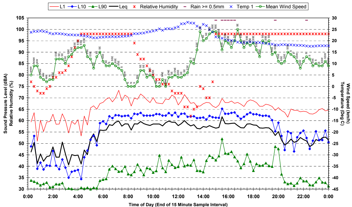
Statistical Ambient Noise Levels Corner Dulwich Road and Riverstone Parade, Vineyard - Saturday 17 March 2007
