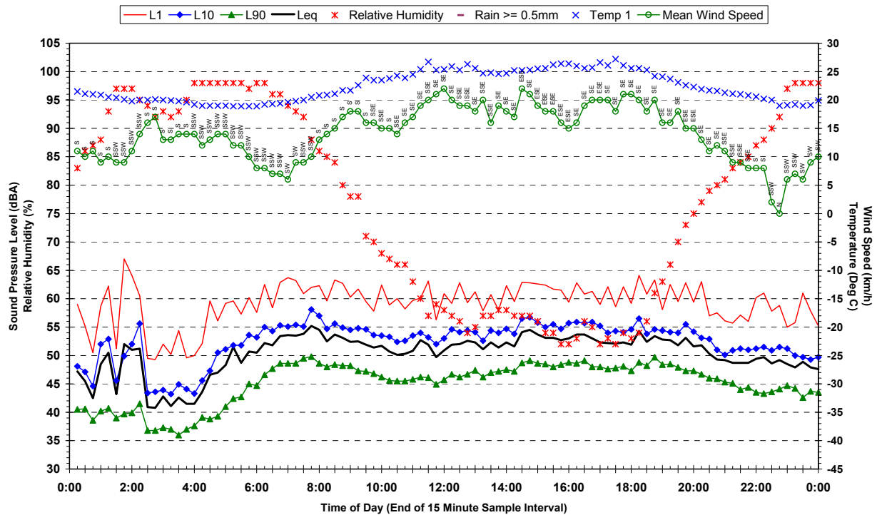
Statistical Ambient Noise Levels Kerry Jones Child Care Centre, Quakers Hill - Friday 9 February 2007
