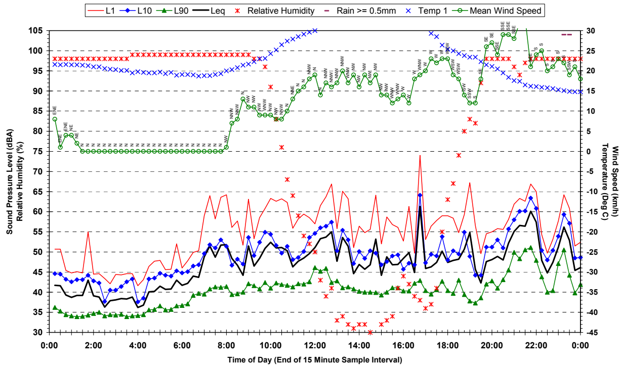
Statistical Ambient Noise Levels 155 Bridge Street, Schofields - Saturday 24 March 2007
