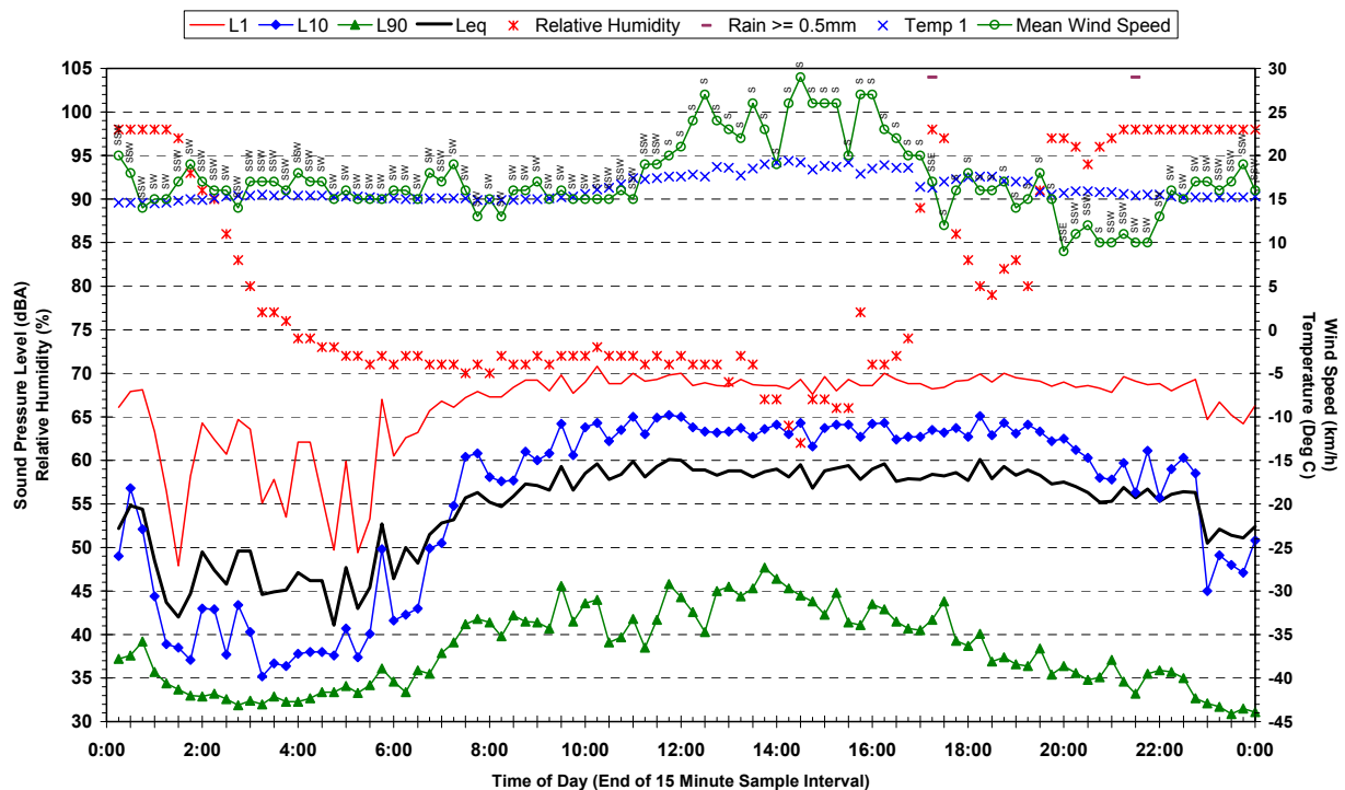
Statistical Ambient Noise Levels Corner Otago Street and Riverstone Parade, Vineyard - Sunday 25 March 2007
