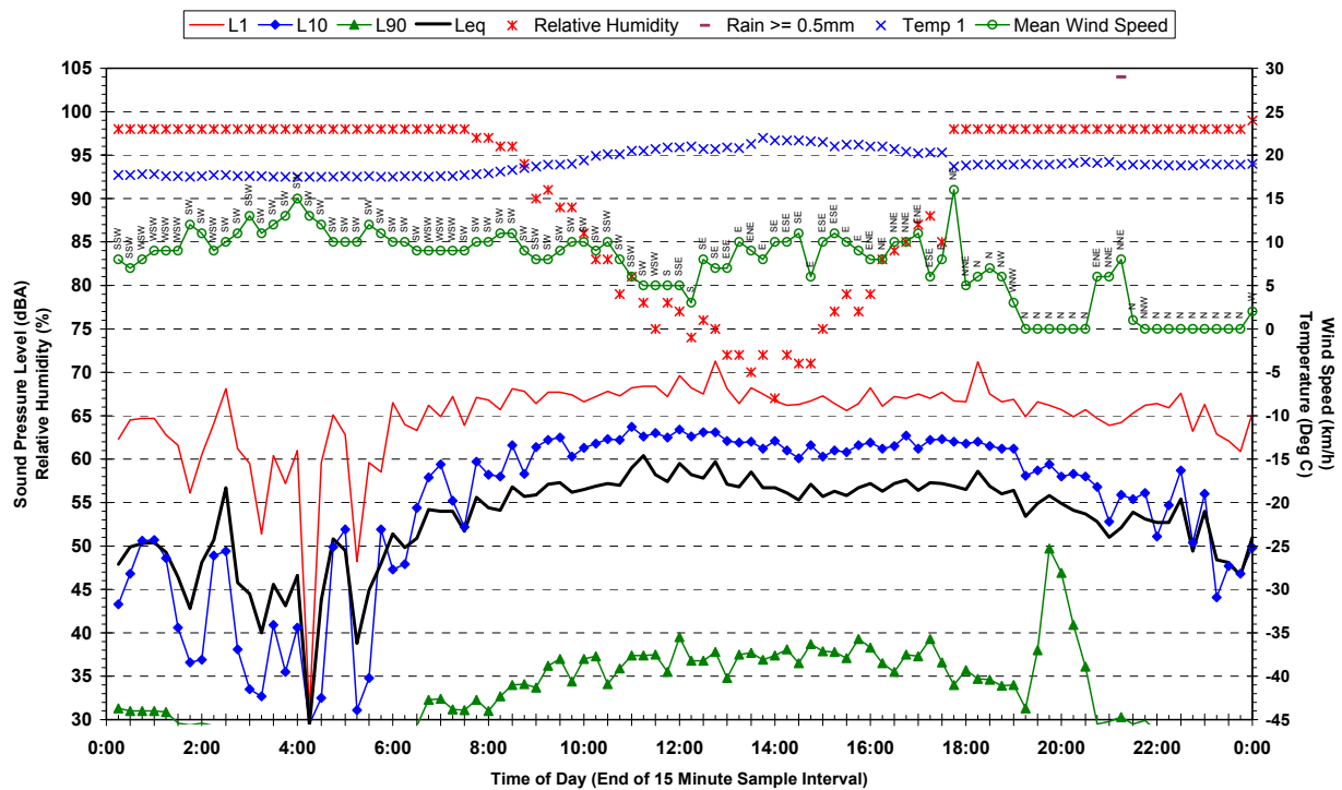
Statistical Ambient Noise Levels Corner Dulwich Road and Riverstone Parade, Vineyard - Sunday 18 March 2007
