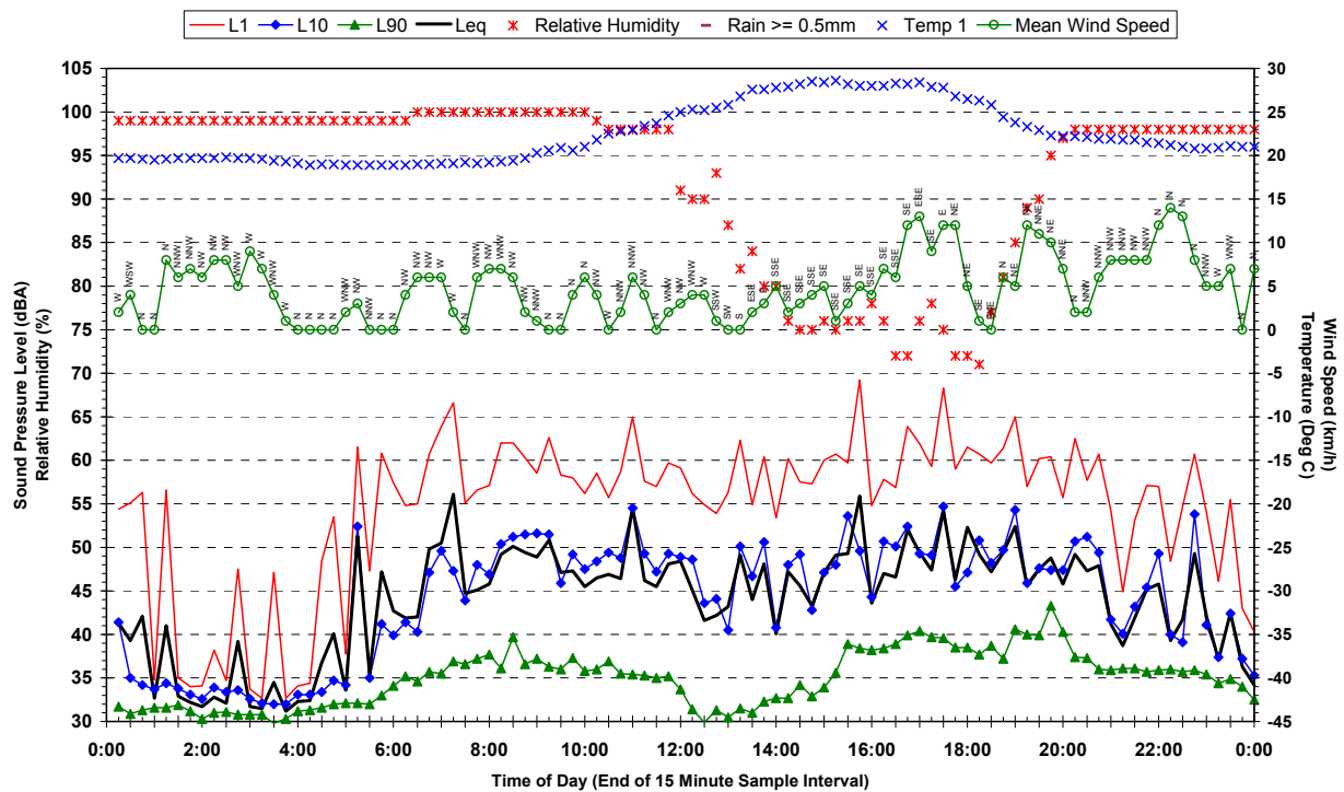
Statistical Ambient Noise Levels 63 Manorhouse Boulevard, Quakers Hill - Tuesday 20 March 2007
