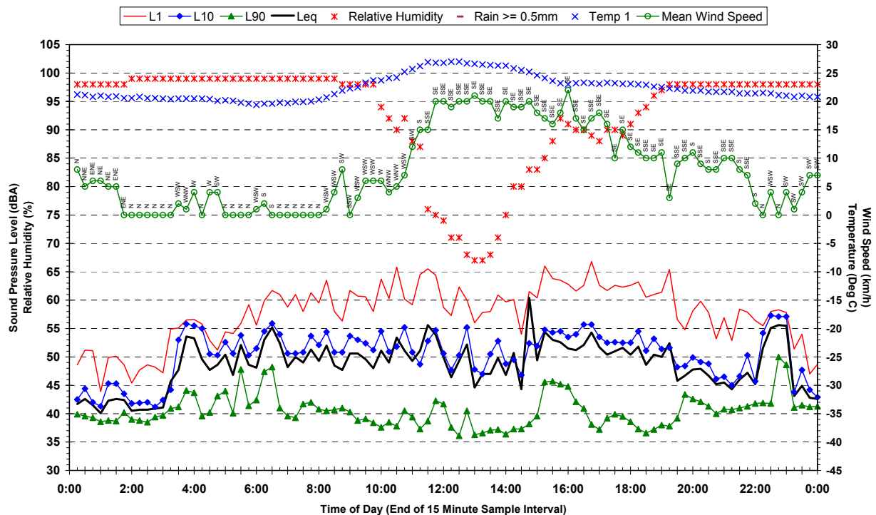
Statistical Ambient Noise Levels 51 Hunter Street, Riverstone - Wednesday 21 March 2007
