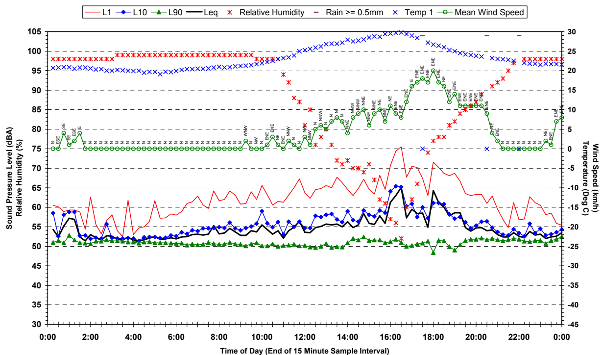
Statistical Ambient Noise Levels 51 Hunter Street, Riverstone - Friday 23 March 2007
