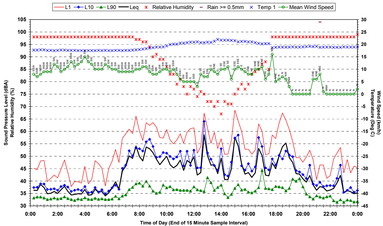
Statistical Ambient Noise Levels 155 Bridge Street, Schofields - Sunday 18 March 2007
