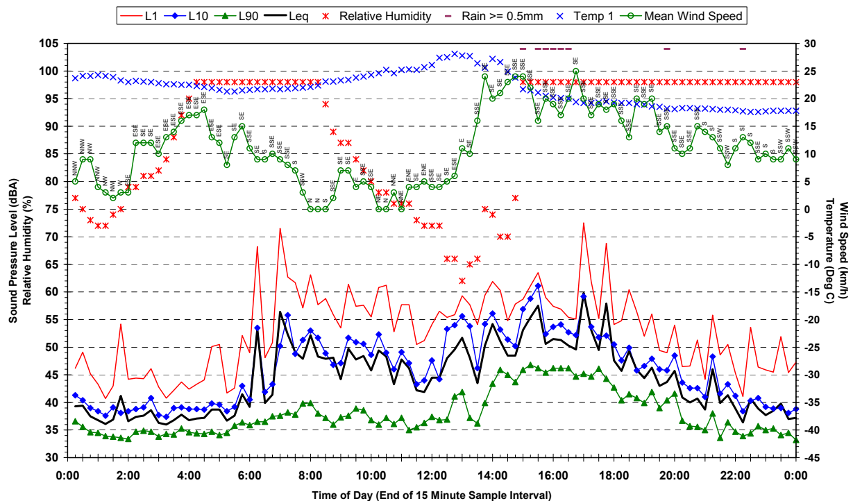
Statistical Ambient Noise Levels 155 Bridge Street, Schofields - Saturday 17 March 2007
