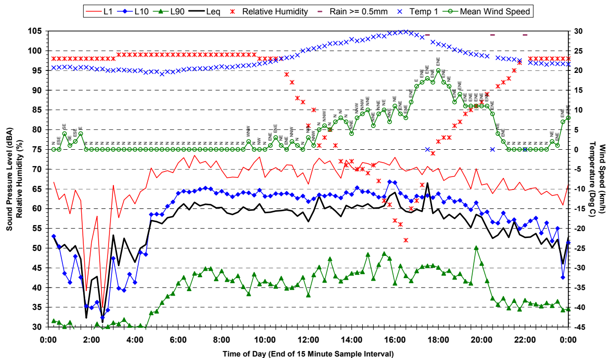
Statistical Ambient Noise Levels Corner Dulwich Road and Riverstone Parade, Vineyard - Friday 23 March 2007
