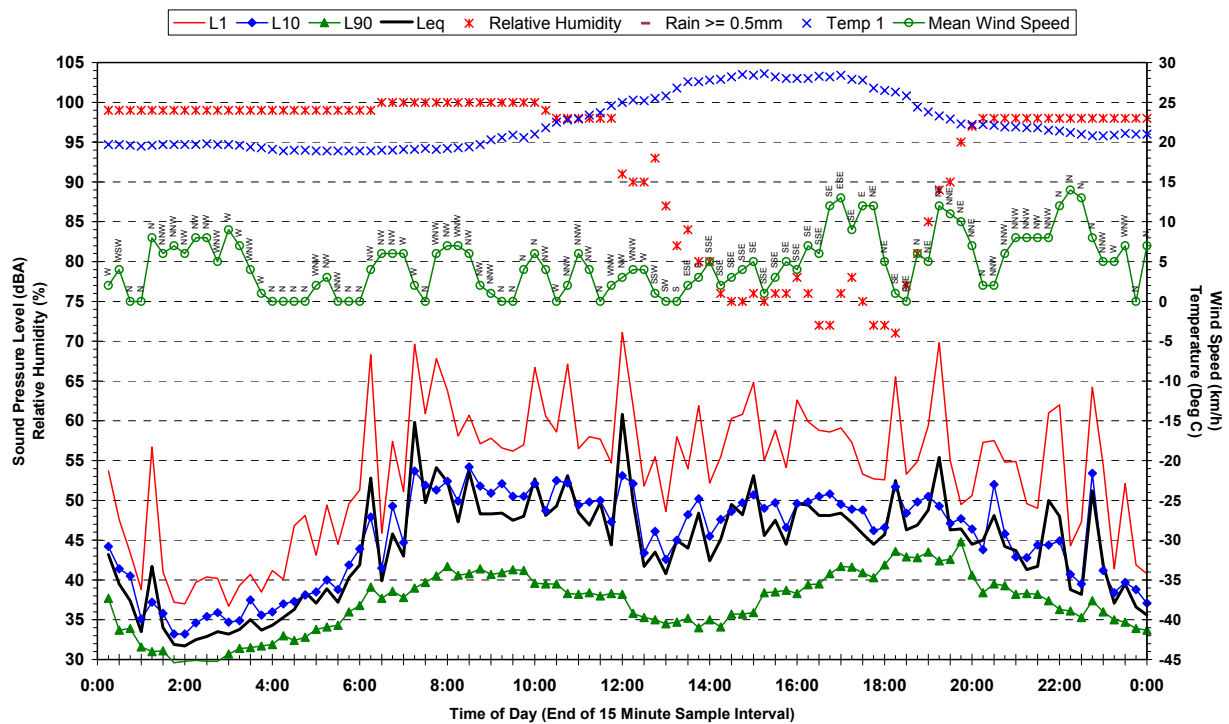
Statistical Ambient Noise Levels 155 Bridge Street, Schofields - Tuesday 20 March 2007
