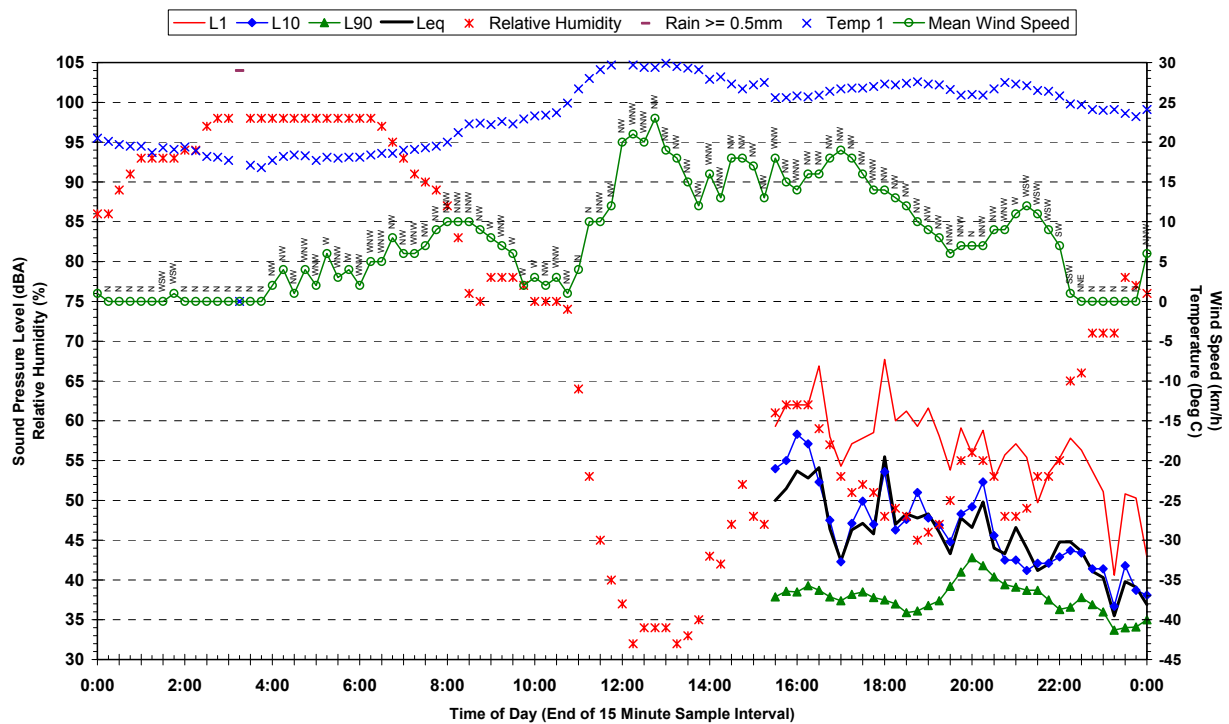
Statistical Ambient Noise Levels 63 Manorhouse Boulevard, Quakers Hill - Friday 16 March 2007
