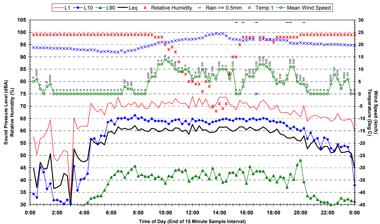
Statistical Ambient Noise Levels Corner Dulwich Road and Riverstone Parade, Vineyard - Monday 19 March 2007
