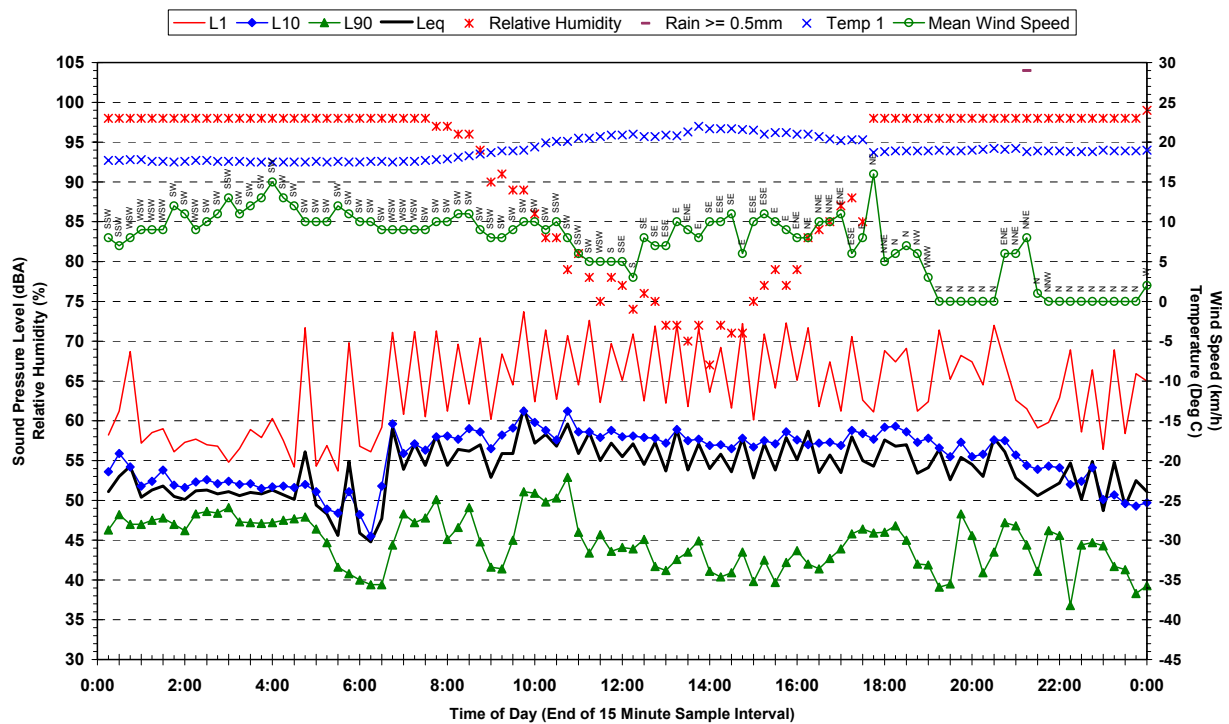
Statistical Ambient Noise Levels 128A Railway Terrace, Riverstone - Sunday 18 March 2007
