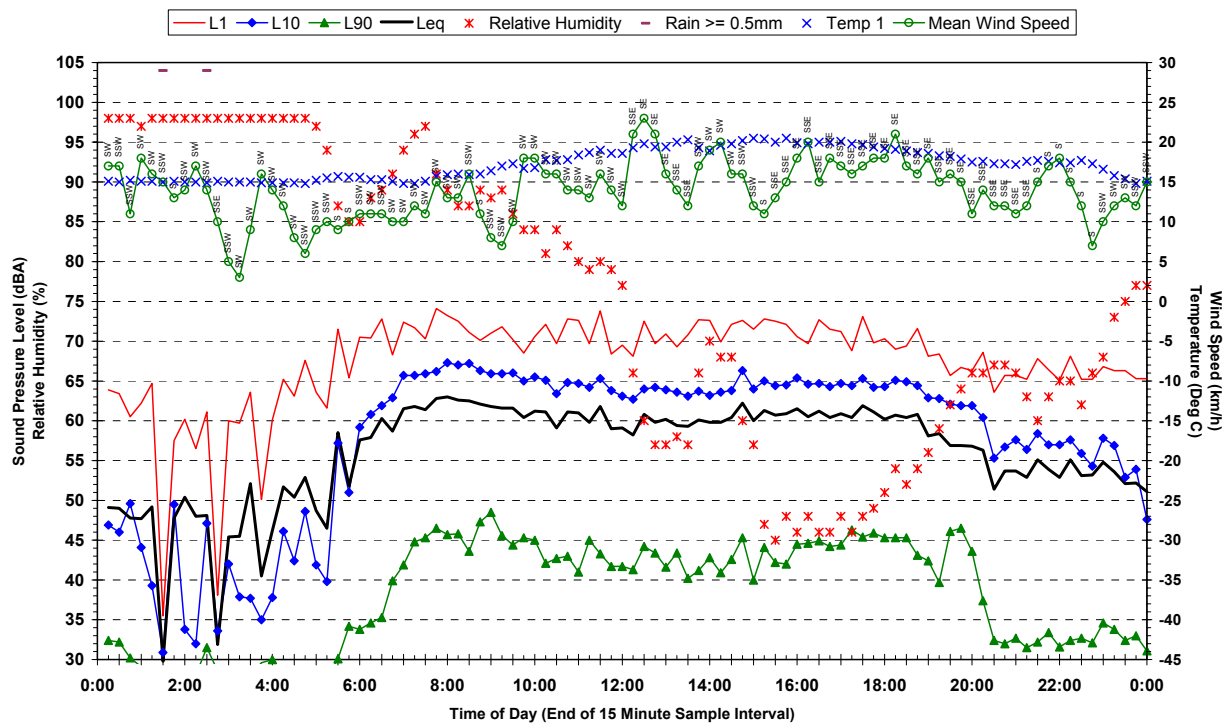
Statistical Ambient Noise Levels Corner Dulwich Road and Riverstone Parade, Vineyard - Monday 26 March 2007
