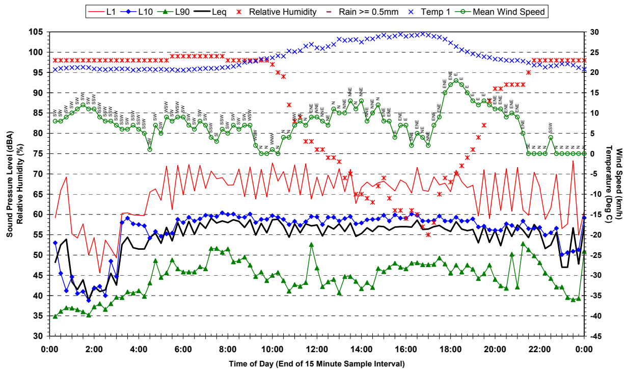
Statistical Ambient Noise Levels 128A Railway Terrace, Riverstone - Thursday 22 March 2007
