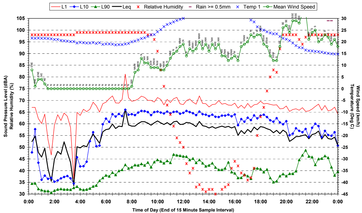
Statistical Ambient Noise Levels Corner Otago Street and Riverstone Parade, Vineyard - Saturday 24 March 2007
