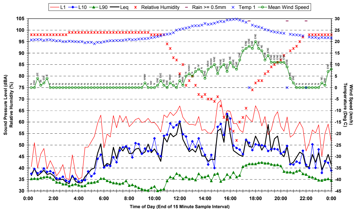
Statistical Ambient Noise Levels 63 Manorhouse Boulevard, Quakers Hill - Friday 23 March 2007
