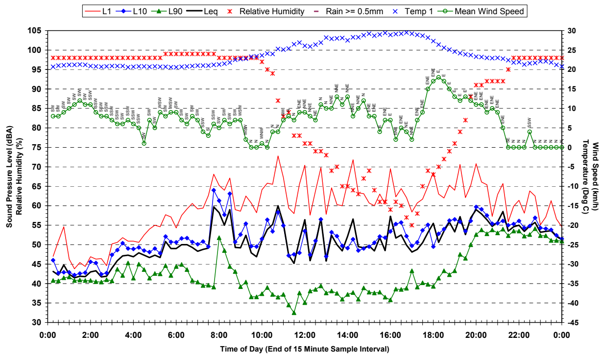
Statistical Ambient Noise Levels 51 Hunter Street, Riverstone - Thursday 22 March 2007
