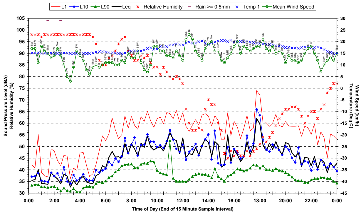
Statistical Ambient Noise Levels 63 Manorhouse Boulevard, Quakers Hill - Monday 26 March 2007
