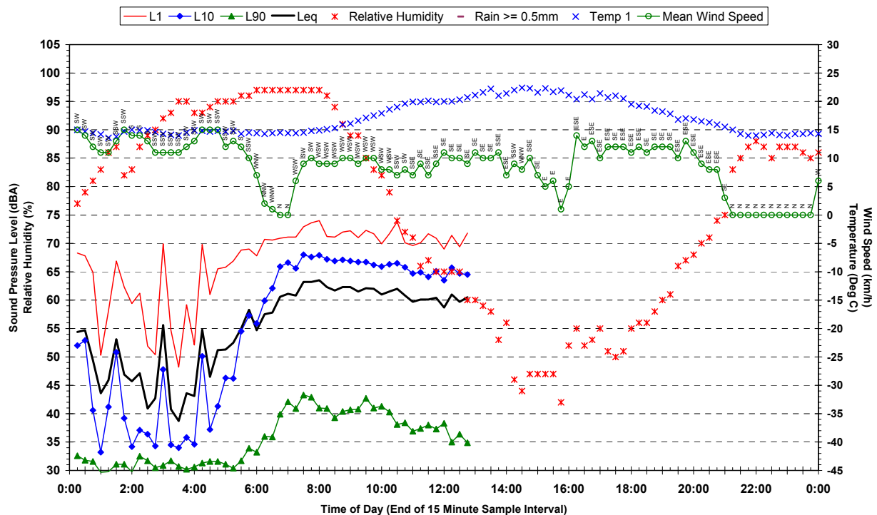
Statistical Ambient Noise Levels Corner Otago Street and Riverstone Parade, Vineyard - Tuesday 27 March 2007
