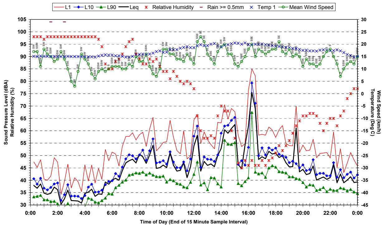
Statistical Ambient Noise Levels 155 Bridge Street, Schofields - Monday 26 March 2007
