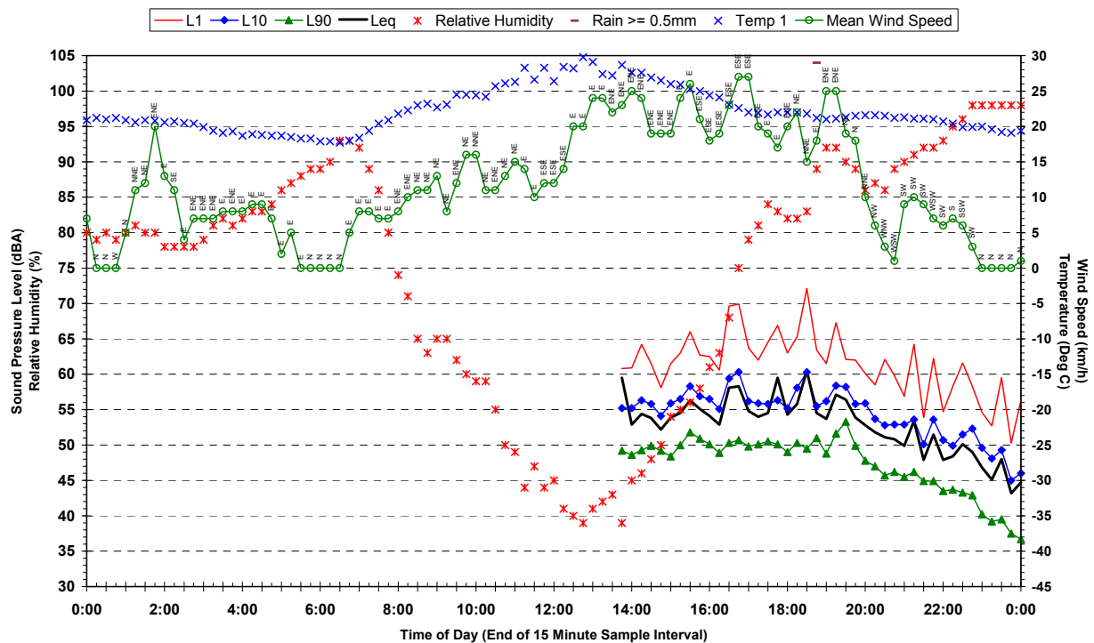
Statistical Ambient Noise Levels Kerry Jones Child Care Centre, Quakers Hill - Wednesday 7 February 2007
