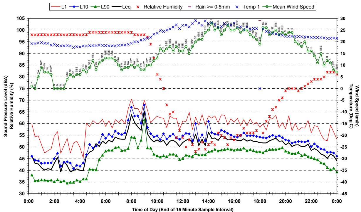
Statistical Ambient Noise Levels Kerry Jones Child Care Centre, Quakers Hill - Thursday 8 February 2007
