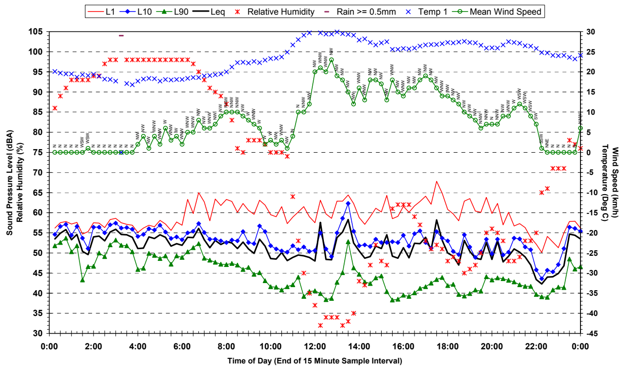
Statistical Ambient Noise Levels 51 Hunter Street, Riverstone - Friday 16 March 2007
