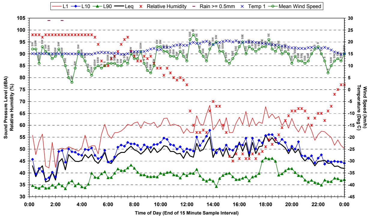
Statistical Ambient Noise Levels 51 Hunter Street, Riverstone - Monday 26 March 2007
