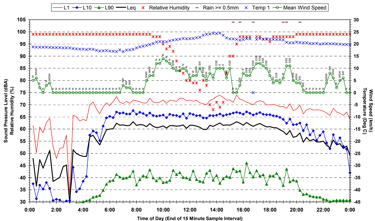
Statistical Ambient Noise Levels Corner Otago Street and Riverstone Parade, Vineyard - Monday 19 March 2007
