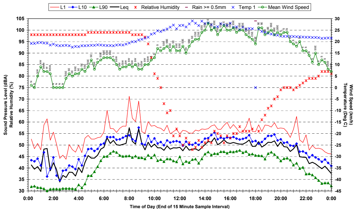
Statistical Ambient Noise Levels 3 Richards Avenue, Riverstone - Thursday 8 February 2007
