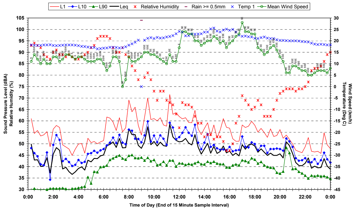
Statistical Ambient Noise Levels 3 Richards Avenue, Riverstone - Tuesday 13 February 2007
