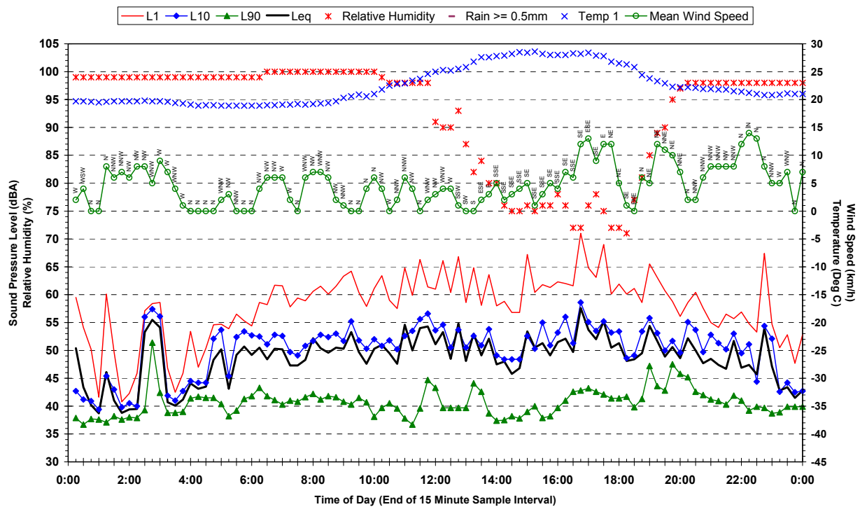
Statistical Ambient Noise Levels 51 Hunter Street, Riverstone - Tuesday 20 March 2007
