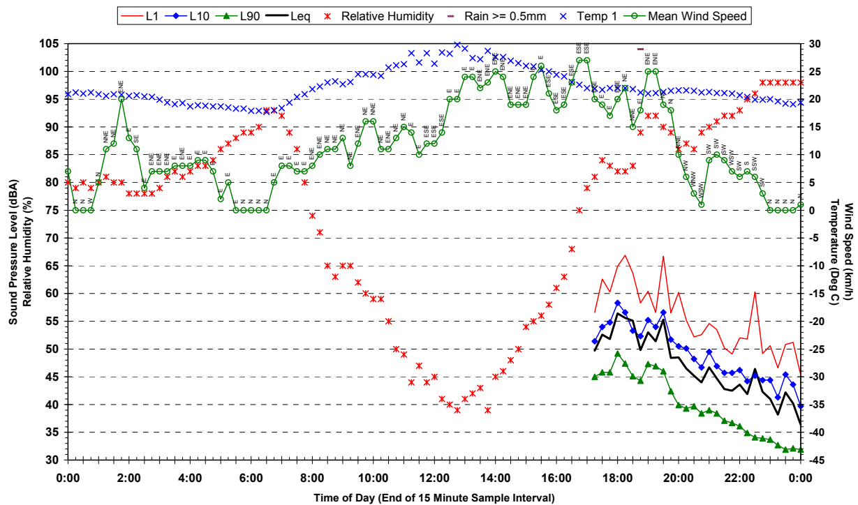
Statistical Ambient Noise Levels 3 Richards Avenue, Riverstone - Wednesday 7 February 2007
