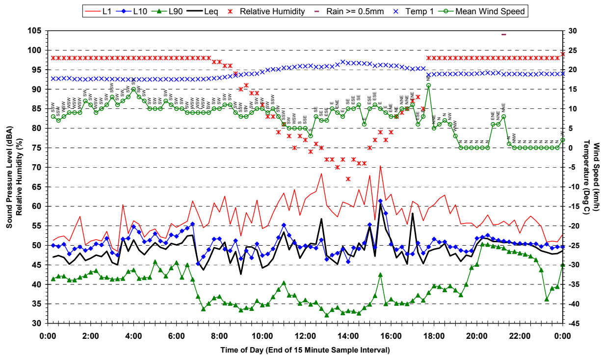
Statistical Ambient Noise Levels 51 Hunter Street, Riverstone - Sunday 18 March 2007
