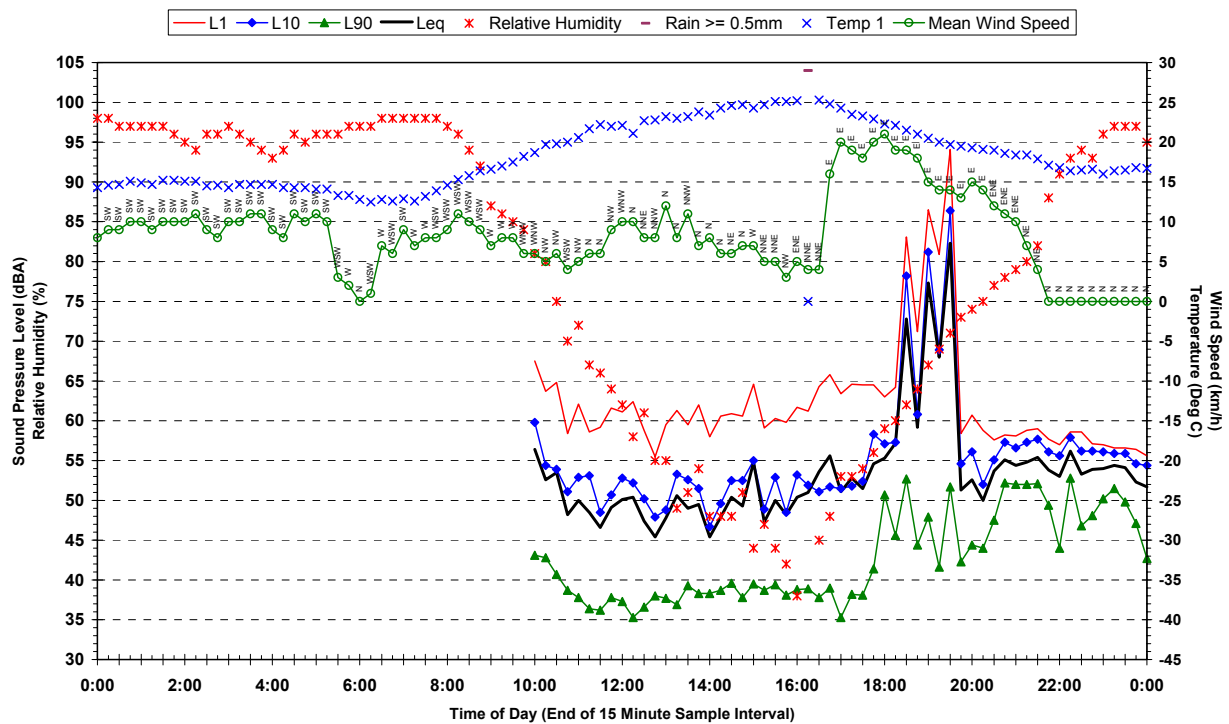
Statistical Ambient Noise Levels 51 Hunter Street, Riverstone - Wednesday 14 March 2007
