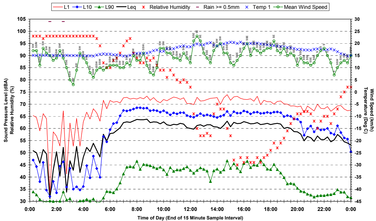
Statistical Ambient Noise Levels Corner Otago Street and Riverstone Parade, Vineyard - Monday 26 March 2007
