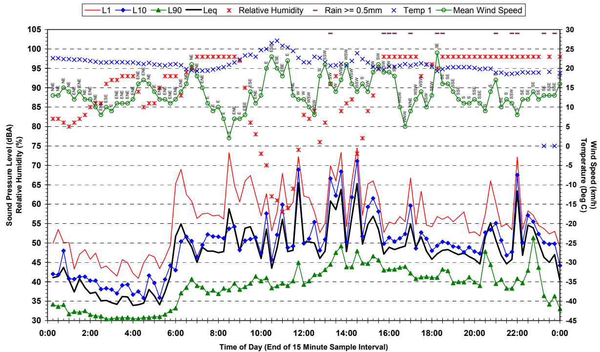
Statistical Ambient Noise Levels 3 Richards Avenue, Riverstone - Sunday 11 February 2007
