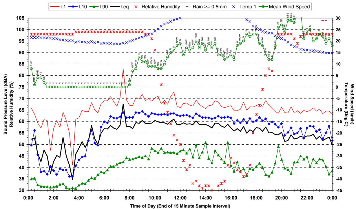
Statistical Ambient Noise Levels Corner Dulwich Road and Riverstone Parade, Vineyard - Saturday 24 March 2007
