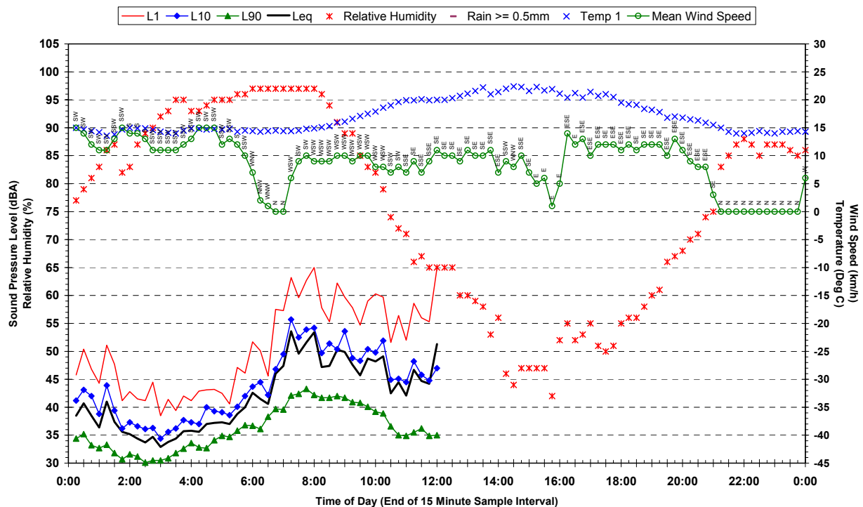
Statistical Ambient Noise Levels 155 Bridge Street, Schofields - Tuesday 27 March 2007
