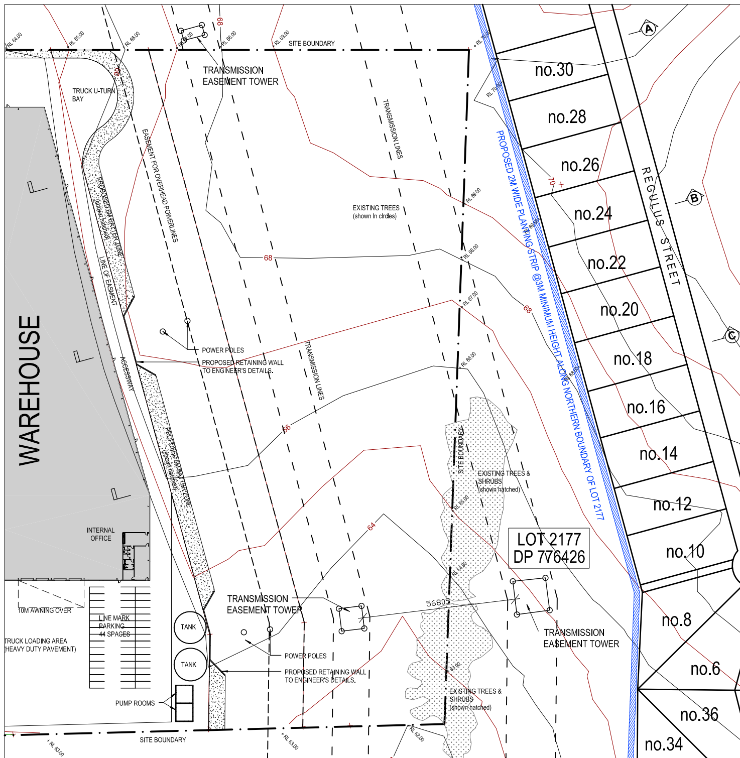
landscape strip location plan
