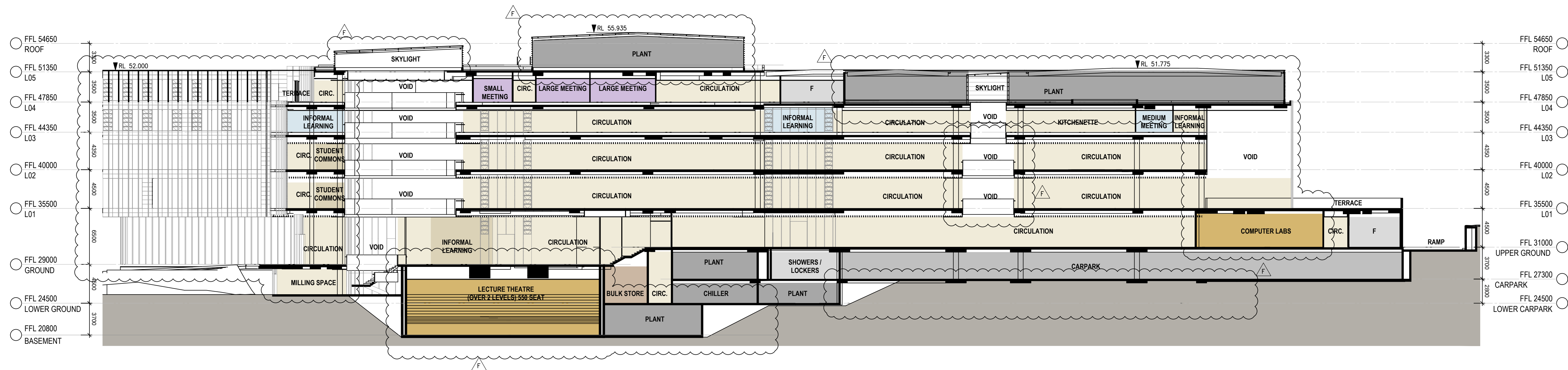
D SECTION D 1:250@A1
