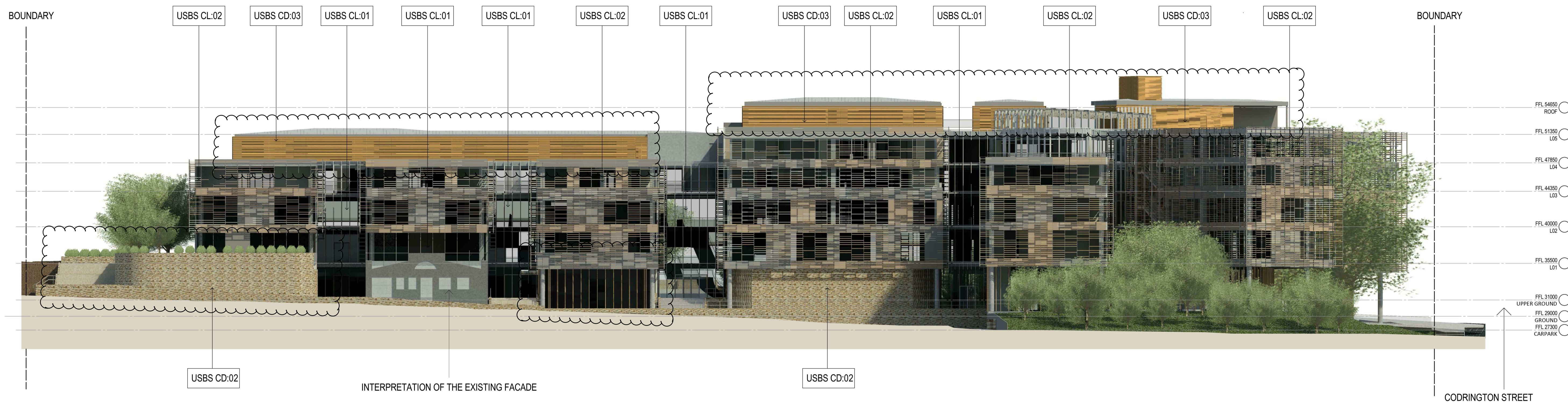
1 ABERCROMBIE STREET ELEVATION buildings infront removed 1:250 @ A1
