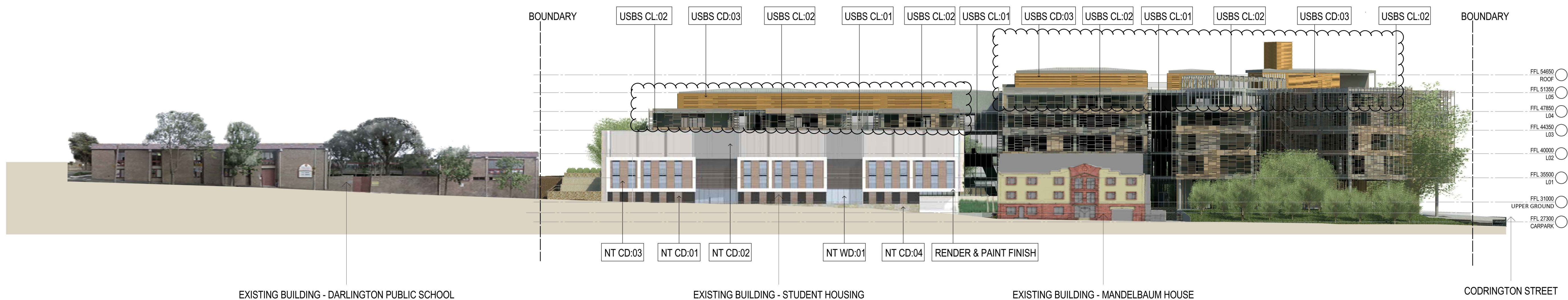
2 ABERCROMBIE STREET ELEVATION with context 1:400 @ A1
