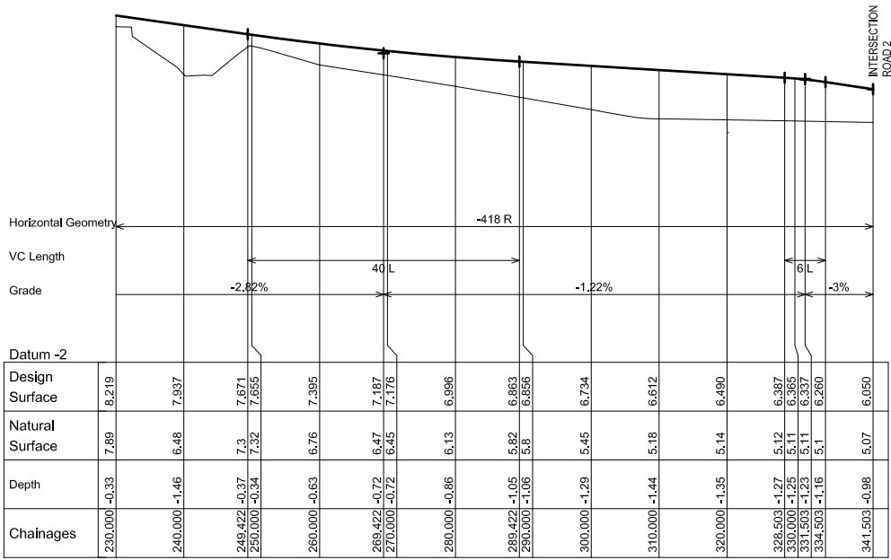
LONGITUDINAL SECTION - ROSEDALE AVENUE
