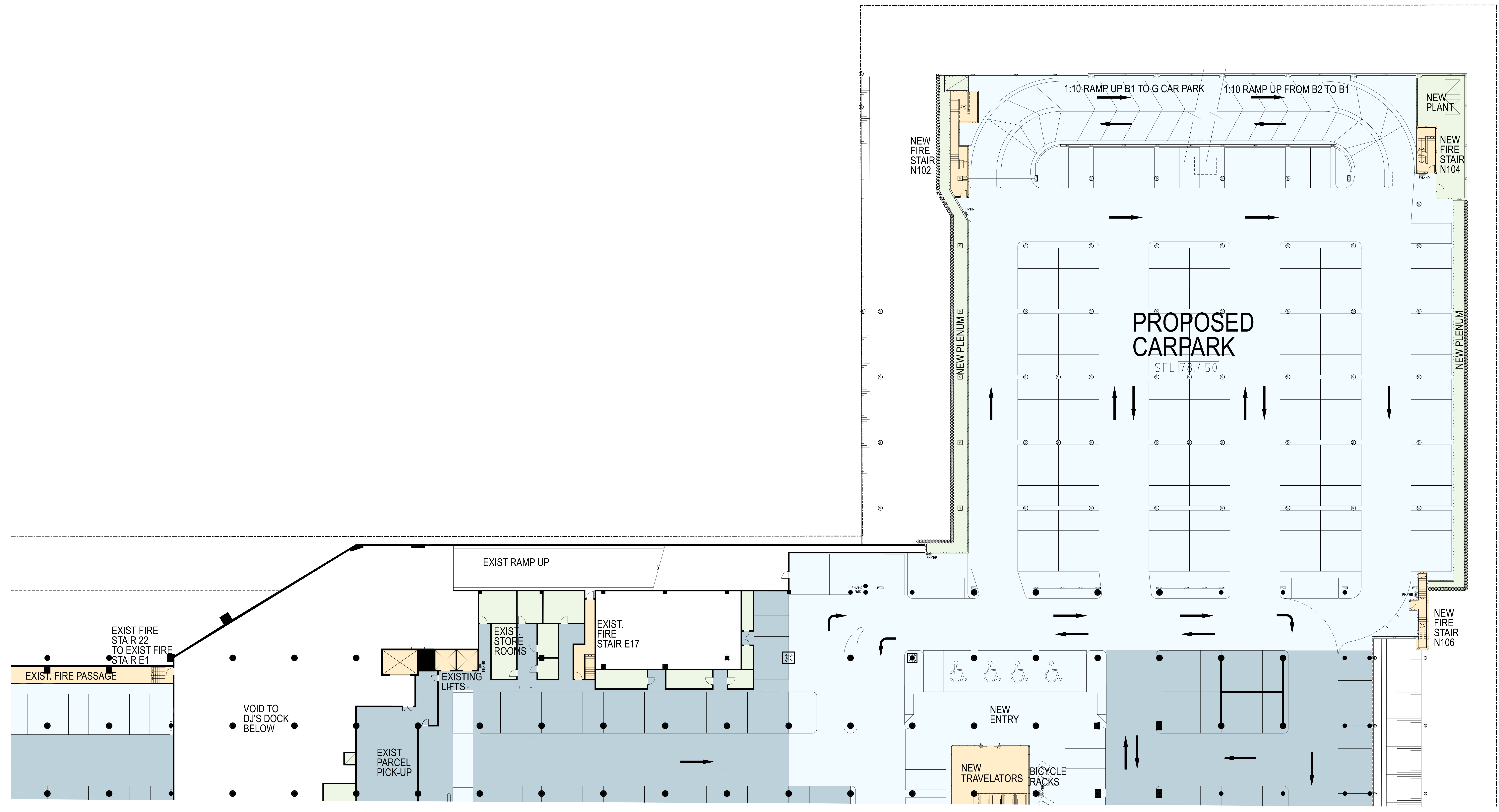
BASEMENT LEVEL 1
