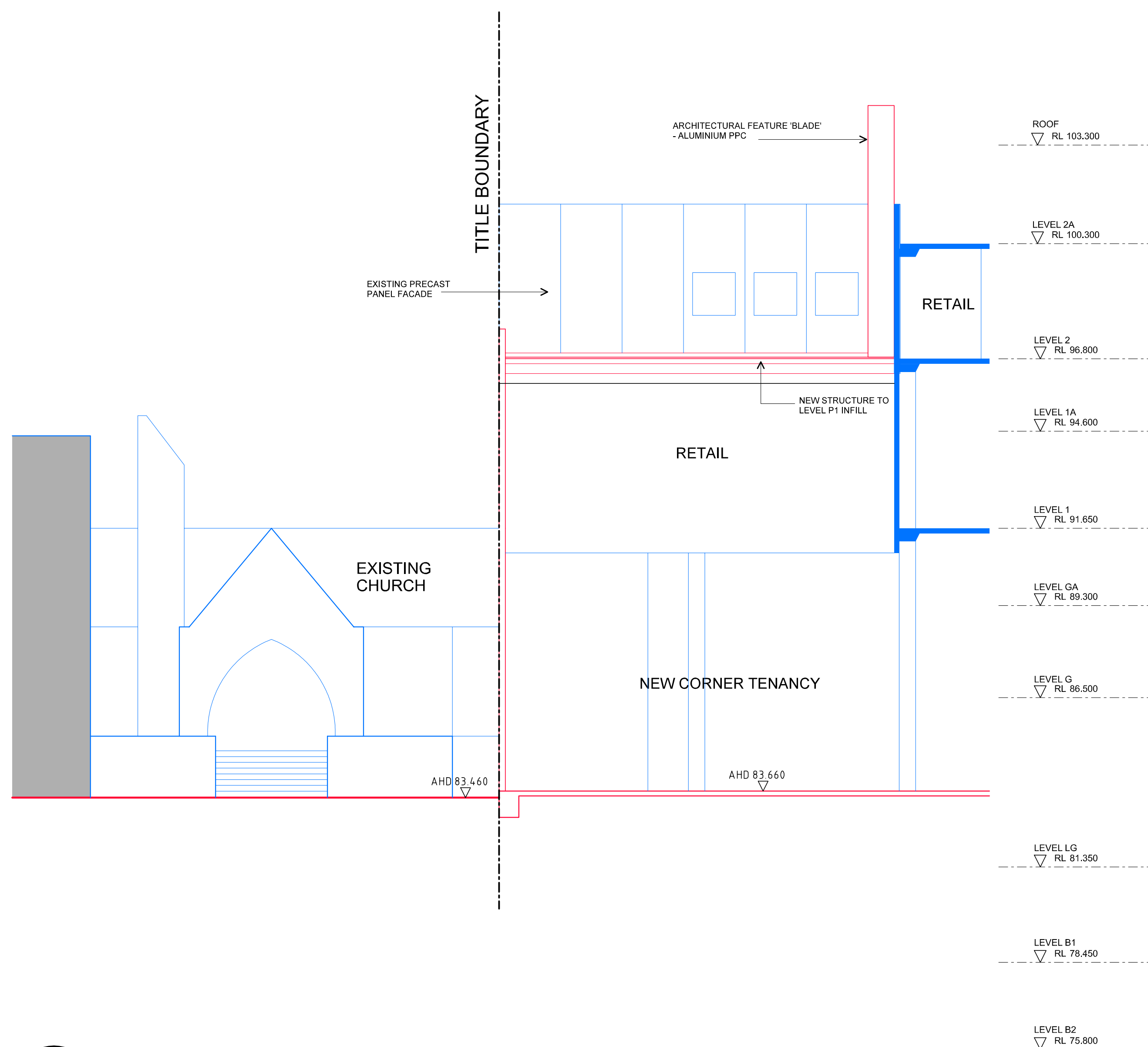
05 SECTION - NEW RETAIL TENANCY SCALE 1:100 VICTORIA AVENUE
