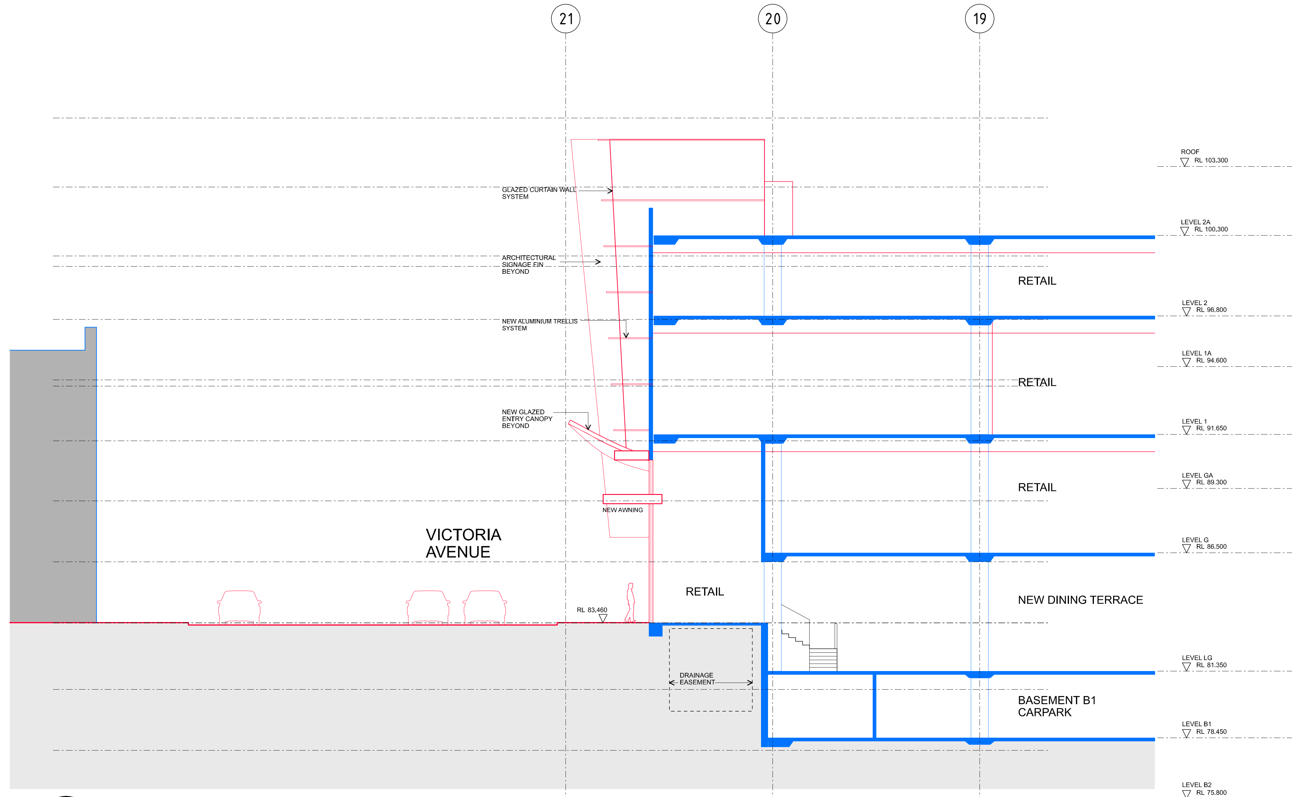
06 SECTION - NEW RETAIL TENANCY SCALE 1:100 VICTORIA AVENUE
