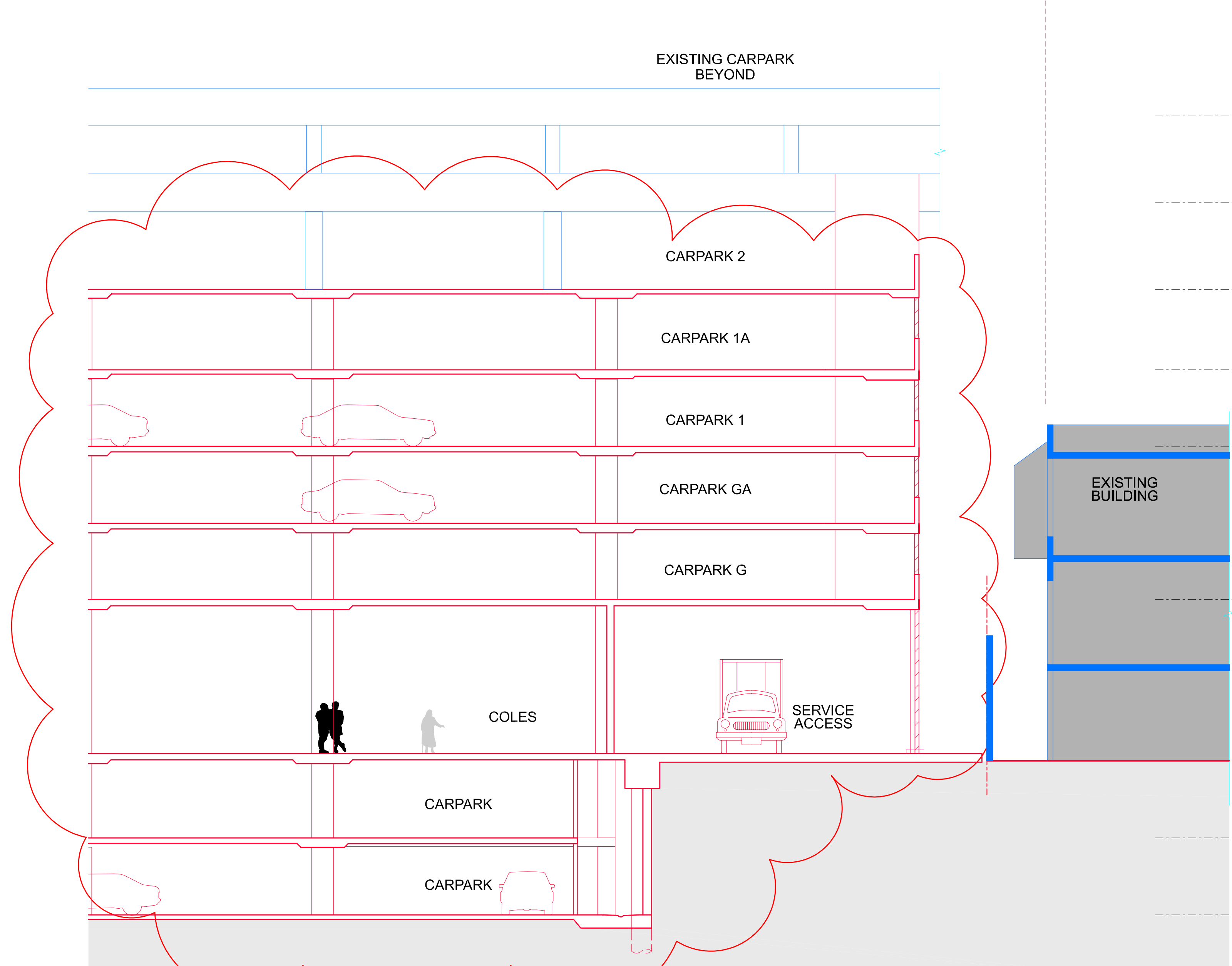
04 SECTION - COLES AT MALVERN AVE. LOADING ENTRY SCALE 1:100 MALVERN AVENUE
