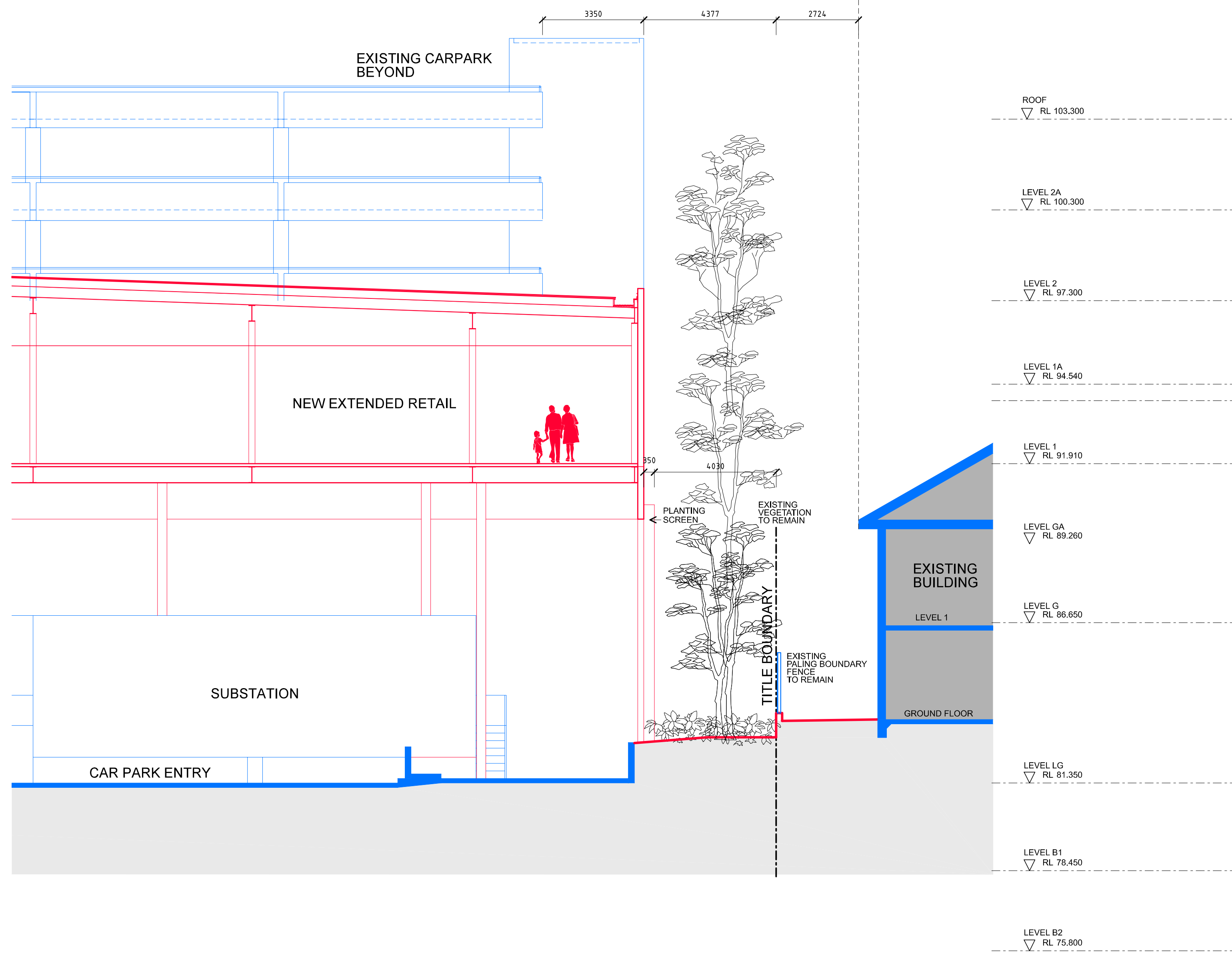
03 SECTION - RETAIL EXTENSION OF EXISTING CARPARK DECKS SCALE 1:100 HAYILAH STREET
