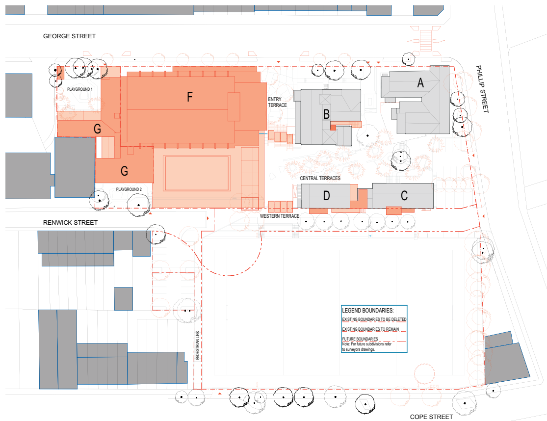
SITE PLAN
