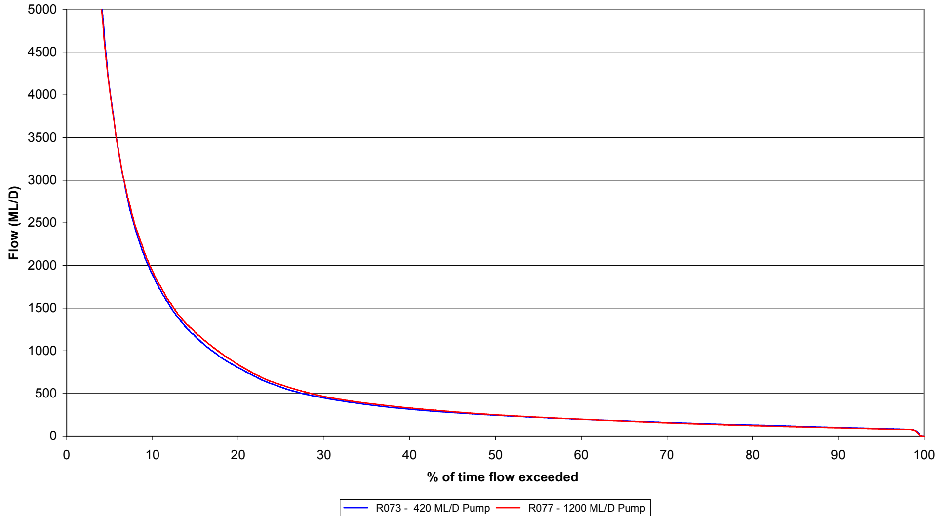
Flow Duration Curve - Downstream of Macquarie Generation Pump Site
