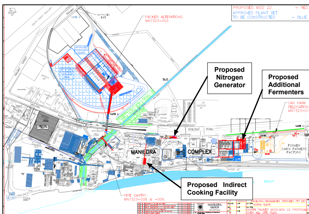
Figure 7: Location of Proposed Nitrogen Generator and Storage Tanks and Indirect Cooking Facility.
