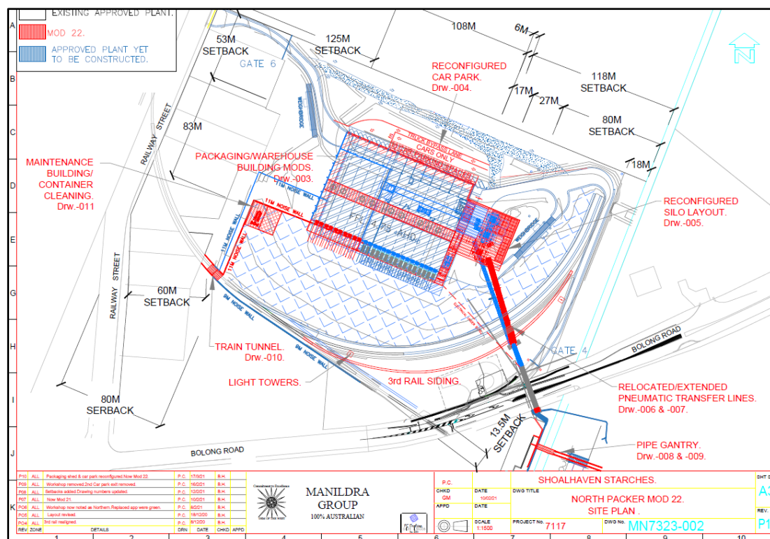
Figure 5: Site Plan – Packing Plant Modifications.
