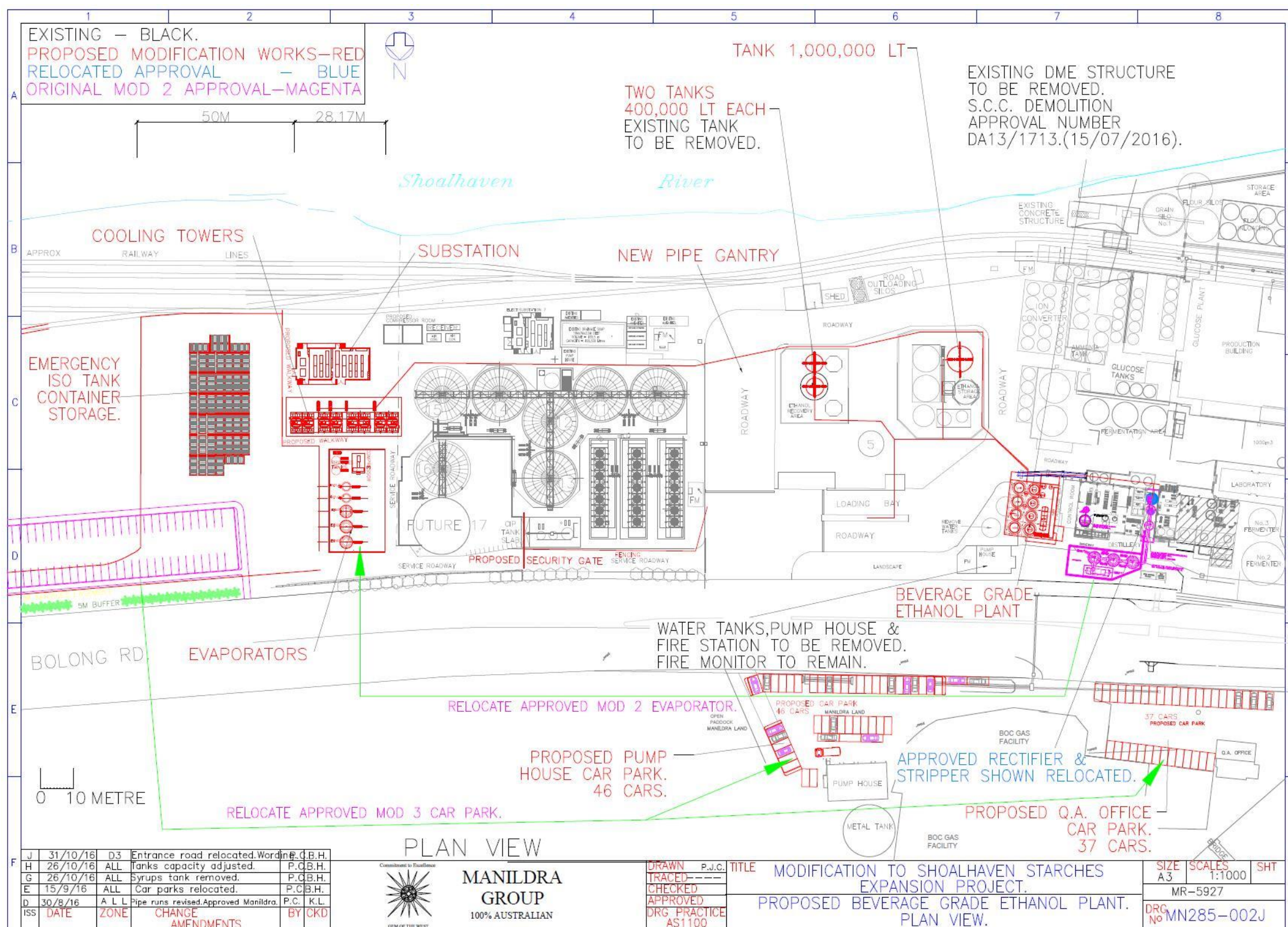
Figure 3 – Site Layout – Ethanol Area
