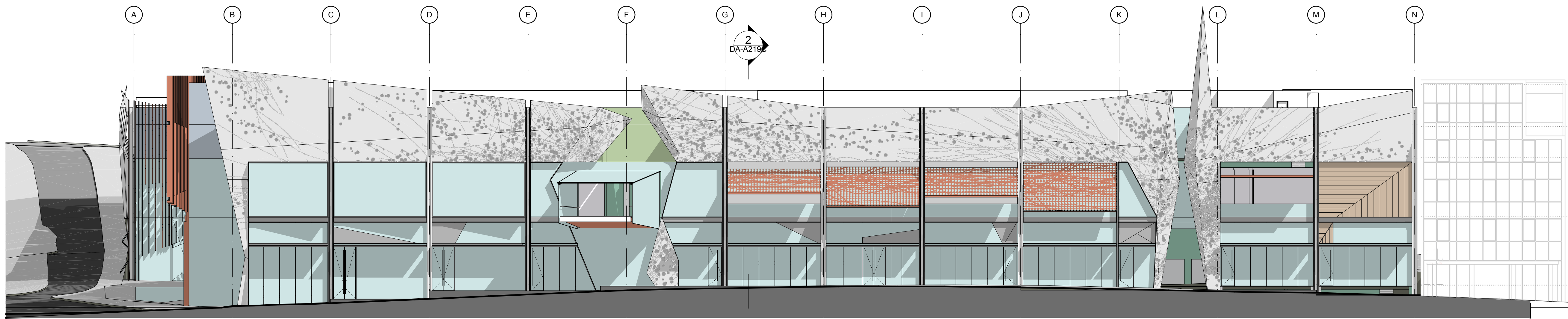
1 ELEVATION KEIRA STREET 1:200 @B1
