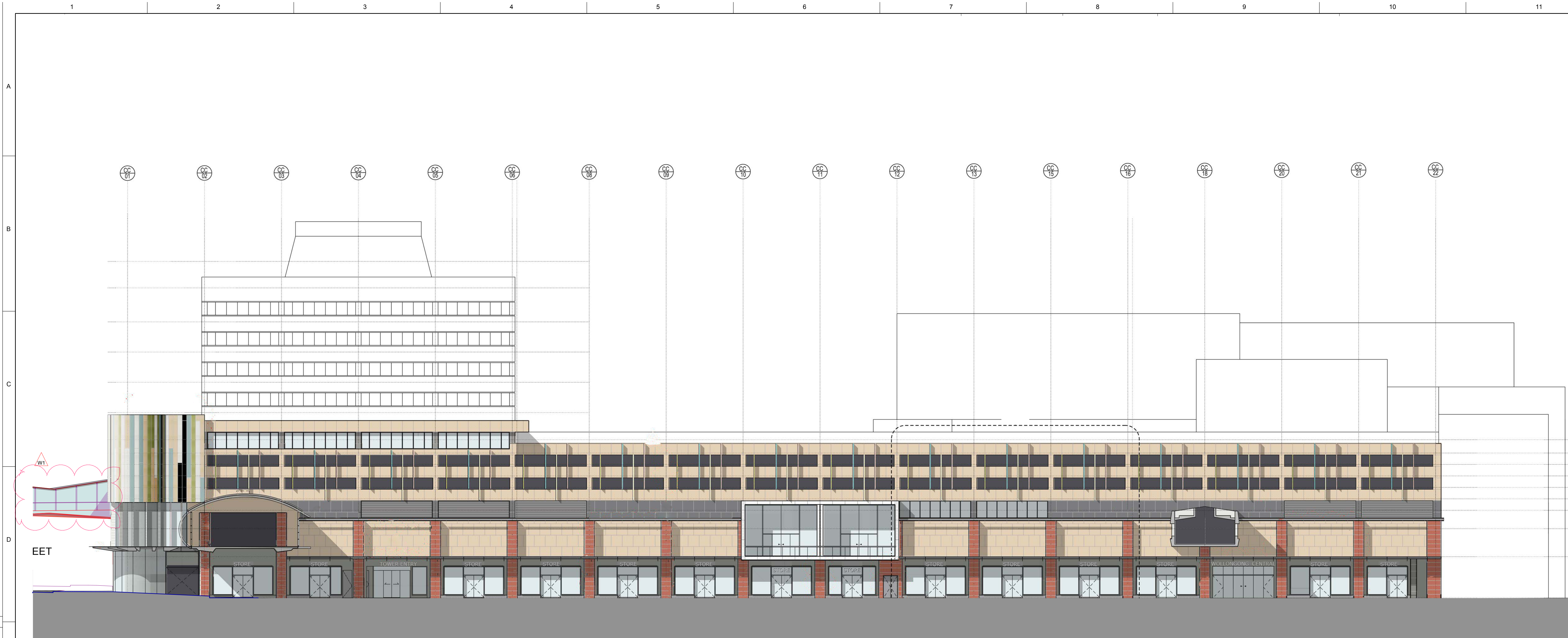
1 ELEVATION CROWN STREET MALL ELEVATION 1:200 @B1
