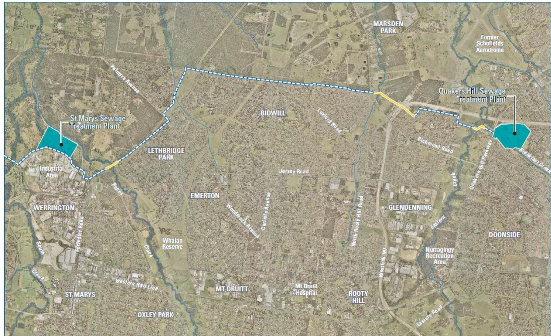
Figure 3.5b Pipeline route - St Marys to Quakers Hill
