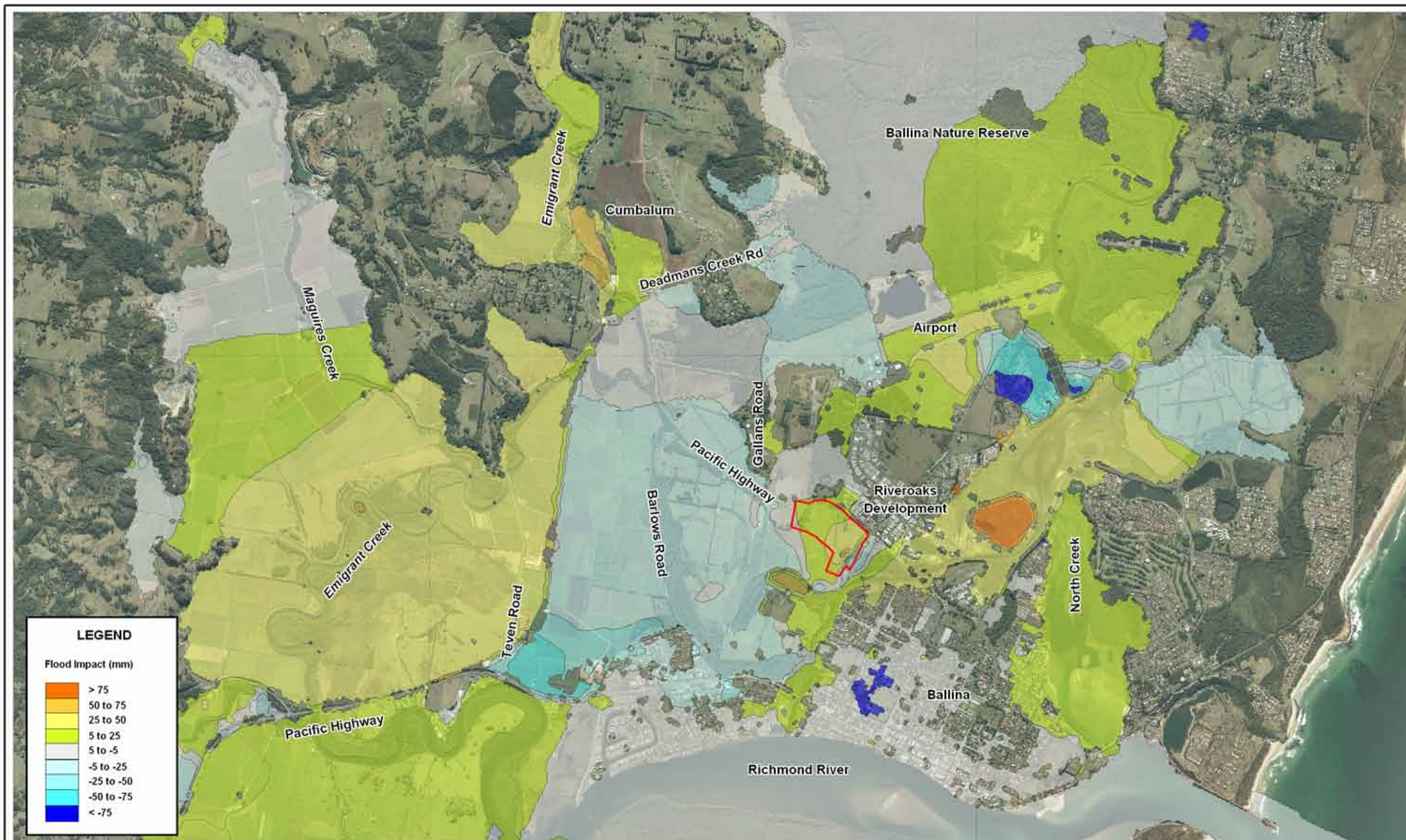
Title: Riveroaks Pre-Development Peak Flood Impacts 100 Year ARI Combined Event
