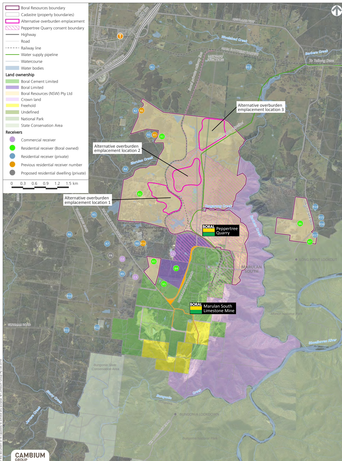
Figure 11a. Alternative overburden emplacement locations (provided by Element Environment)
