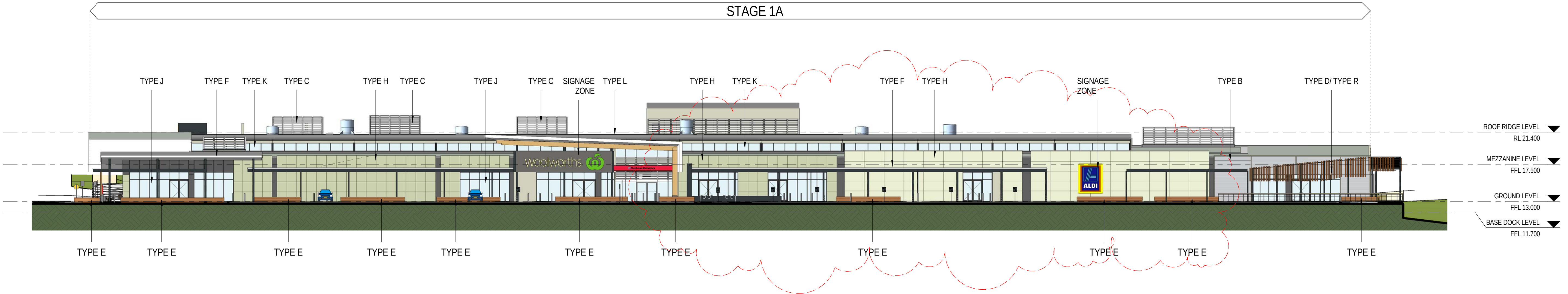
2 ELEVATION EAST ELEVATION
