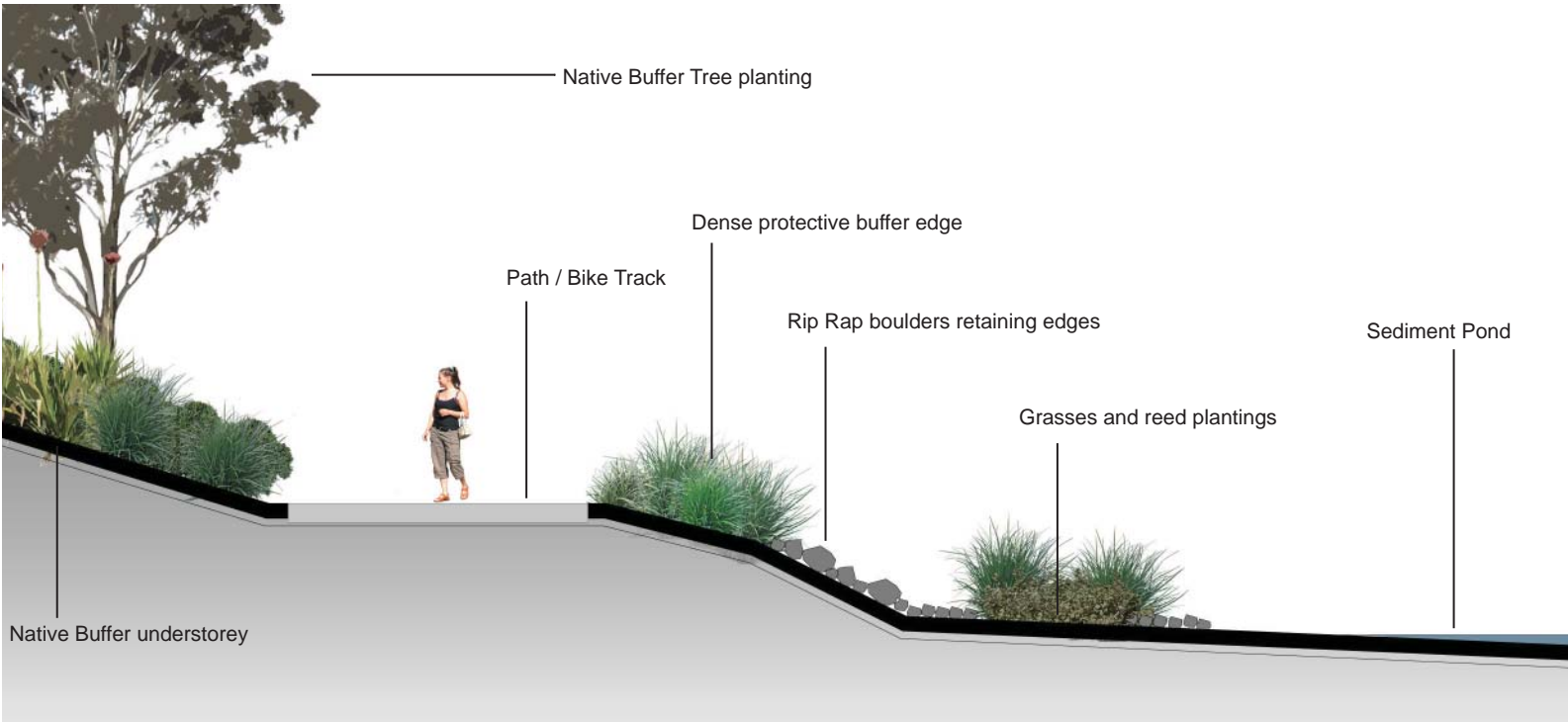
D. INDICATIVE SECTION THROUGH THE WATERFRONT TERRACES - NTS
