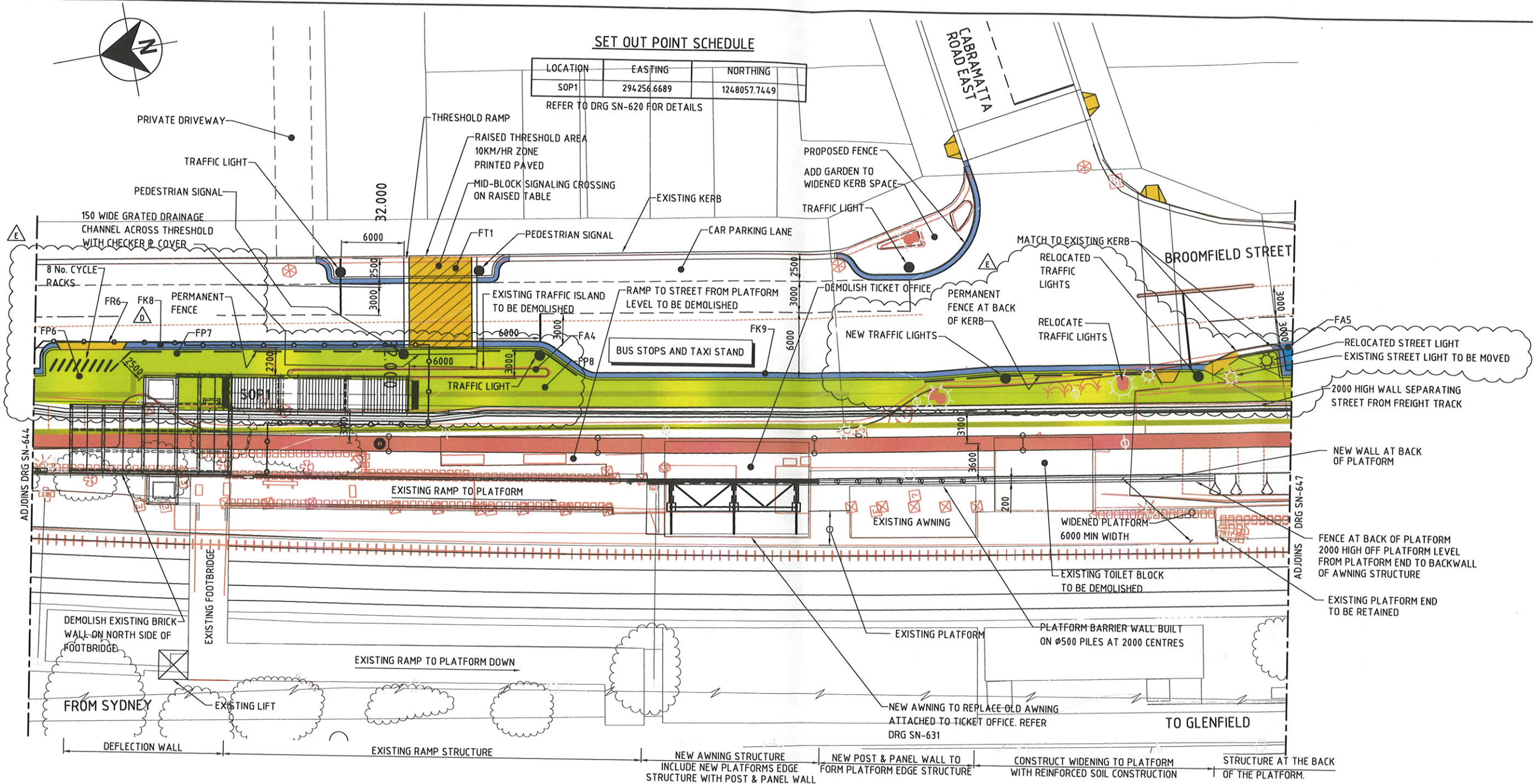
CABRAMATTA STATION SURFACE PLAN 1:200
