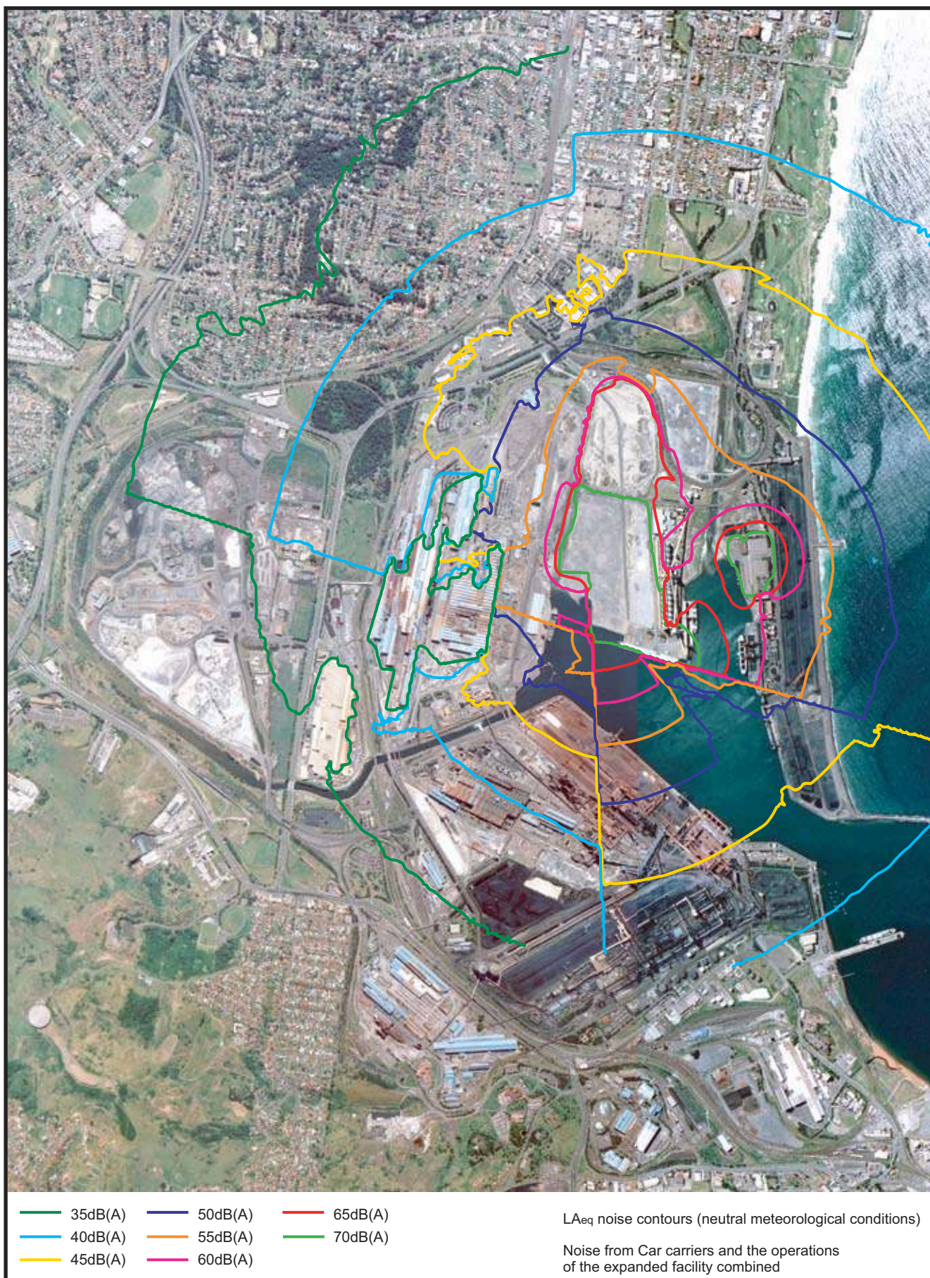
Figure 4.6b NOISE EMISSION CONTOURS
