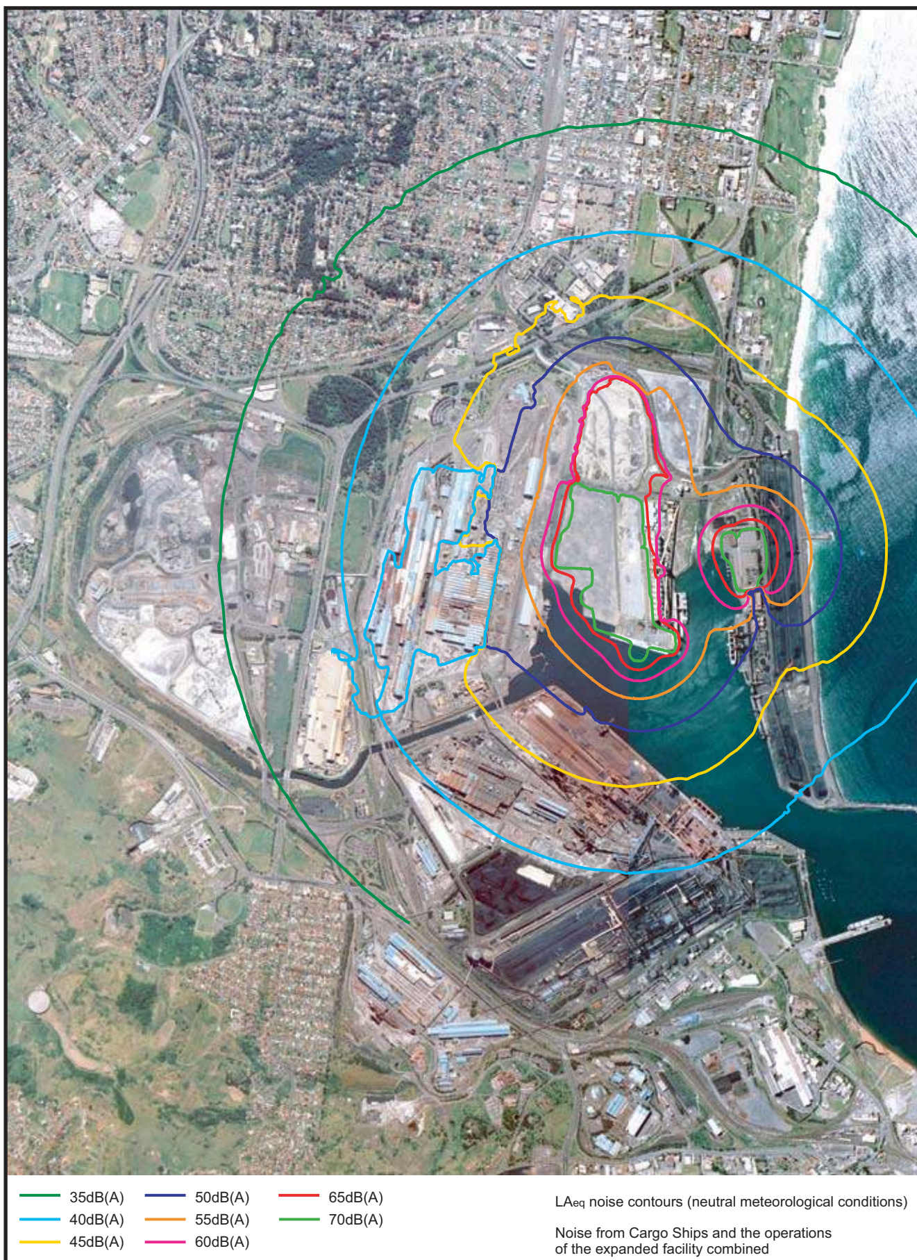
Figure 4.6a NOISE EMISSION CONTOURS
