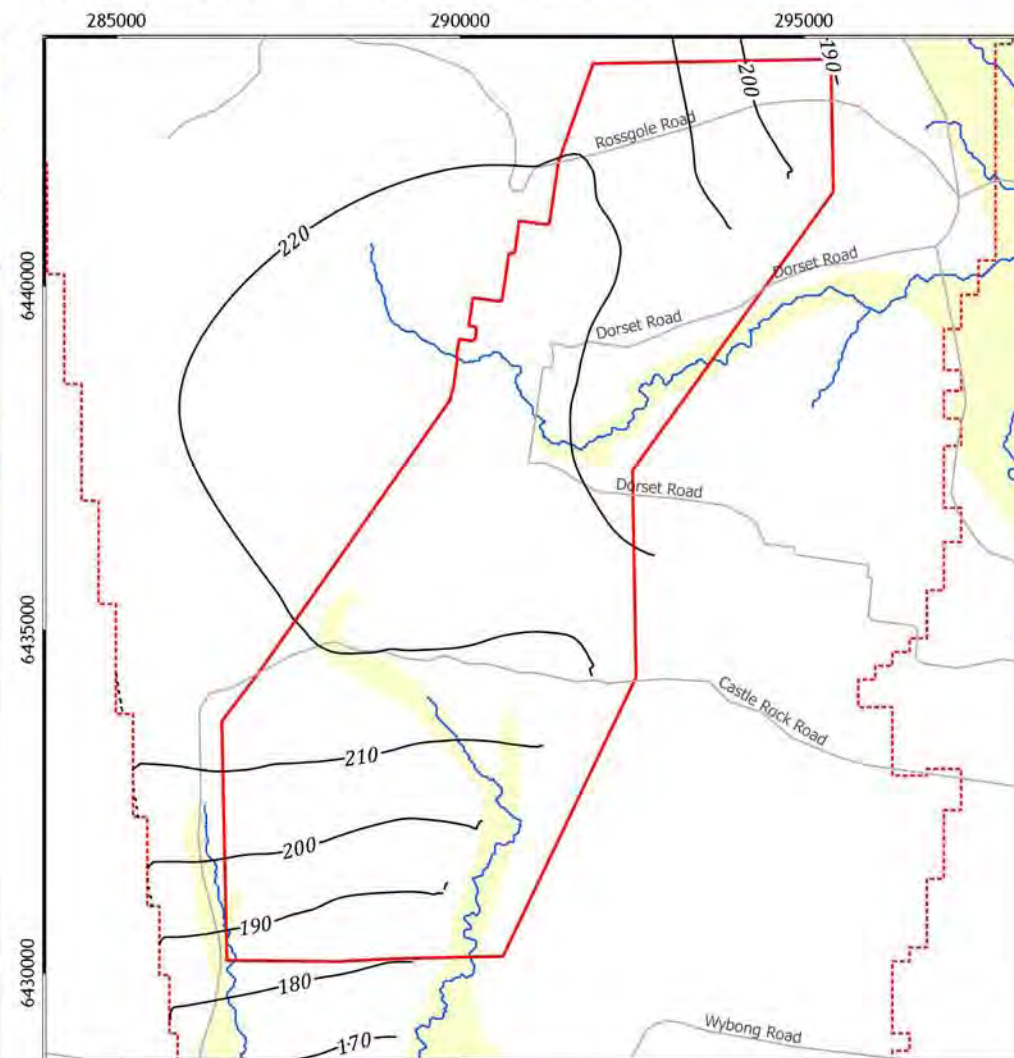
Hydraulic head - L09 - Permian coal seam (Blakefield)
