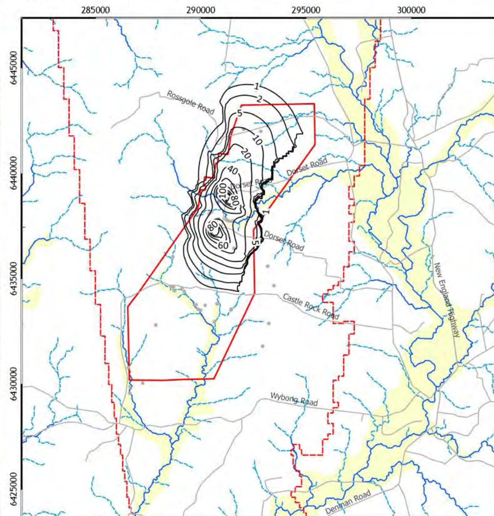
Drawdown Y10 - Permian coal seams (L09)
