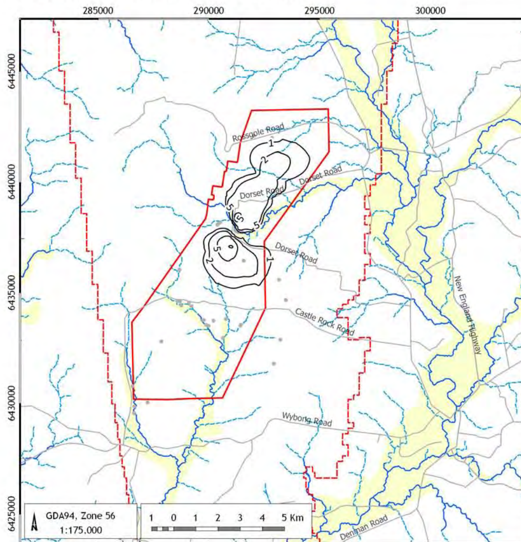
Drawdown Y10 - alluvium/weathered regolith (L02)
