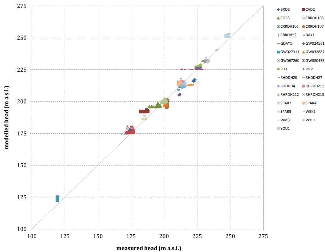
Figure C 15 Scatter diagram – ‘transient trends’ dataset – selected bores
