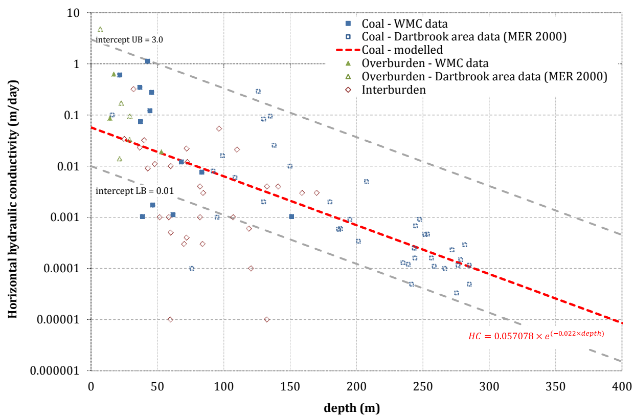
Figure C 8 Change of hydraulic conductivity with depth – field and model data
