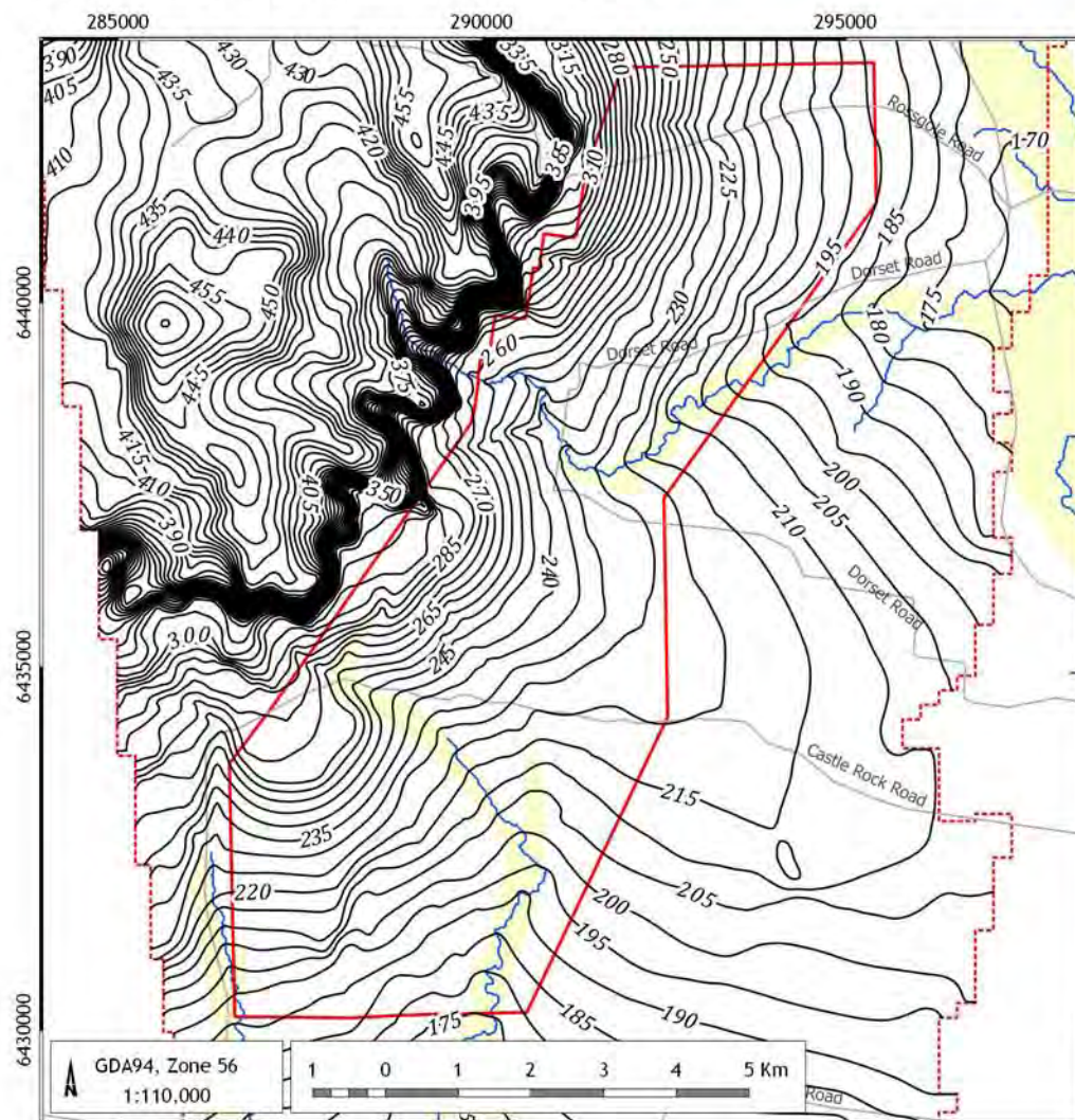
Hydraulic head - L01 - weathered regolith, alluvium
