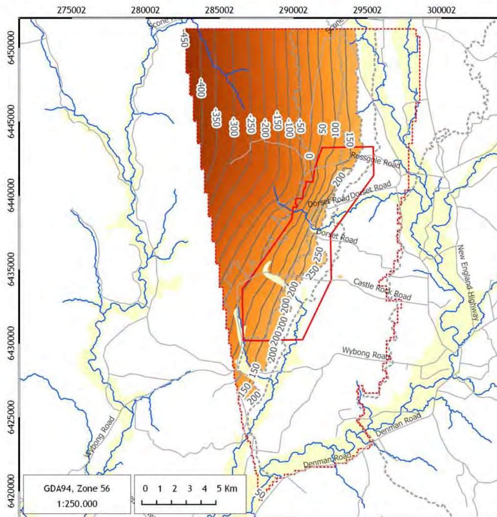
Base of Layer 7 - Wambo
