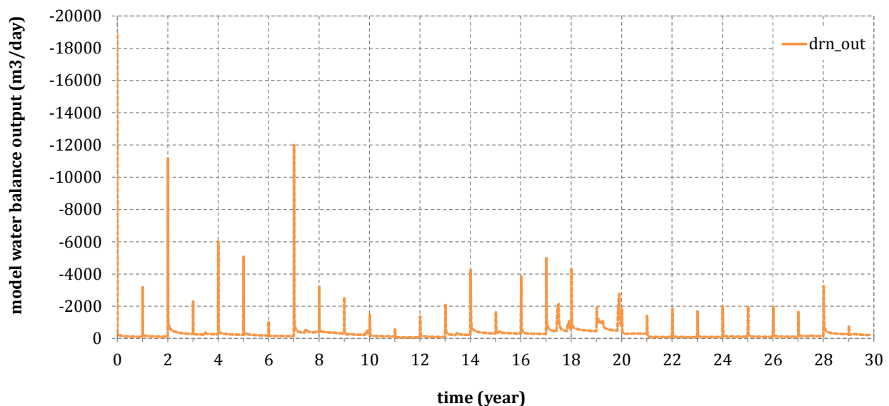
Figure C 21 Model water balance output – DRN boundary condition
