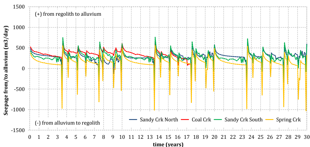
Figure C 23 Transient flow rates for alluvial zones
