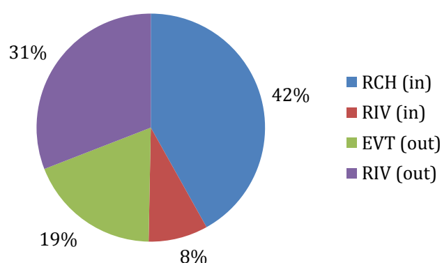
Figure C 11 Water budget overview – representation of individual boundary conditions
