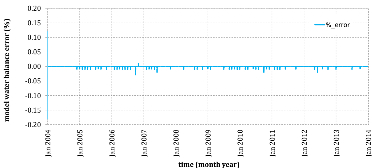
Figure C 10 The water balance error for the calibration period
