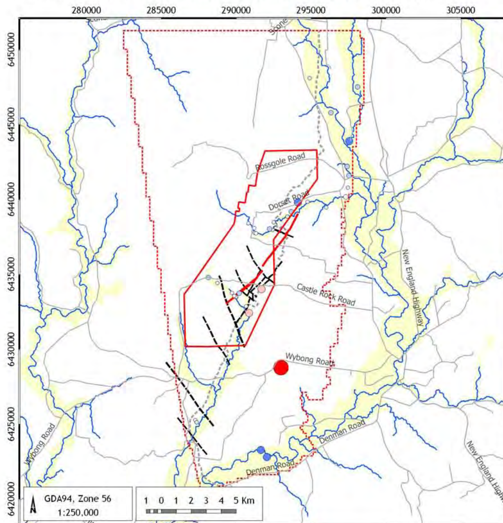
Residuals - 'starting heads' dataset - L01-02 - weathered regolith, alluvium
