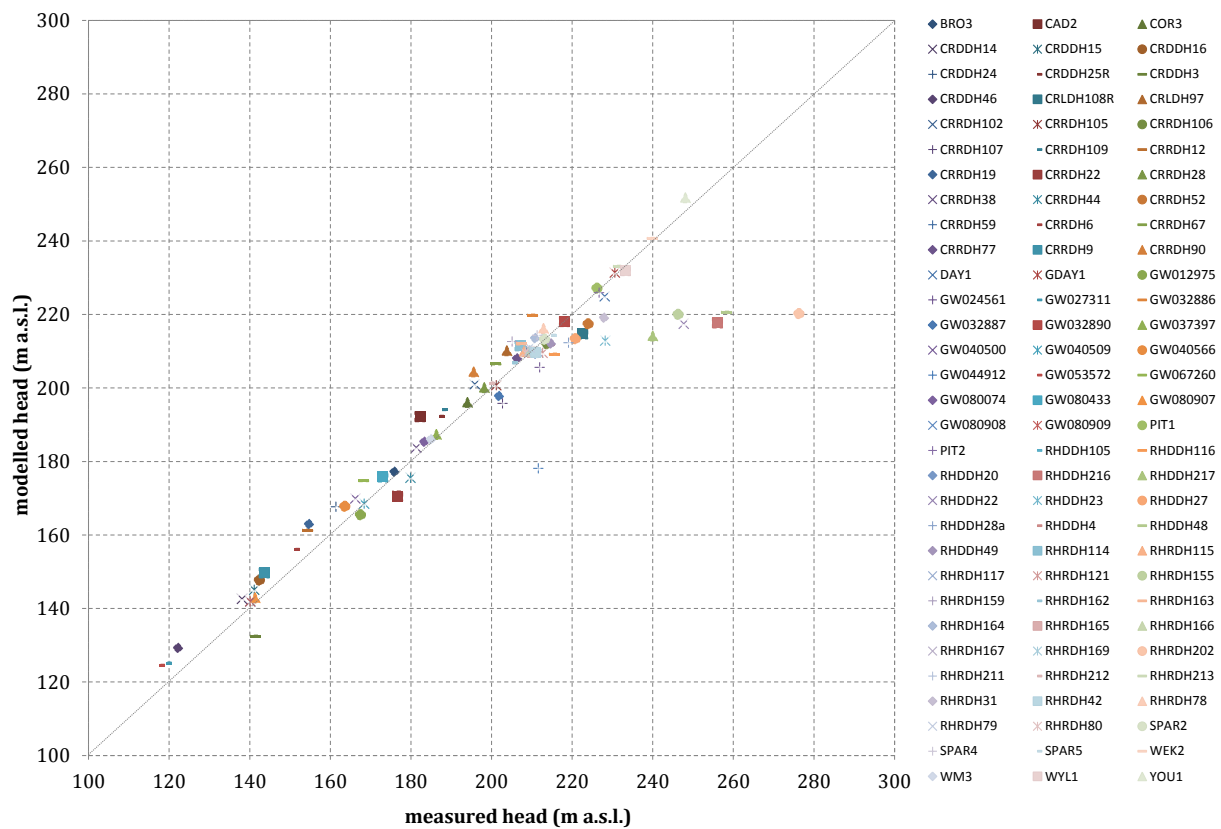
Figure C 12 Scatter diagram – ‘starting heads’ dataset – all bores
