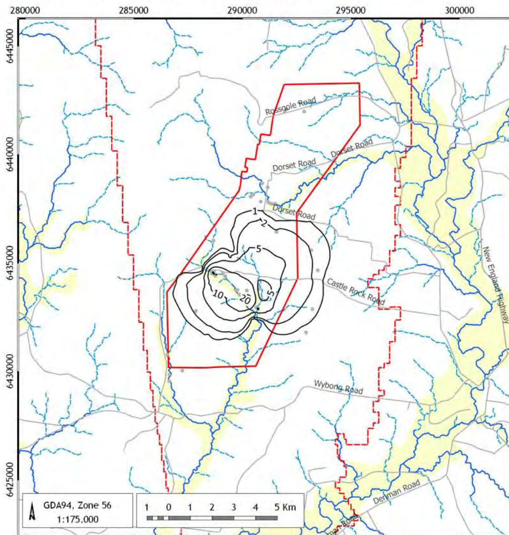
Drawdown Y20 - alluvium/weathered regolith (L02)
