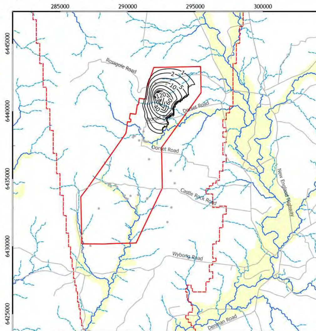
Drawdown Y03 - Permian coal seams (L09)
