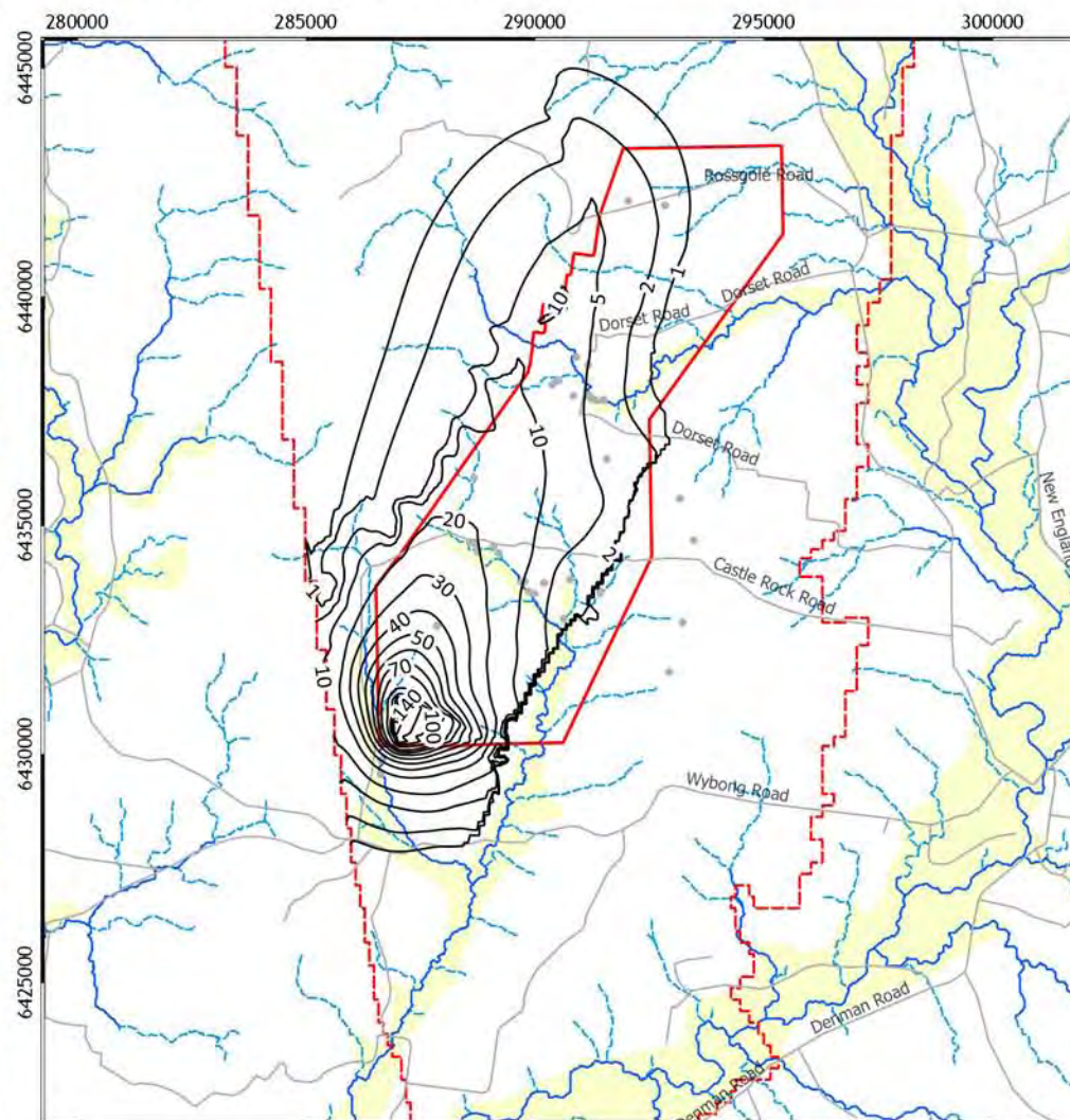
Drawdown Y30 - Permian coal seams (L09)
