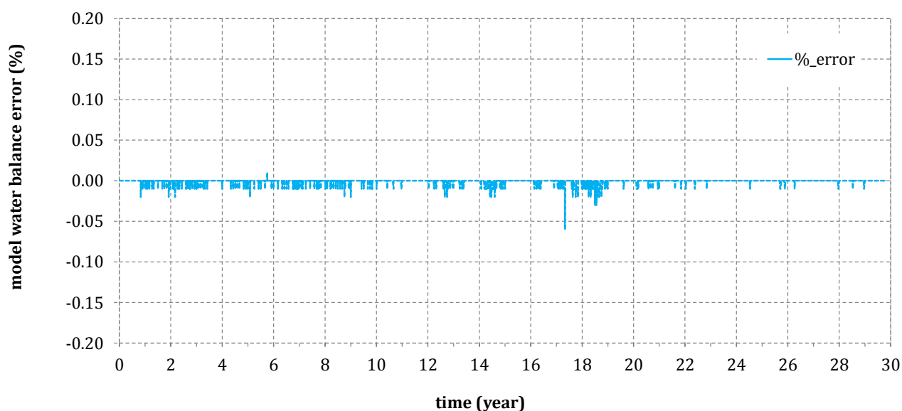
Figure C 19 The water balance error for the prediction (mining) period
