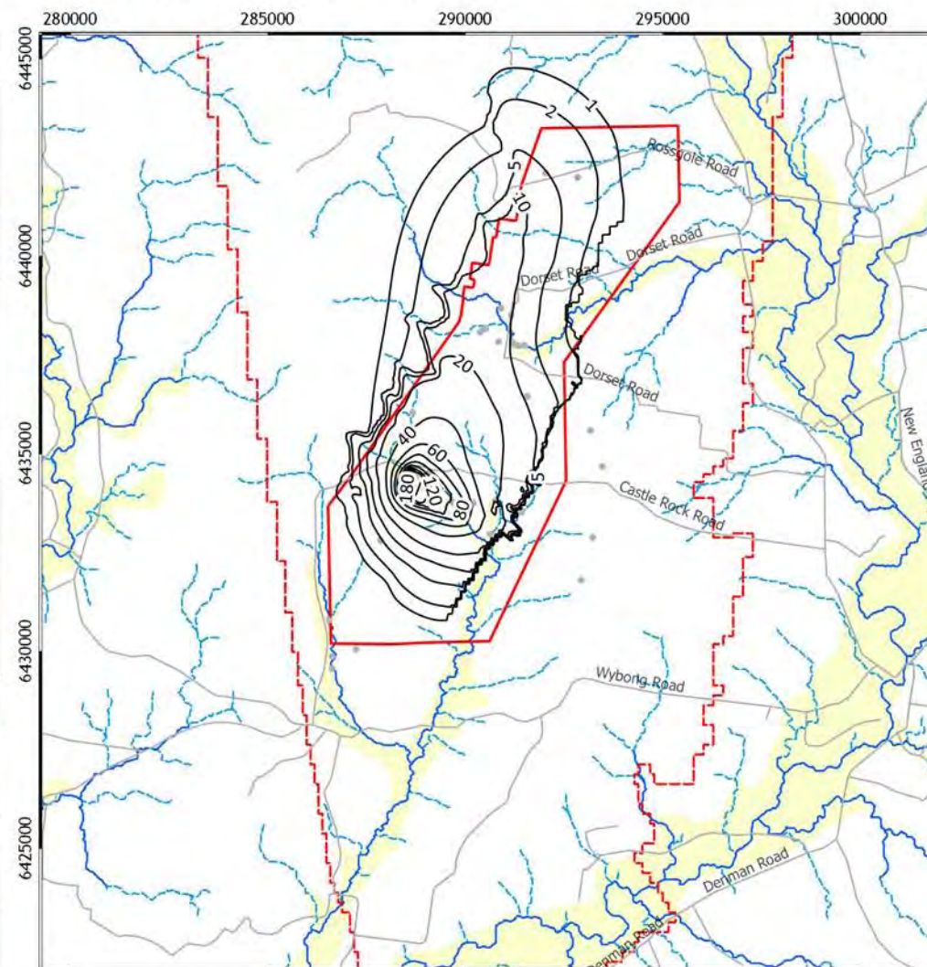
Drawdown Y20 - Permian coal seams (L09)
