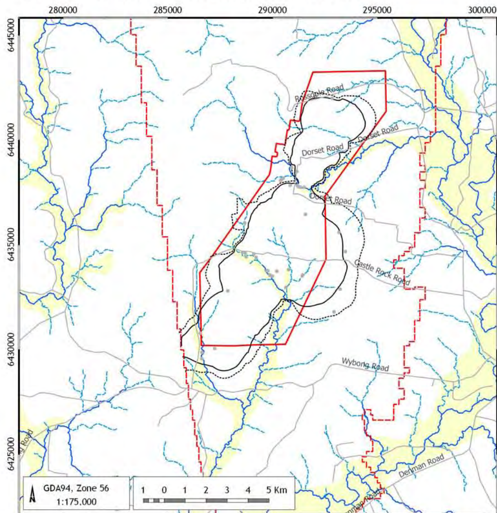
Cumulative drawdown - alluvium/weathered regolith (L01-02)
