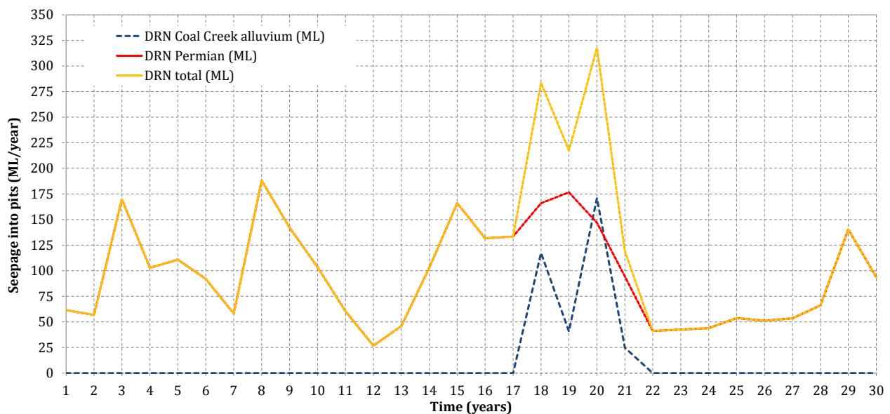
Figure C 22 DRN boundary condition – summary annual output
