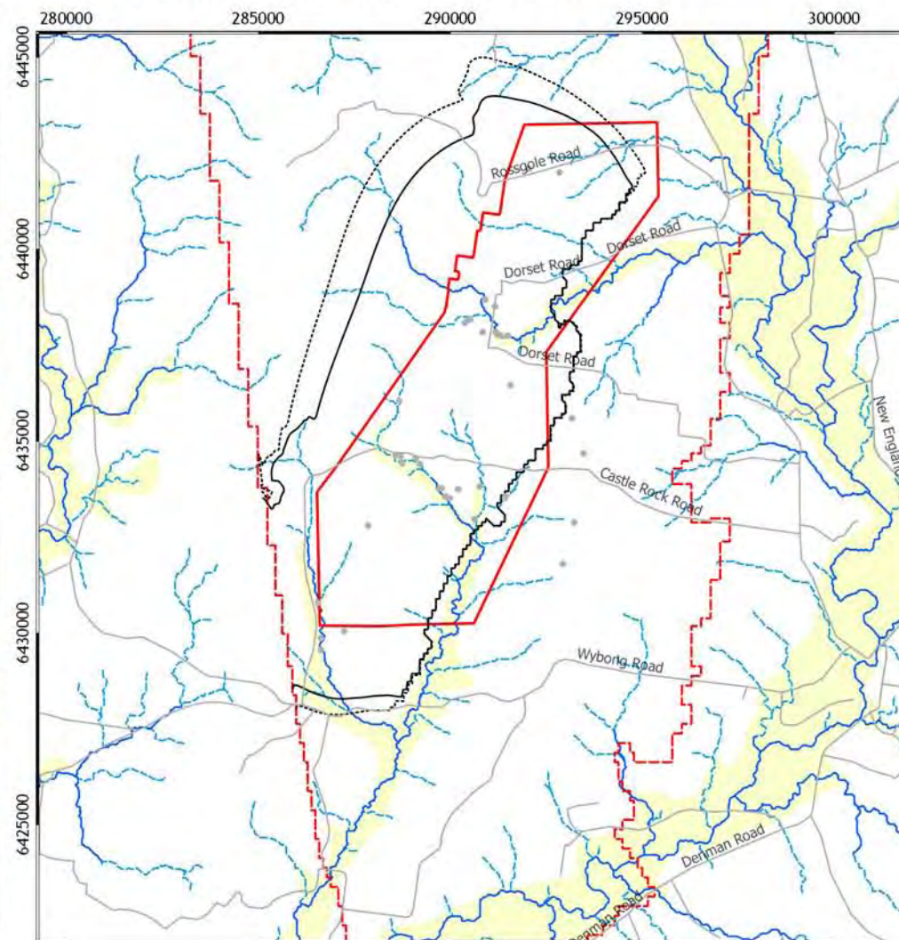
Cumulative drawdown - Permian coal seams (L05-11)
