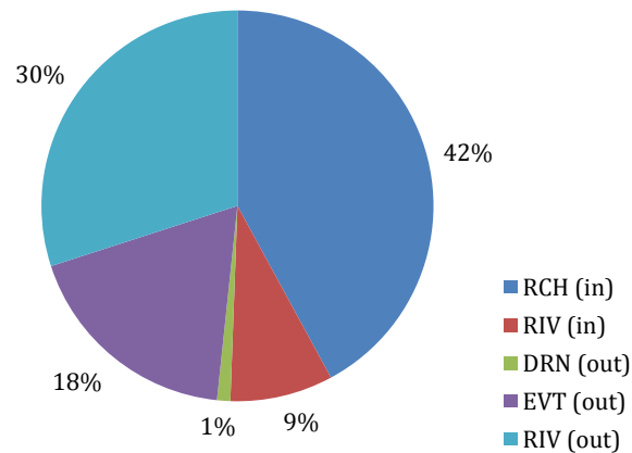
Figure C 20 Water budget overview – representation of individual boundary conditions
