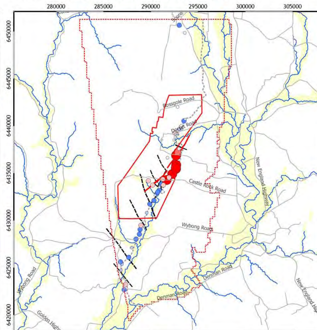
Residuals - 'starting heads' dataset - L05-11 - Permian coal seams
