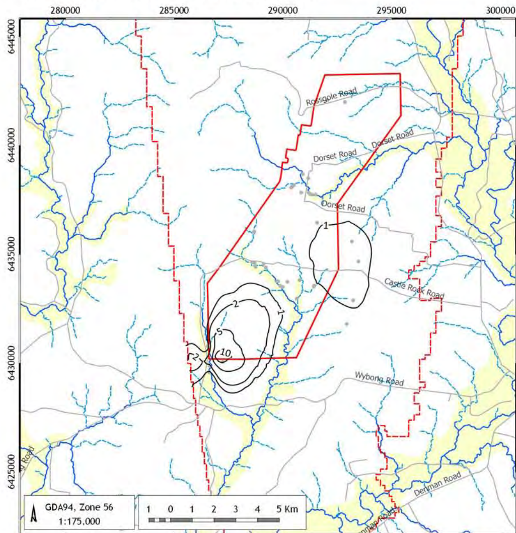
Drawdown Y30 - alluvium/weathered regolith (L02)
