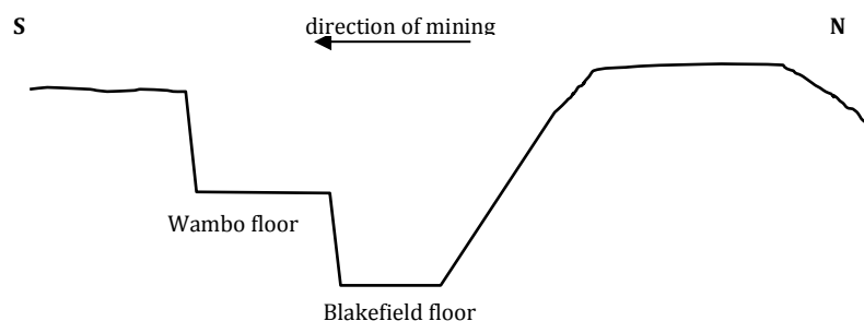
Figure C 17 Mining progression - simplified cross section
