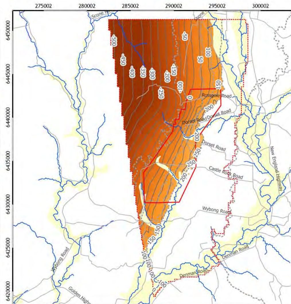
Base of Layer 9 - Blakefield
