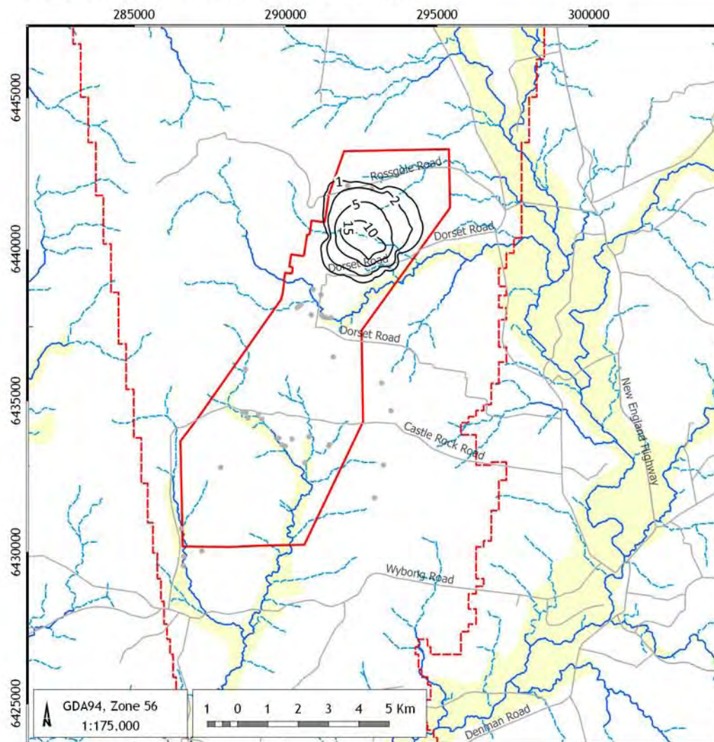
Drawdown Y03 - alluvium/weathered regolith (L02)
