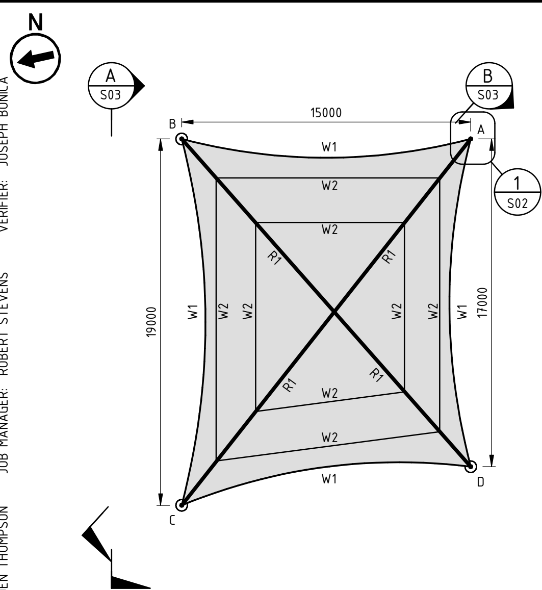
PLAN
