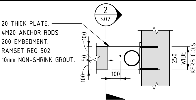
DETAIL 1 S02
