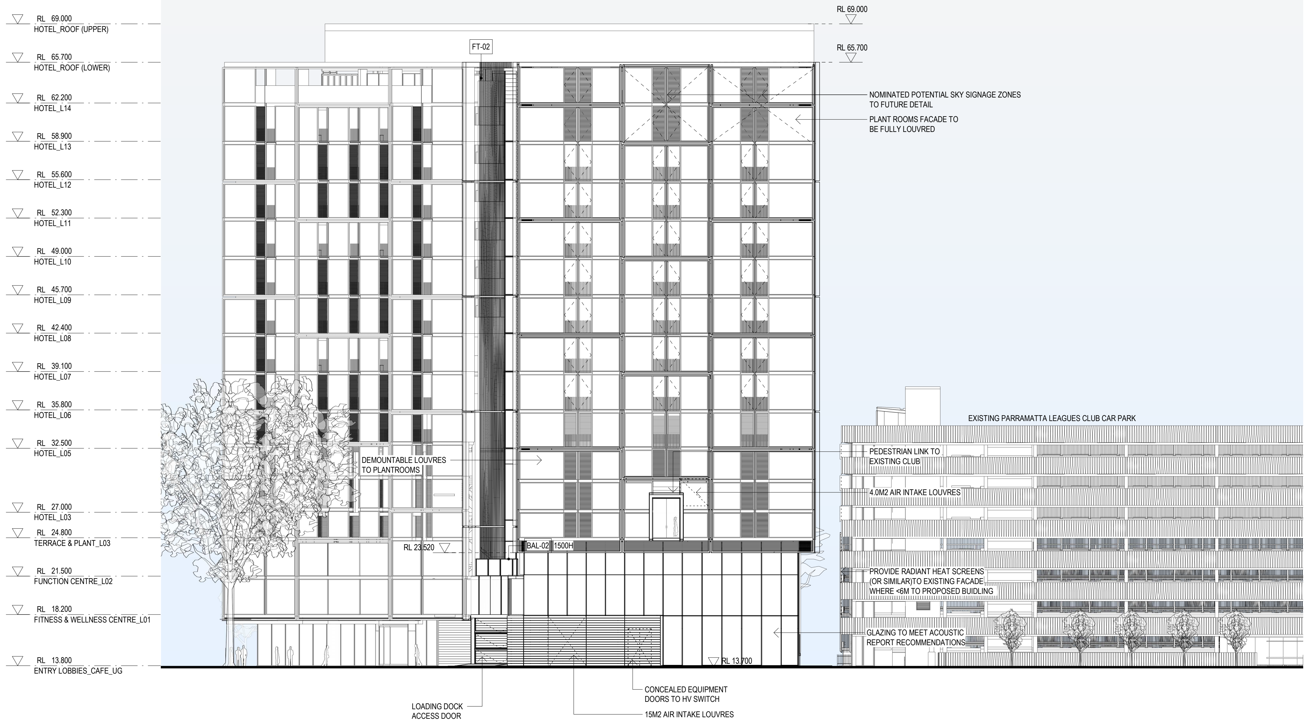
1 GA ELEVATION - NORTH-EAST (EAST) DA_1101 1:200
