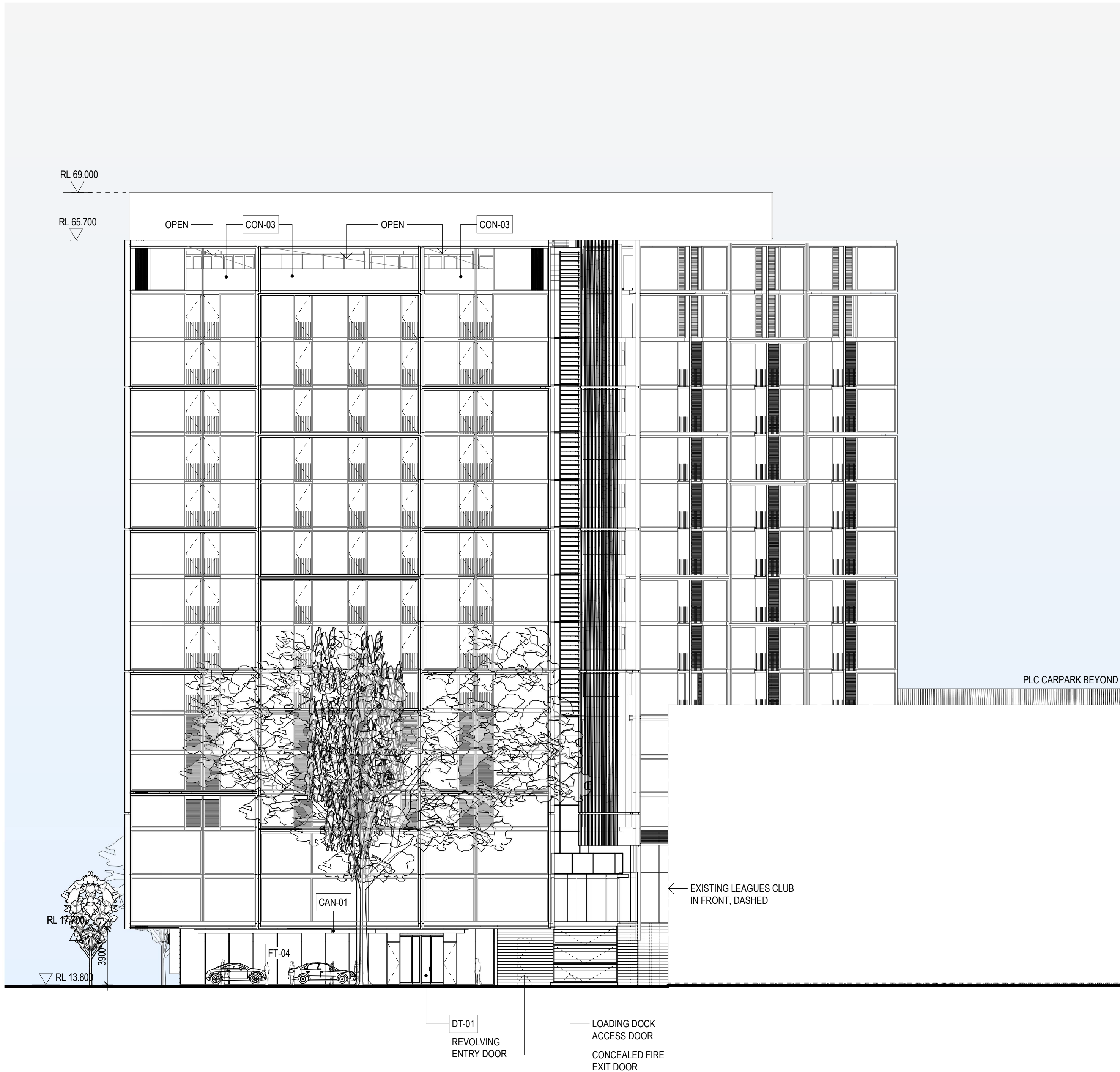
1 GA ELEVATION - SOUTH-EAST (SOUTH) DA_1101 / 1:200
