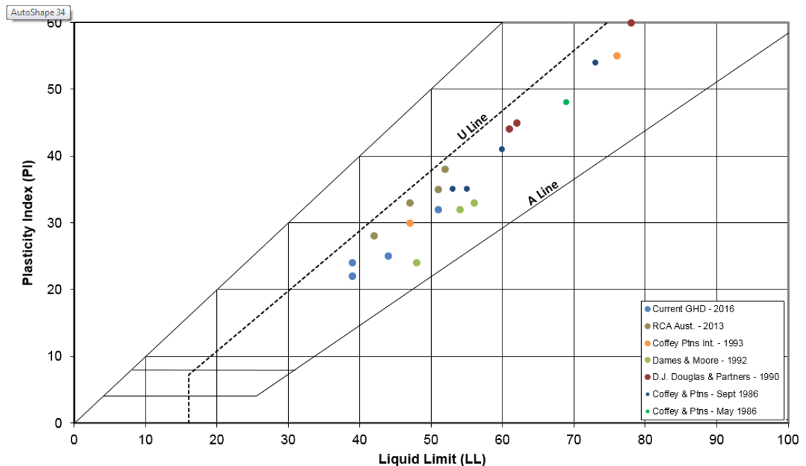
Figure 5-1 Plasticity Chart
