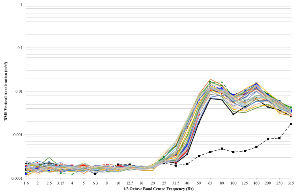
Figure 8: Measured train vibration levels, lower basement – 39 Martin Place
