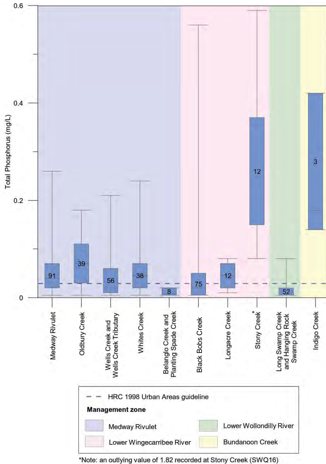
Figure 3.10 Baseline concentrations of Total Phosphorous
