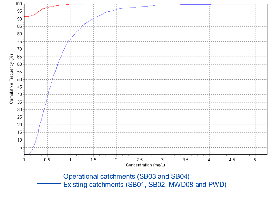
Figure 5.4 Total Phosphorus cumulative frequency graph for SB03 and SB04 discharge assessment
