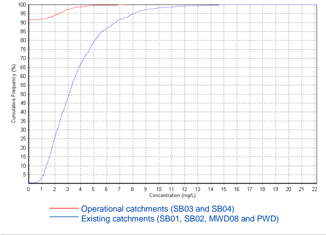
Figure 5.5 Total Nitrogen cumulative frequency graph for SB03 and SB04 discharge assessment
