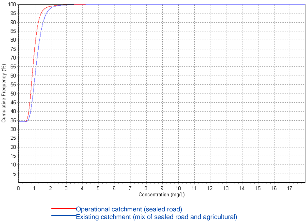
Figure 5.11 Total Nitrogen cumulative frequency graph for sealed road southern catchment
