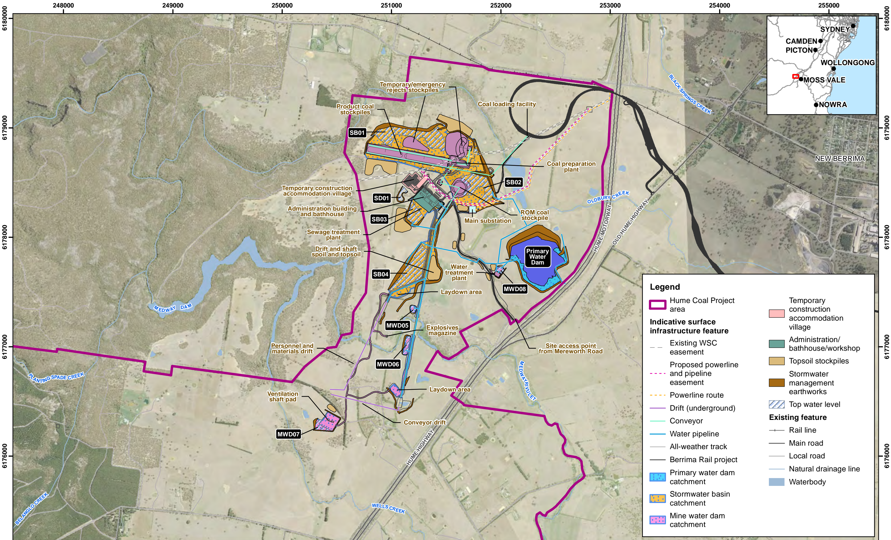
Hume Coal Surface Water Quality Assessment Figure 1.3 Surface infrastructure layout
