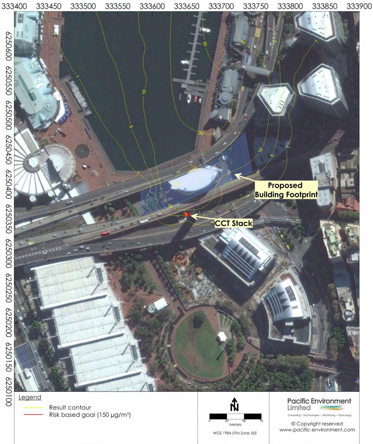
60 m – Low Emissions Scenario – 1-Hour NO 2 Concentration (Goal – 150 µg/m 3 )
