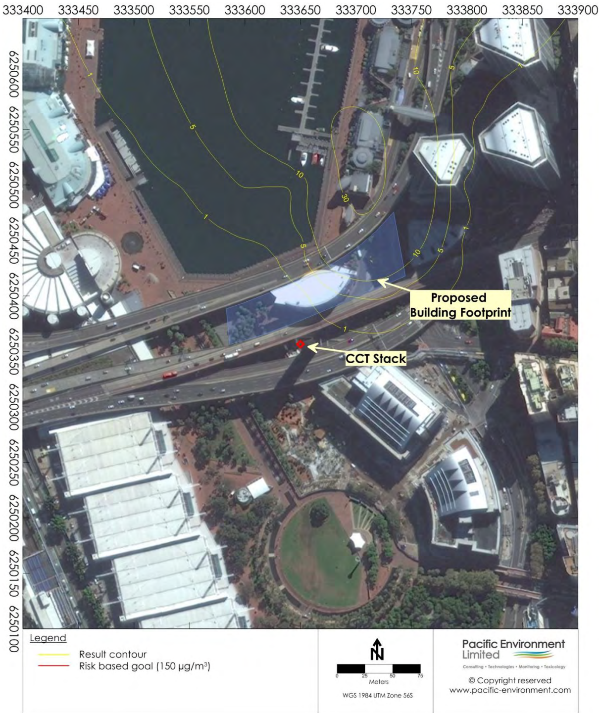
30 m – Medium Emissions Scenario – 1-Hour NO 2 Concentration (Goal – 150 µg/m³)
