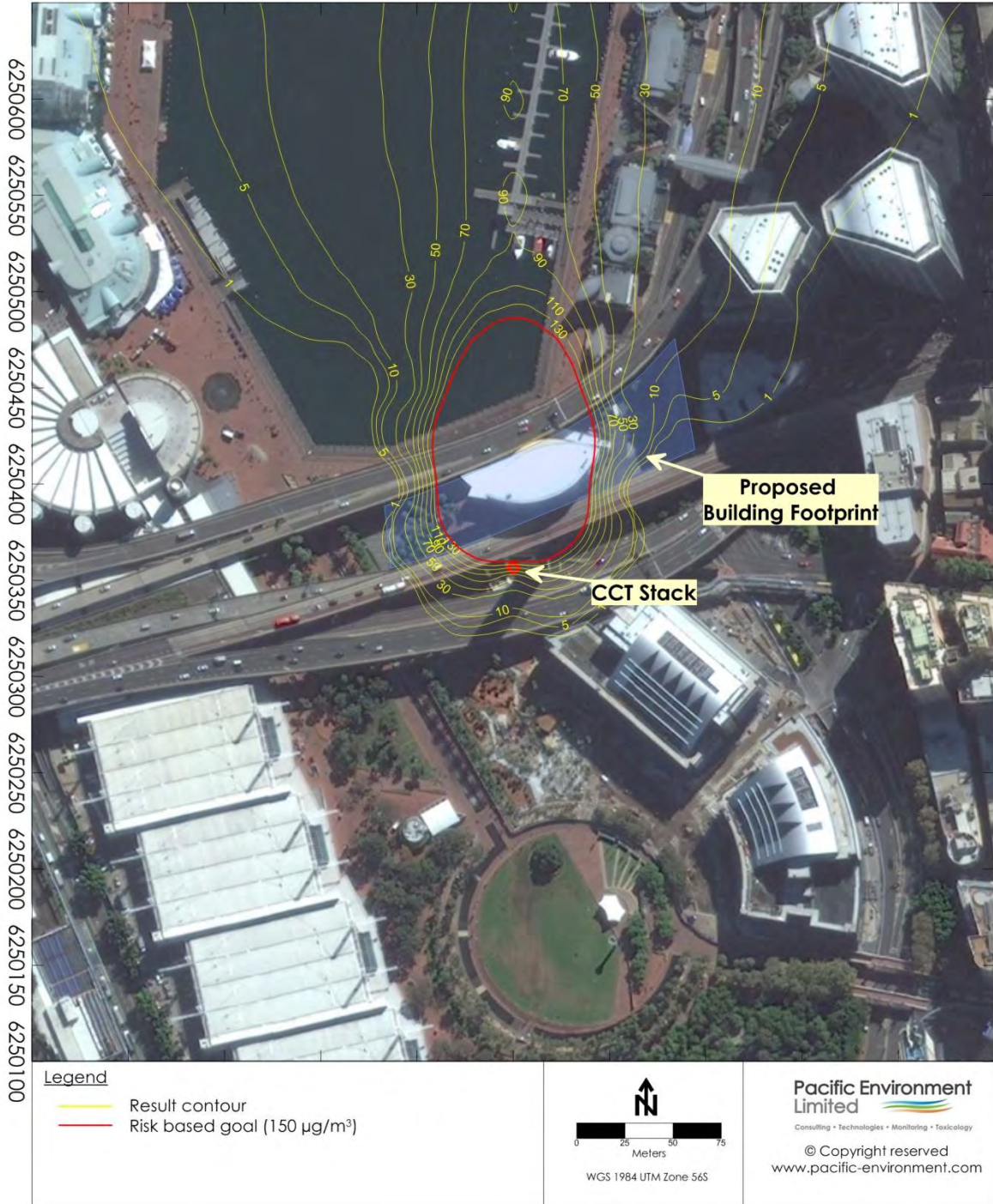
90 m – Peak Emissions Scenario – 1-Hour NO 2 Concentration (Goal – 150 µg/m³)
